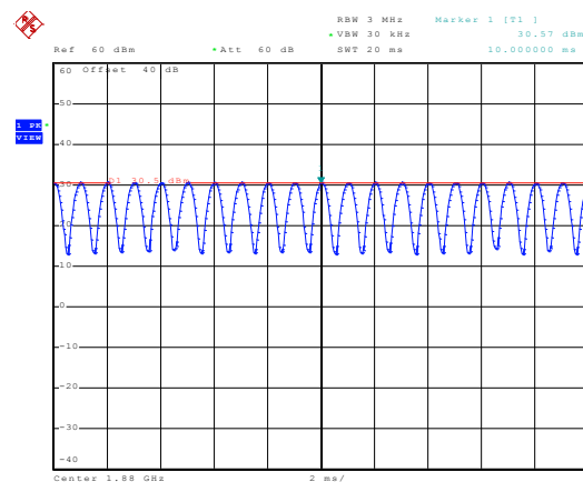
1880MHz - 80% AM
