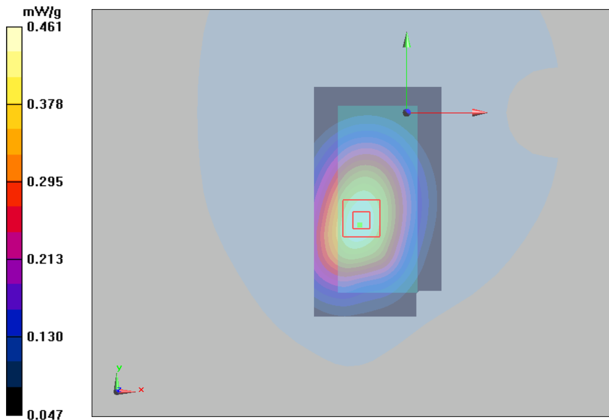
Figure 25 Body, Towards Phantom, GSM 850 GPRS (4TXslots) Channel 251
