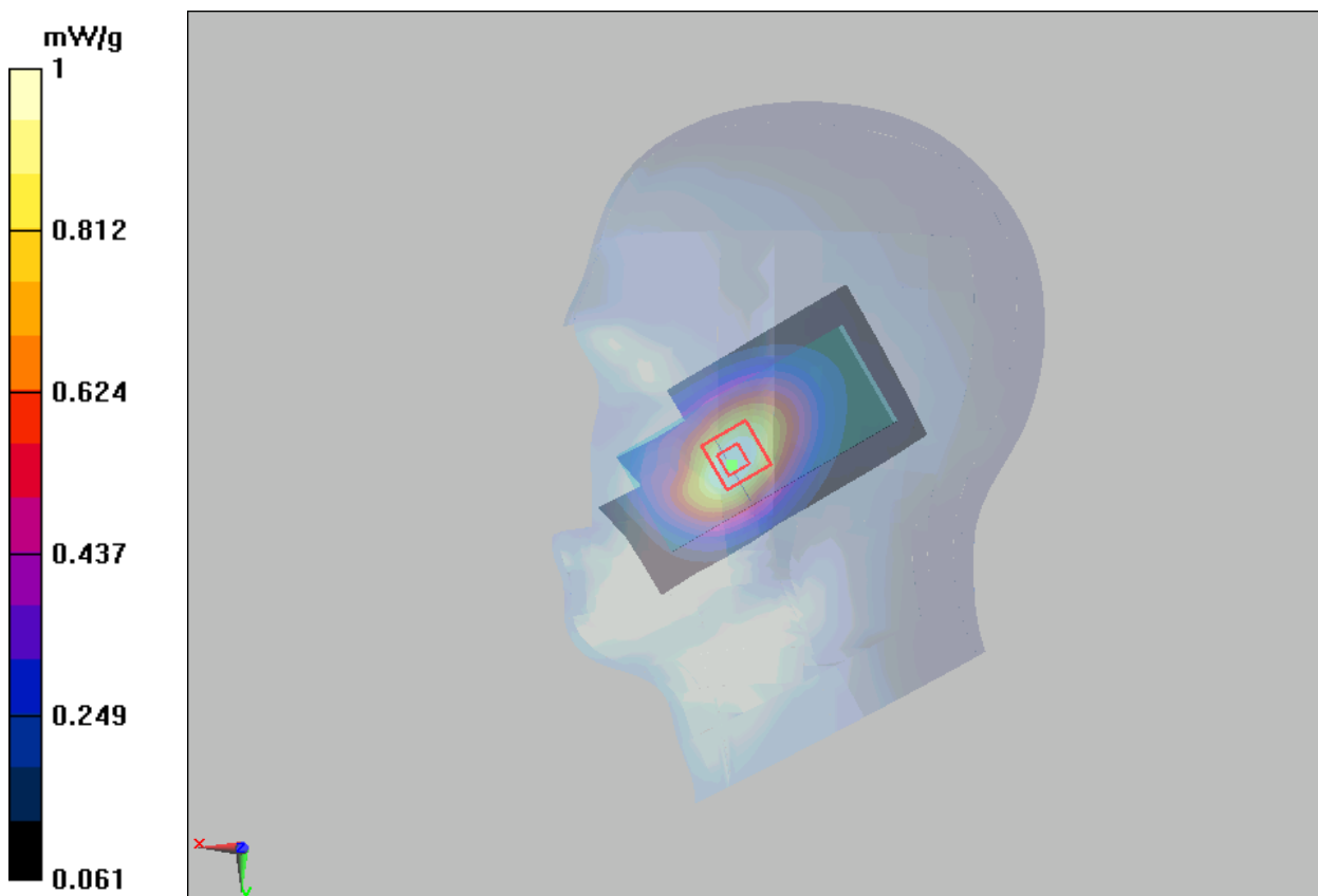
Figure 61 Right Hand Touch Cheek WCDMA Band V Channel 4183
