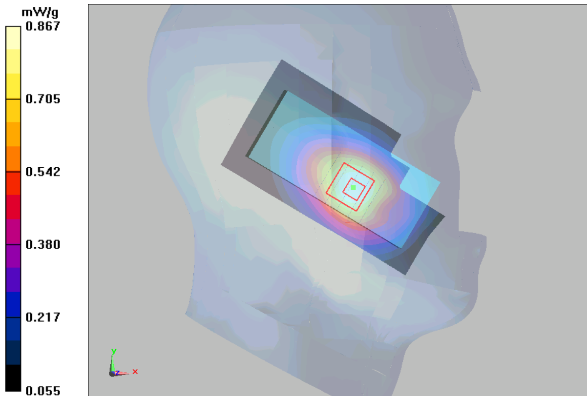
Figure 14 Left Hand Touch Cheek GSM 850 Channel 190
