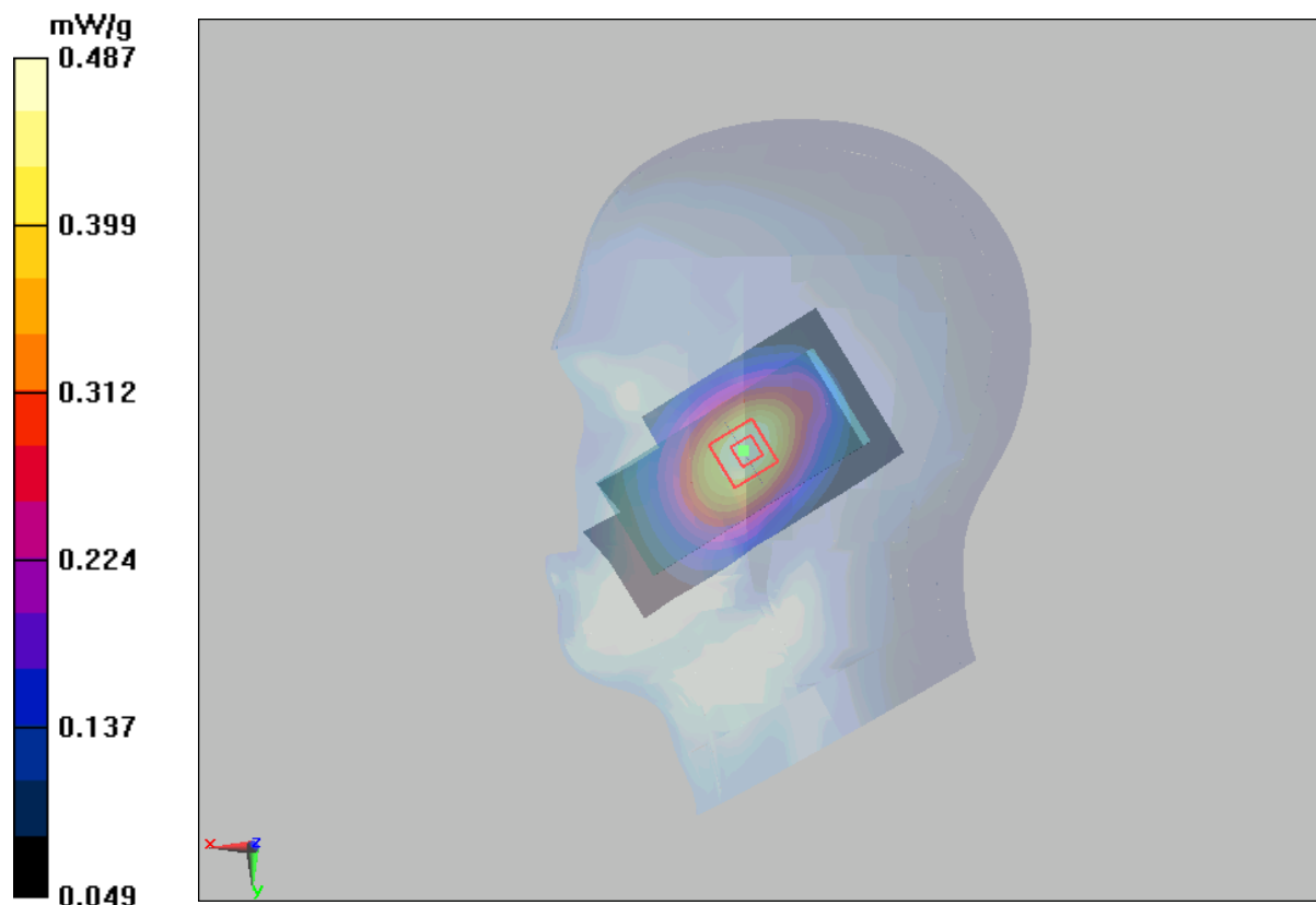
Figure 63 Right Hand Tilt 15° WCDMA Band V Channel 4183
