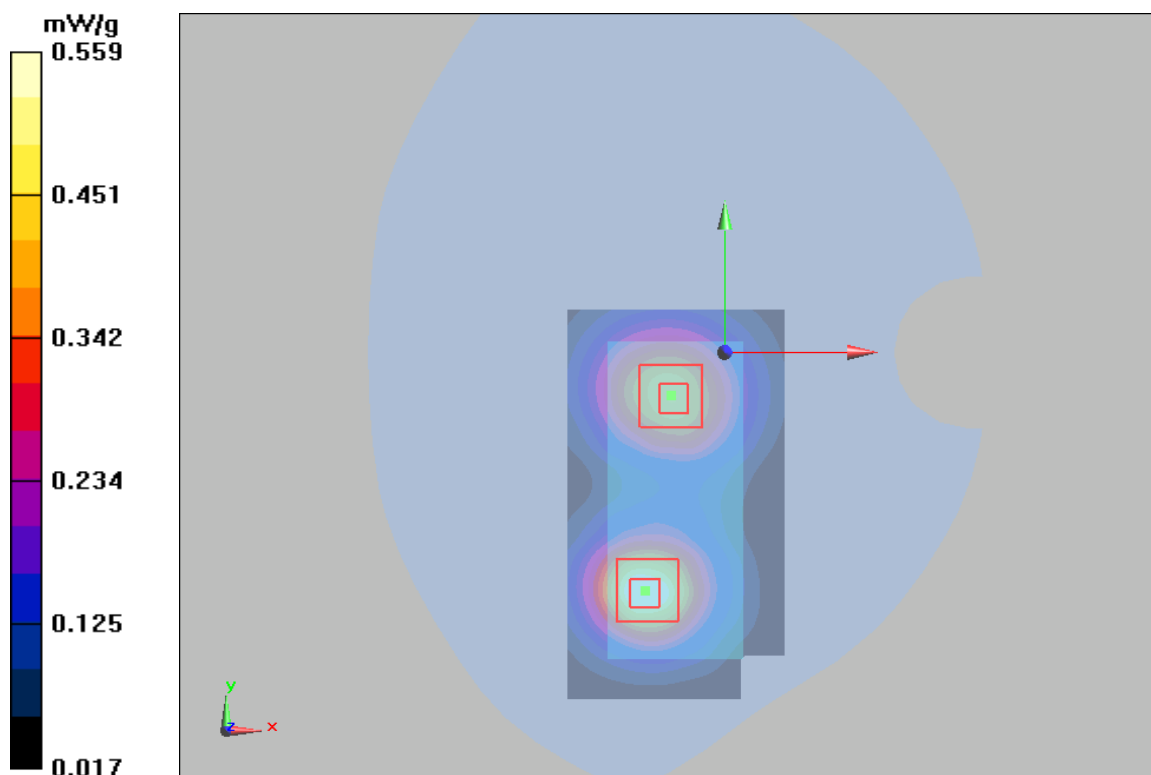
Figure 52 Body, Towards Ground, WCDMA Band IV Channel 1413
