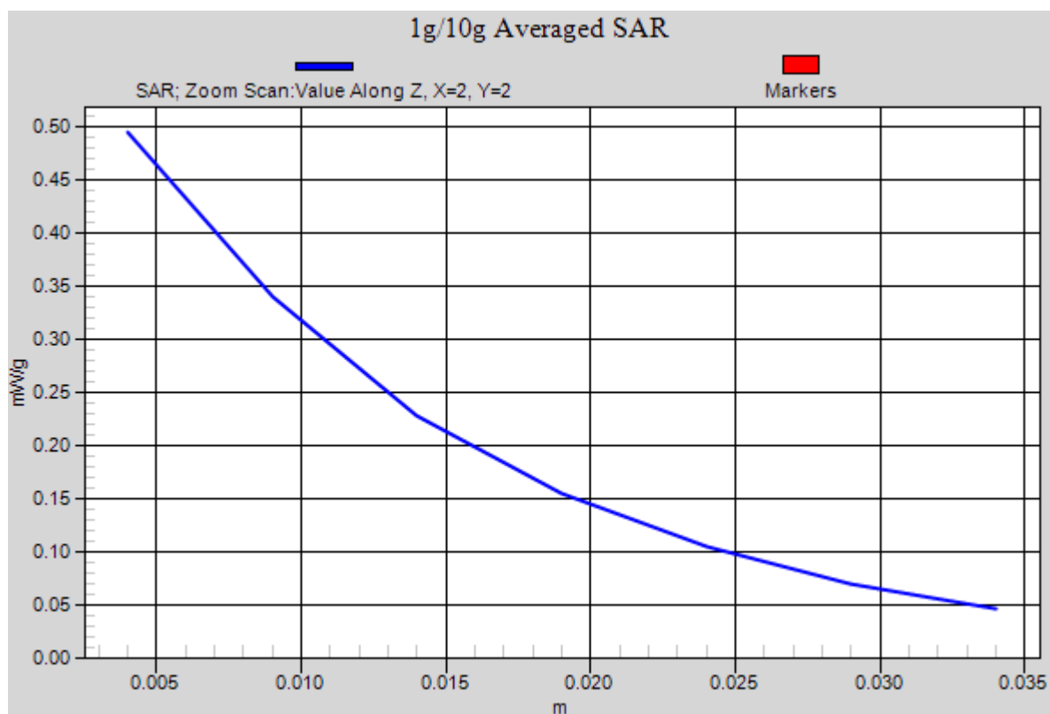
Figure 34 Right Hand Touch Cheek GSM 1900 Channel 512
