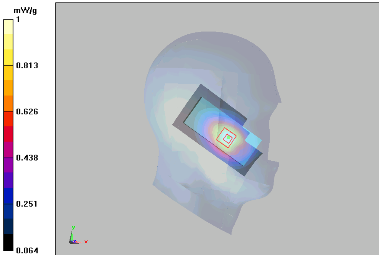
Figure 57 Left Hand Touch Cheek WCDMA Band V Channel 4183
