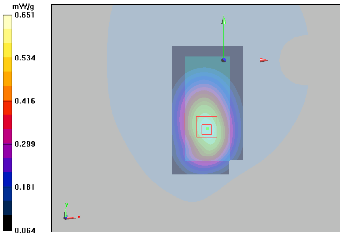
Figure 67 Body, Towards Phantom, WCDMA Band V Channel 4132
