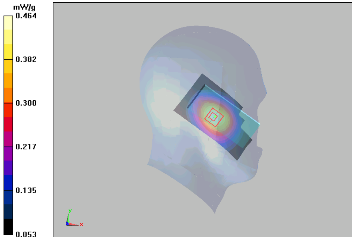
Figure 59 Left Hand Tilt 15° WCDMA Band V Channel 4183
