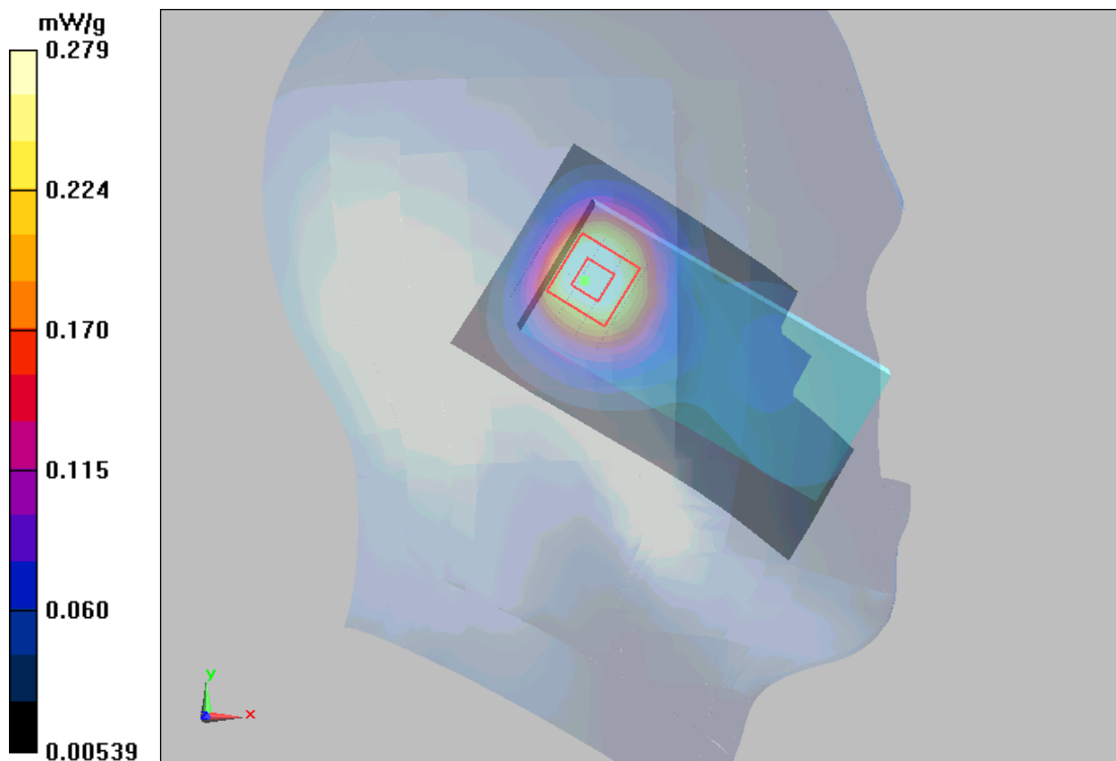
Figure 31 Left Hand Tilt 15° GSM 1900 Channel 661
