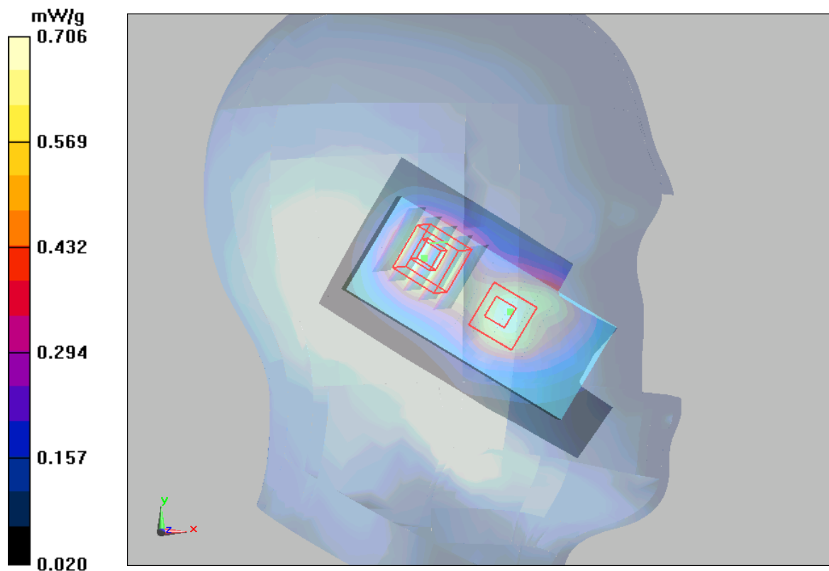
Figure 45 Left Hand Touch Cheek WCDMA Band IV Channel 1413
