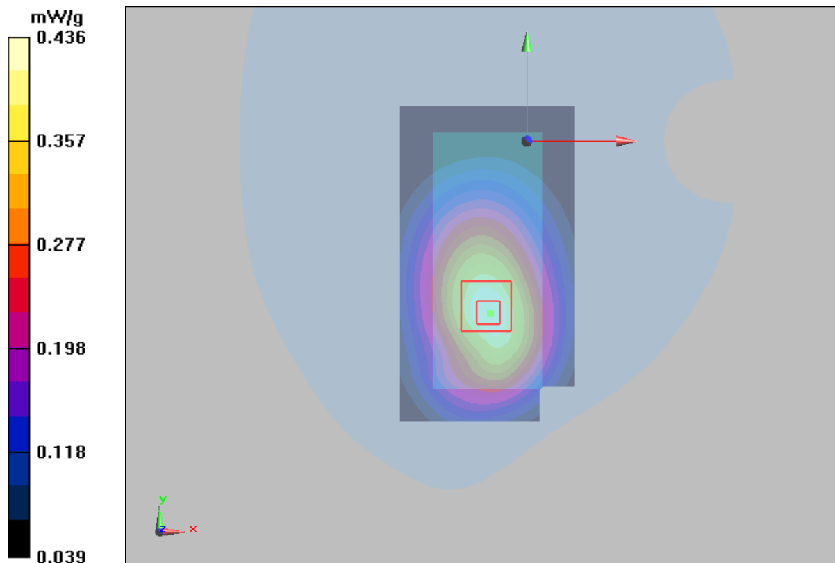
Figure 28 Body with Earphone, Towards Phantom, GSM 850 Channel 190
