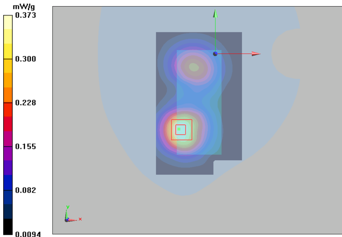
Figure 38 Body, Towards Ground, GSM 1900 GPRS (2TXslots) Channel 661
