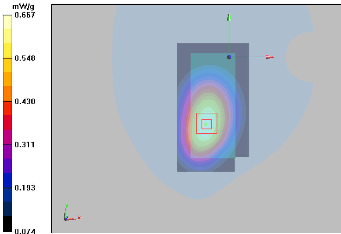
Figure 64 Body, Towards Ground, WCDMA Band V Channel 4183
