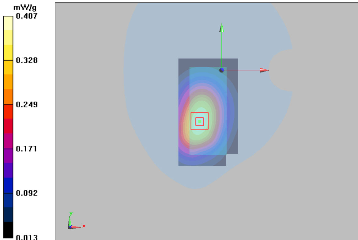
Figure 21 Body, Towards Ground, GSM 850 Channel 190
