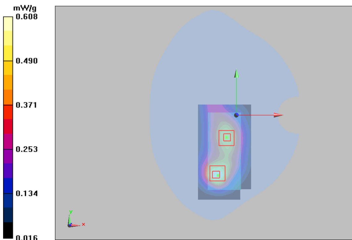
Figure 55 Body with Earphone, Towards Ground, WCDMA Band IV Channel 1513
