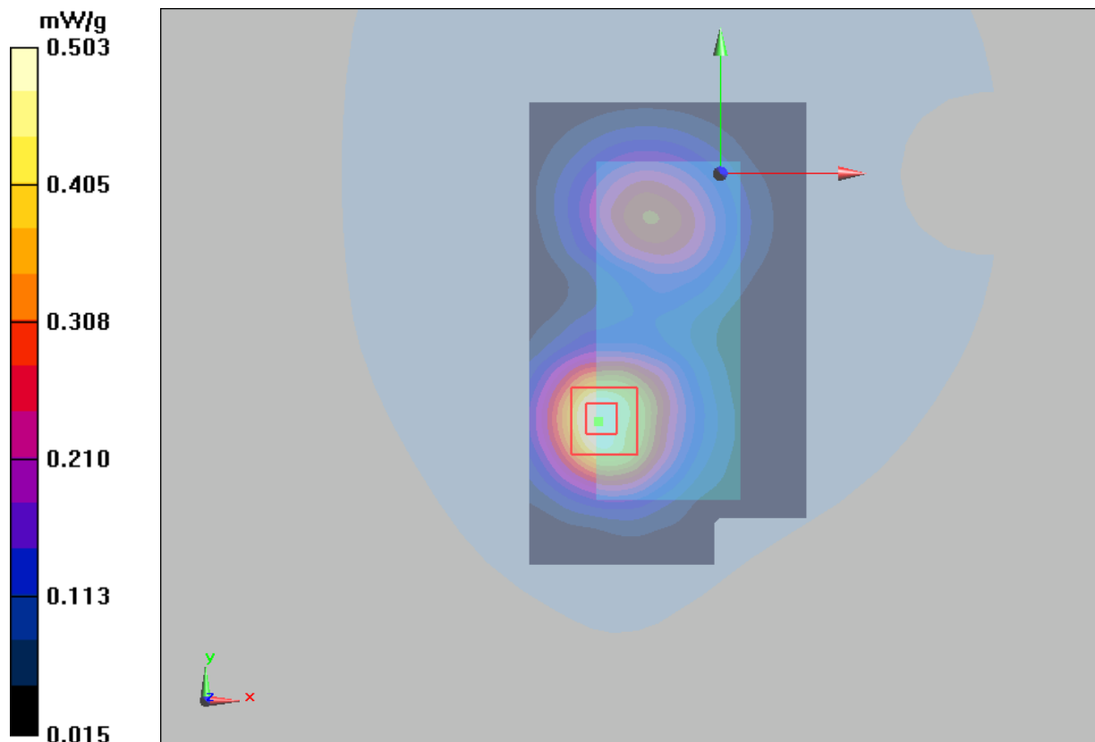
Figure 44 Body, Towards Ground, GSM 1900 EGPRS (2TXslots) Channel 512
