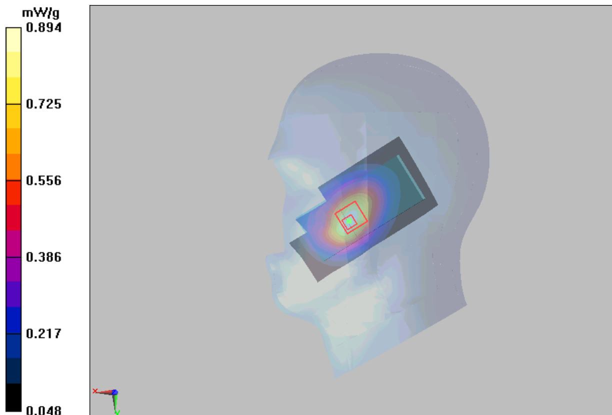
Figure 18 Right Hand Touch Cheek GSM 850 Channel 190
