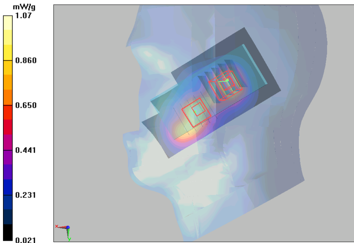
Figure 49 Right Hand Touch Cheek WCDMA Band IV Channel 1312
