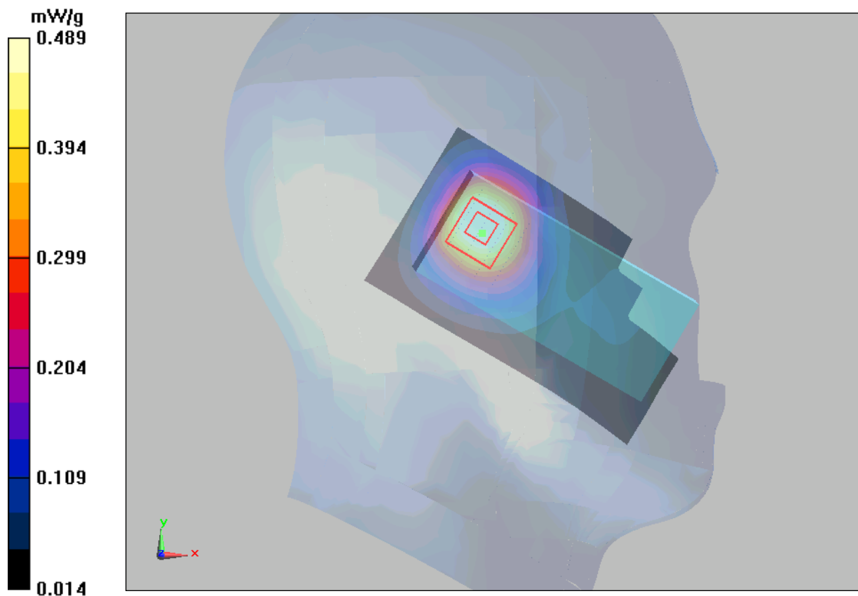
Figure 46 Left Hand Tilt 15° WCDMA Band IV Channel 1413
