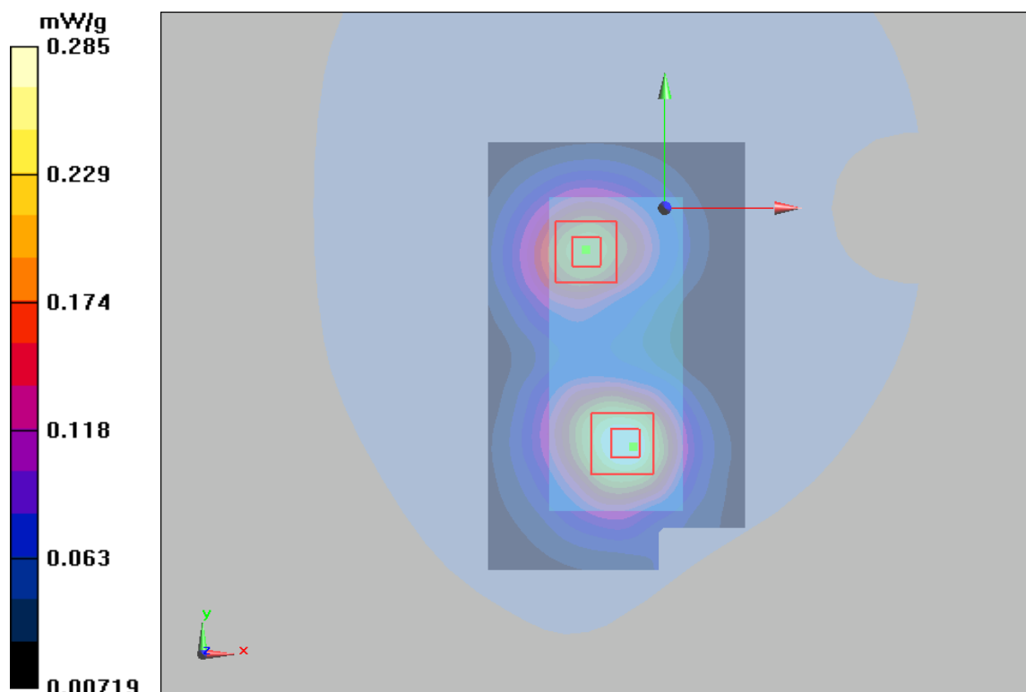
Figure 42 Body, Towards Phantom, GSM 1900 GPRS (2TXslots) Channel 661
