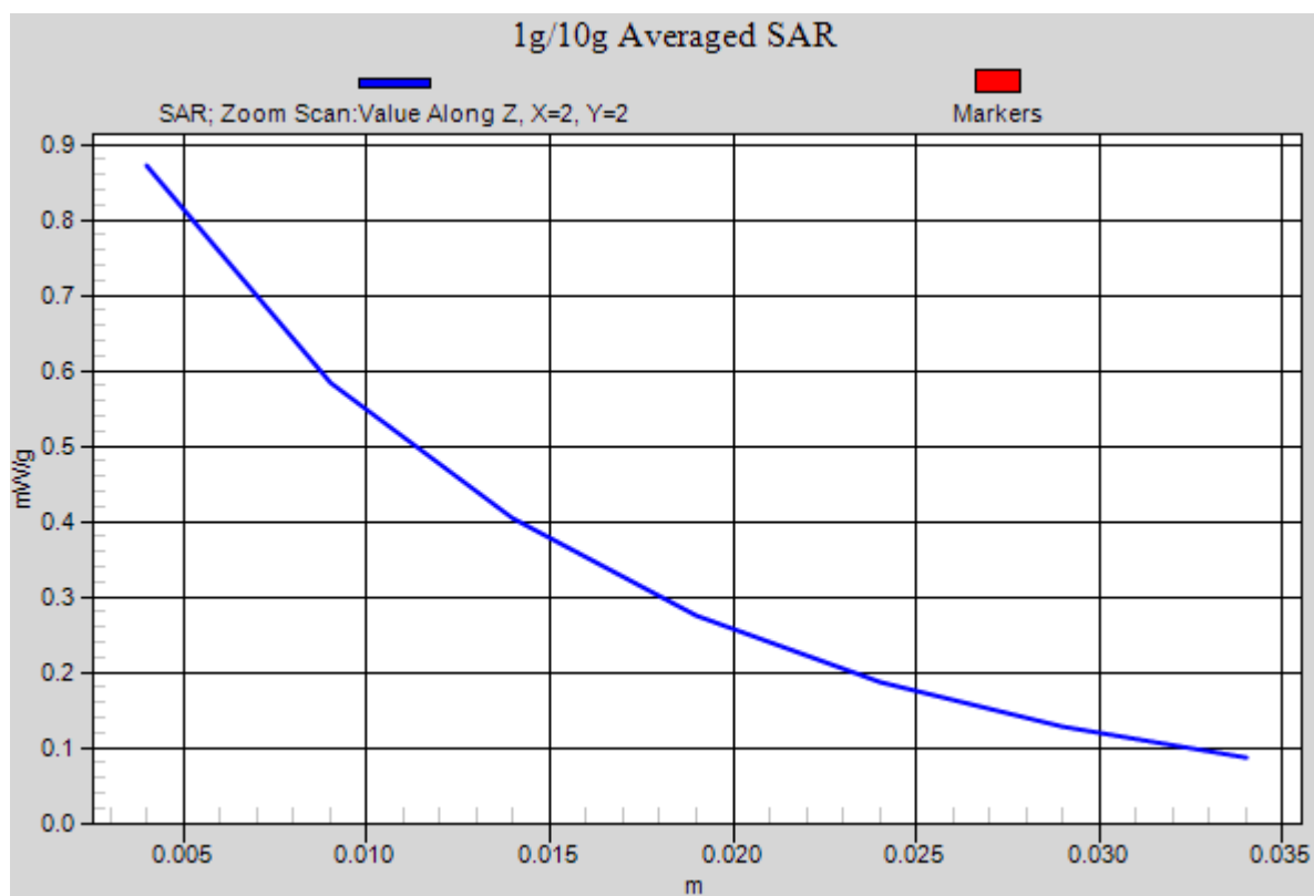
Figure 51 Body, Towards Ground, WCDMA Band IV Channel 1513
