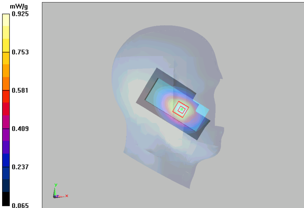
Figure 58 Left Hand Touch Cheek WCDMA Band V Channel 4132
