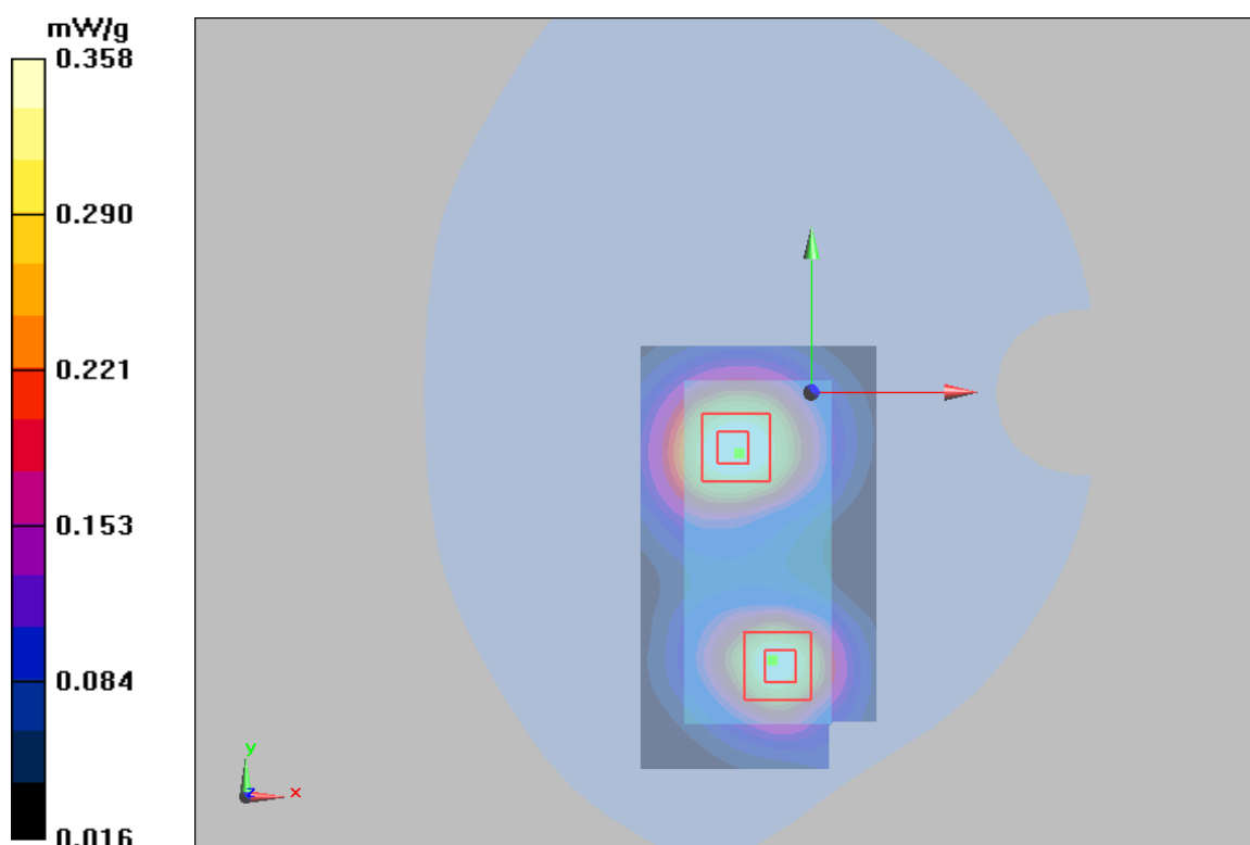
Figure 54 Body, Towards Phantom, WCDMA Band IV Channel 1413
