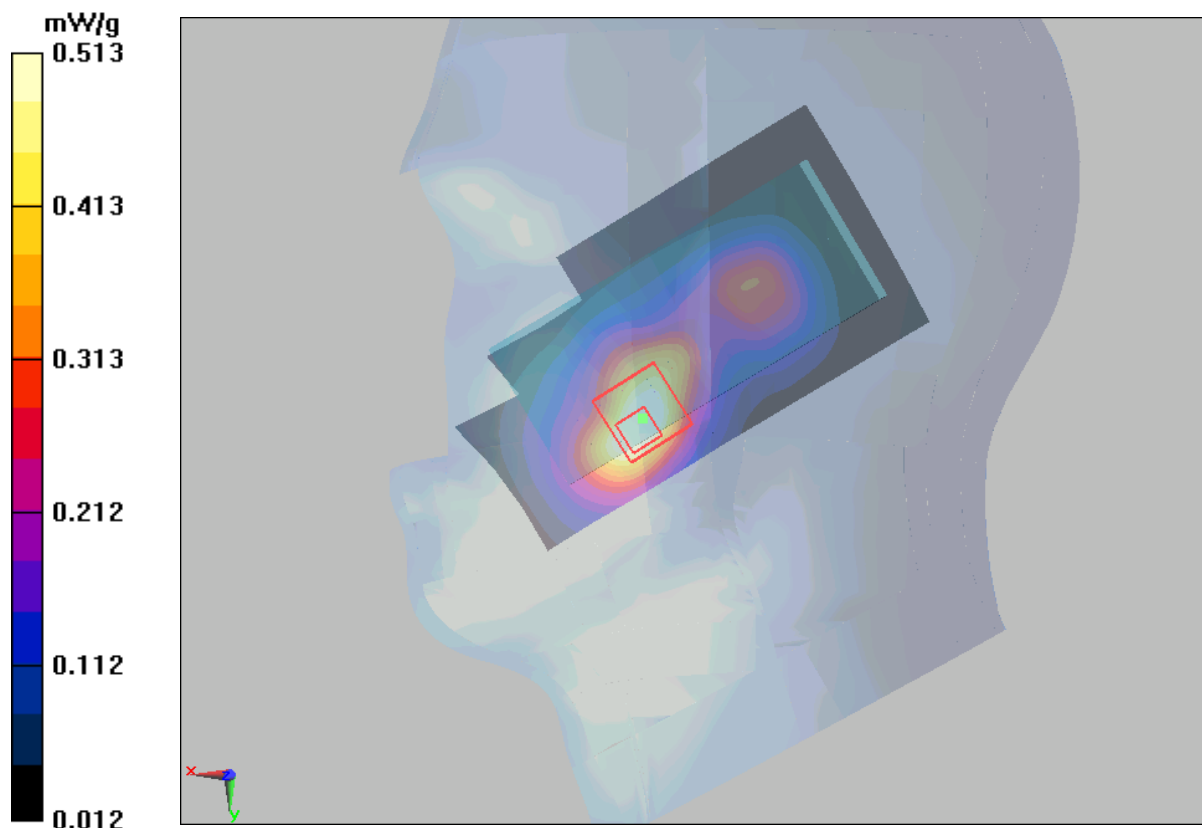
Figure 32 Right Hand Touch Cheek GSM 1900 Channel 810
