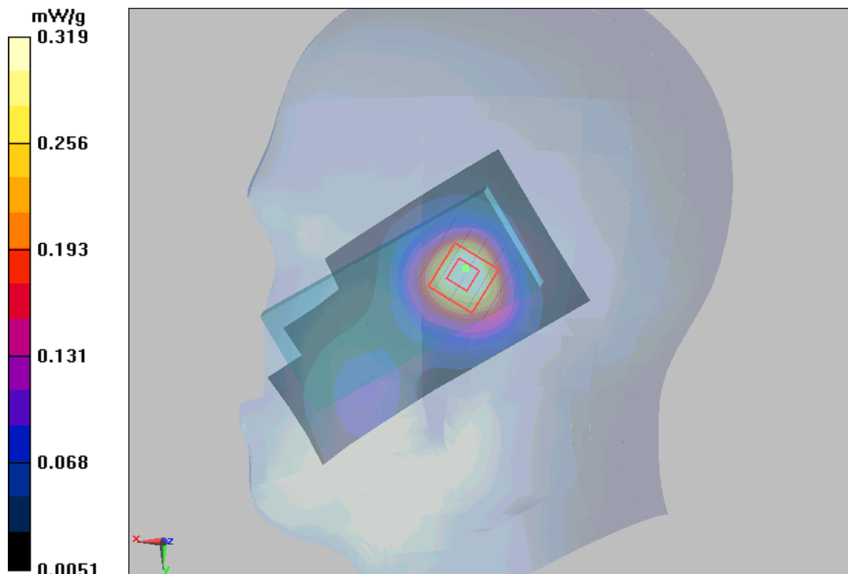
Figure 35 Right Hand Tilt 15° GSM 1900 Channel 661
