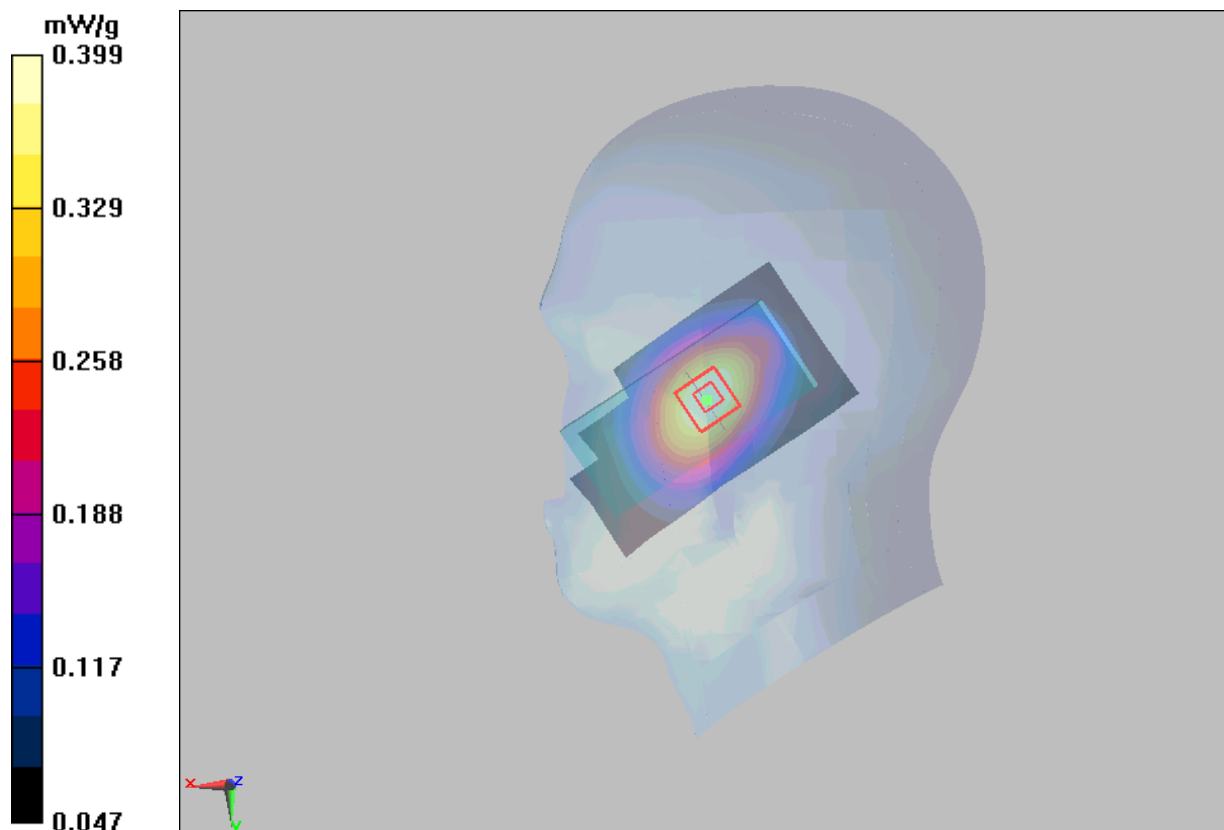
Figure 20 Right Hand Tilt 15° GSM 850 Channel 190
