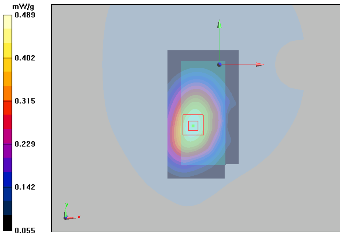
Figure 23 Body, Towards Ground, GSM 850 GPRS (3TXslots) Channel 190
