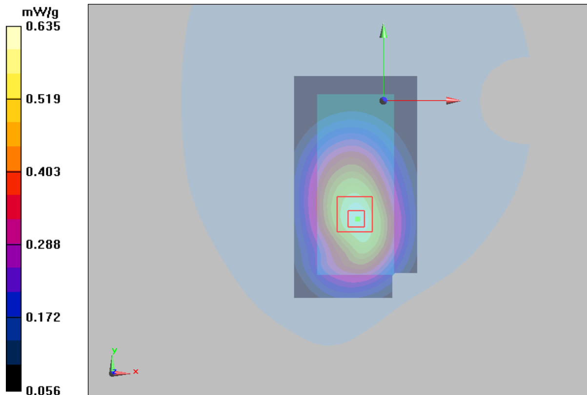
Figure 65 Body, Towards Phantom, WCDMA Band V Channel 4233
