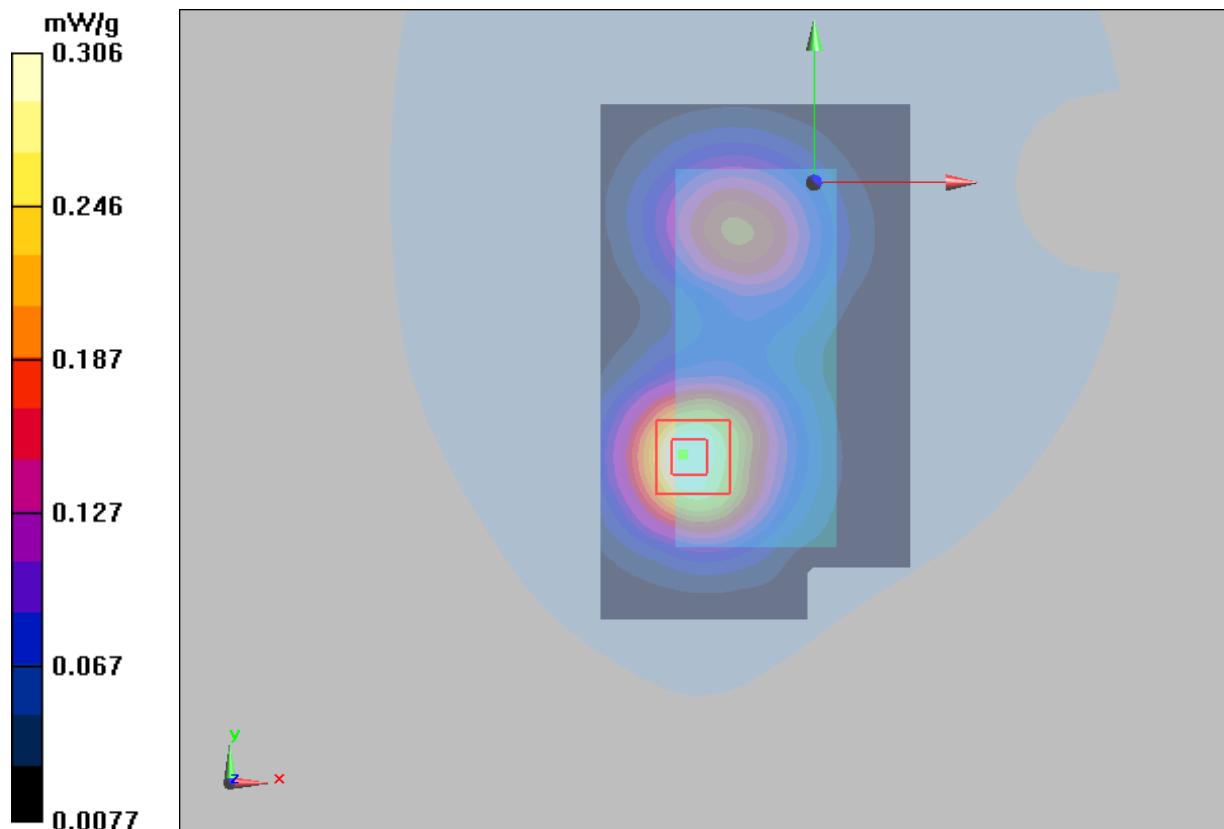
Figure 36 Body, Towards Ground, GSM 1900 Channel 661
