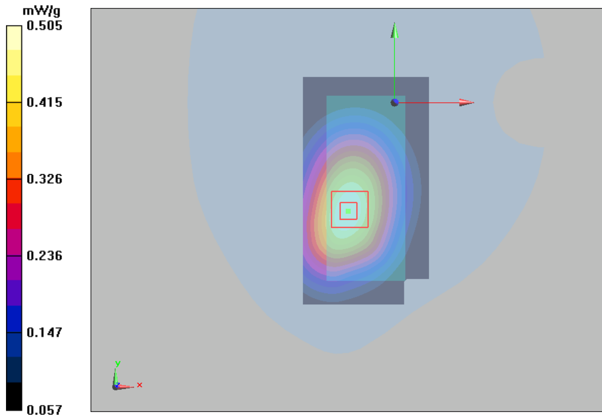
Figure 22 Body, Towards Ground, GSM 850 GPRS (2TXslots) Channel 190
