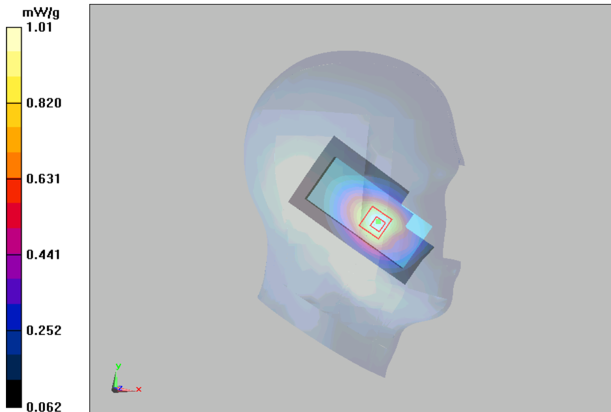
Figure 56 Left Hand Touch Cheek WCDMA Band V Channel 4233
