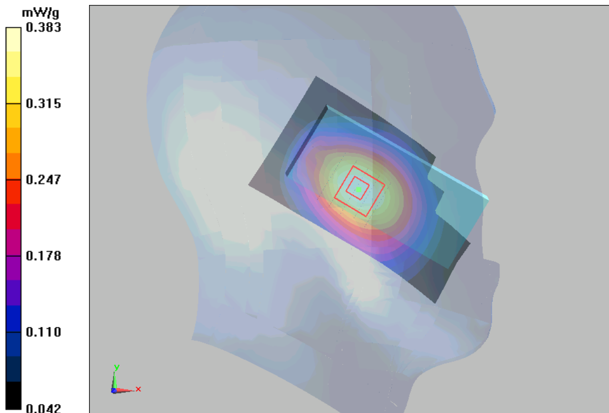
Figure 16 Left Hand Tilt 15° GSM 850 Channel 190
