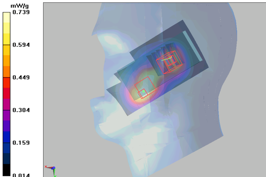
Figure 48 Right Hand Touch Cheek WCDMA Band IV Channel 1413
