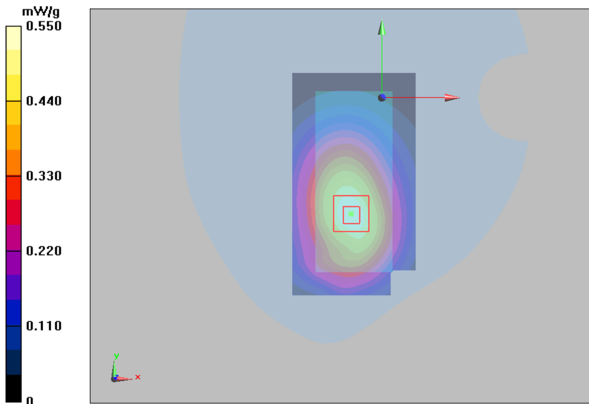
Figure 26 Body, Towards Phantom, GSM 850 GPRS (4TXslots) Channel 190
