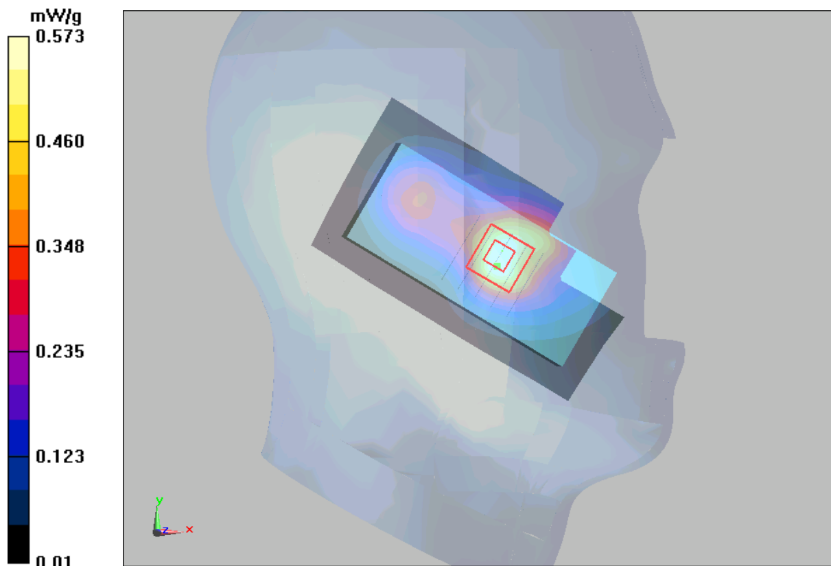
Figure 30 Left Hand Touch Cheek GSM 1900 Channel 661
