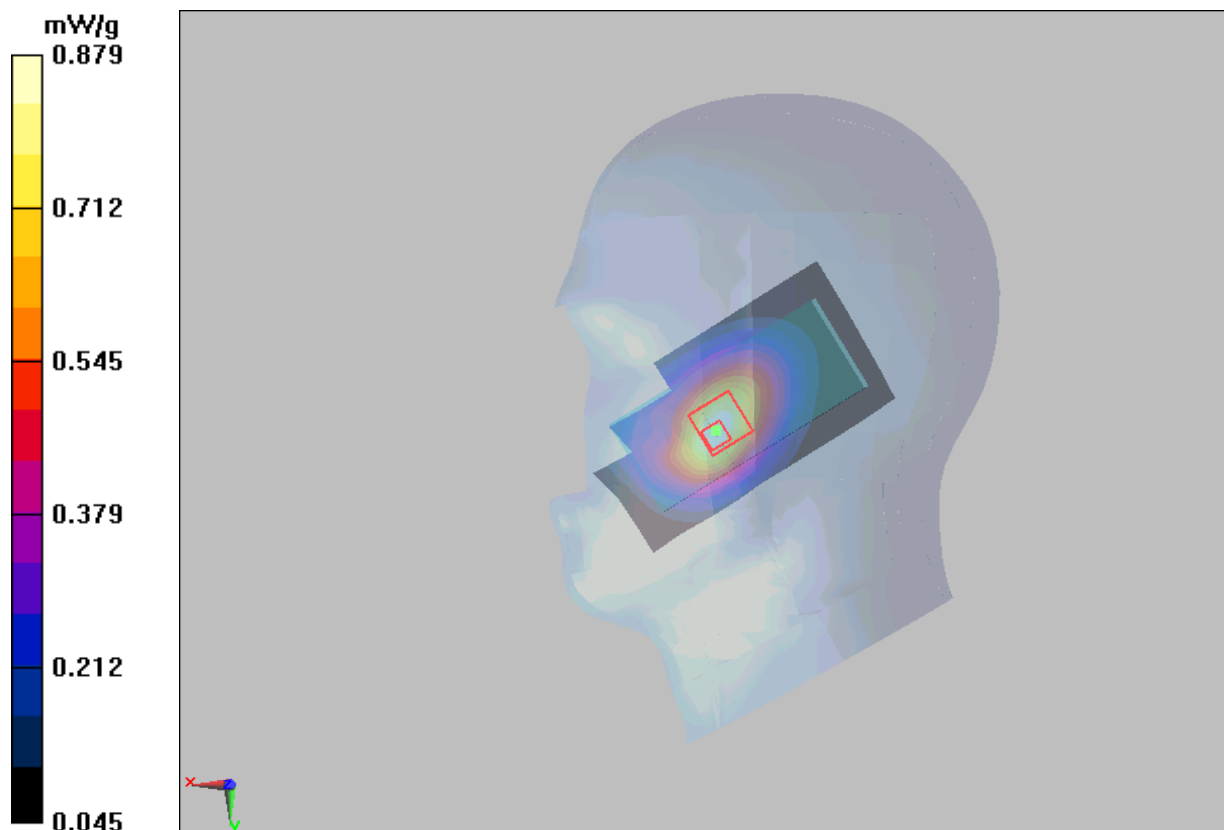
Figure 17 Right Hand Touch Cheek GSM 850 Channel 251
