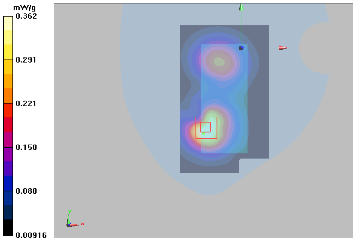
Figure 40 Body, Towards Ground, GSM 1900 GPRS (3TXslots) Channel 661
