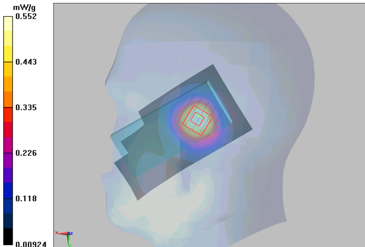
Figure 50 Right Hand Tilt 15° WCDMA Band IV Channel 1413
