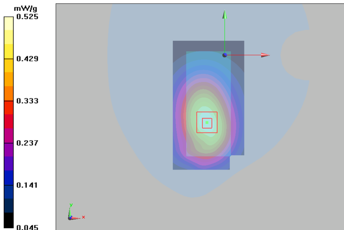
Figure 27 Body, Towards Phantom, GSM 850 GPRS (4TXslots) Channel 128
