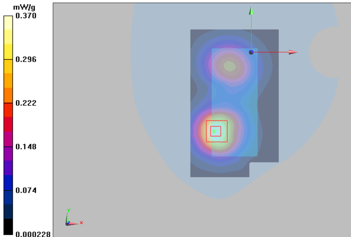
Figure 41 Body, Towards Ground, GSM 1900 GPRS (4TXslots) Channel 661
