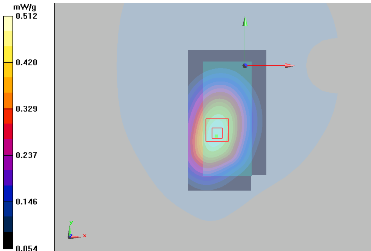
Figure 24 Body, Towards Ground, GSM 850 GPRS (4TXslots) Channel 190
