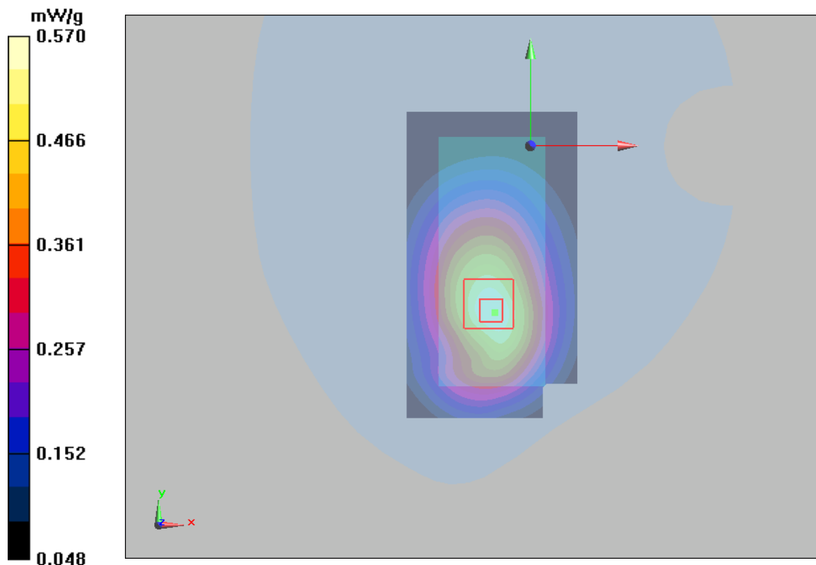
Figure 68 Body with Earphone, Towards Phantom, WCDMA Band V Channel 4183
