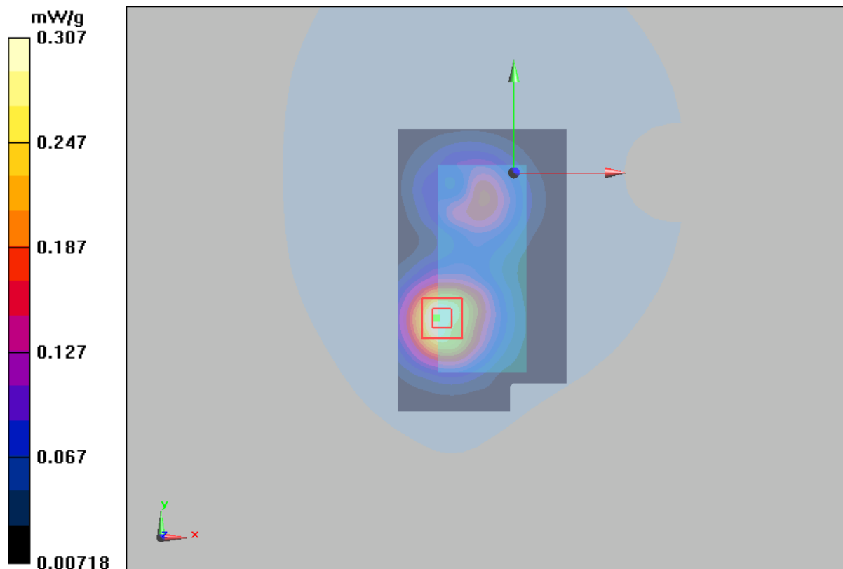
Figure 37 Body, Towards Ground, GSM 1900 GPRS (2TXslots) Channel 810
