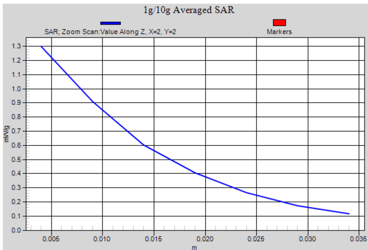
Figure 47 Right Hand Touch Cheek WCDMA Band IV Channel 1513
