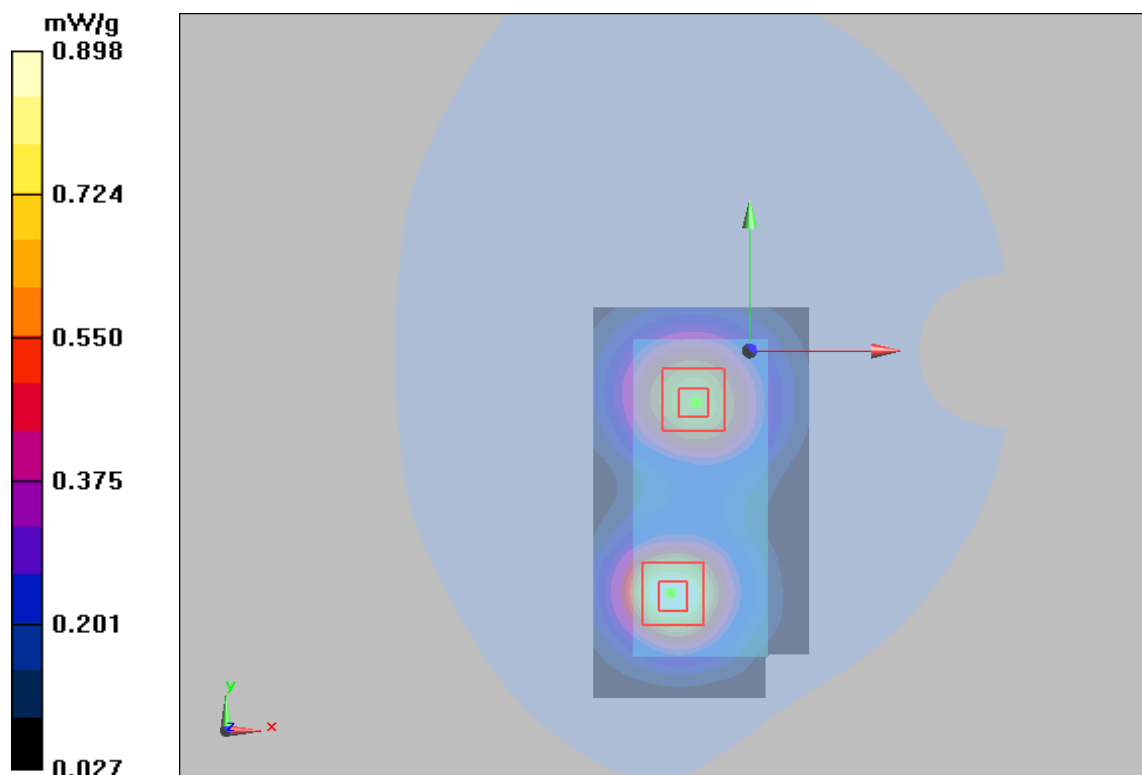
Figure 53 Body, Towards Ground, WCDMA Band IV Channel 1312
