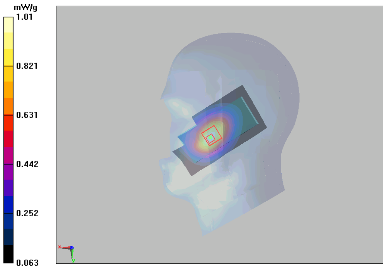
Figure 62 Right Hand Touch Cheek WCDMA Band V Channel 4132
