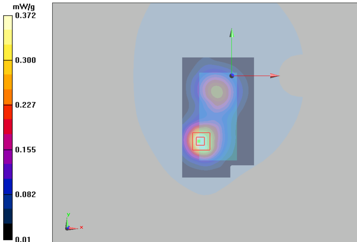
Figure 43 Body with Earphone, Towards Ground, GSM 1900 Channel 512
