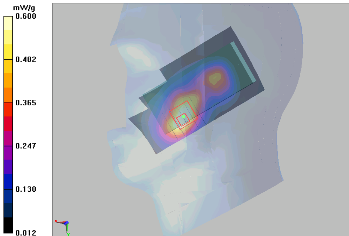
Figure 33 Right Hand Touch Cheek GSM 1900 Channel 661
