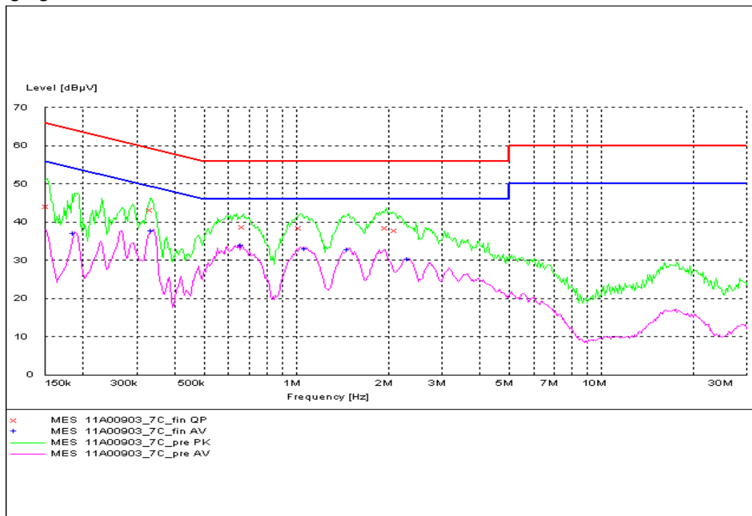
Figure A.5 Conducted Emission
