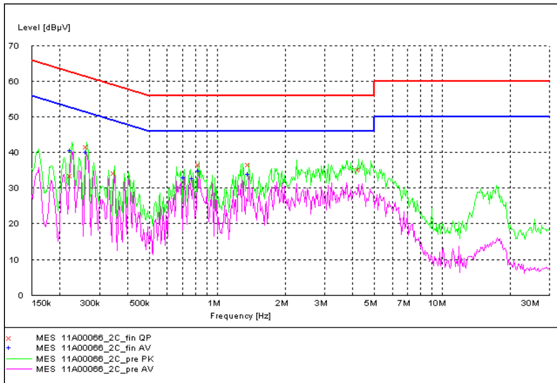
Figure A.6 Conducted Emission
