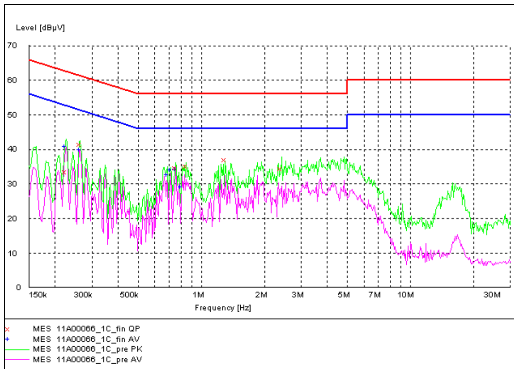
Figure A.5 Conducted Emission
