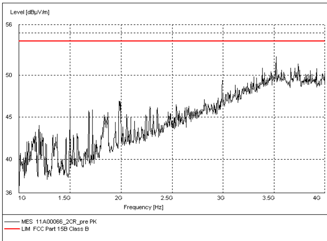
Figure A.2 Radiated Emission from 1GHz to 4GHz
