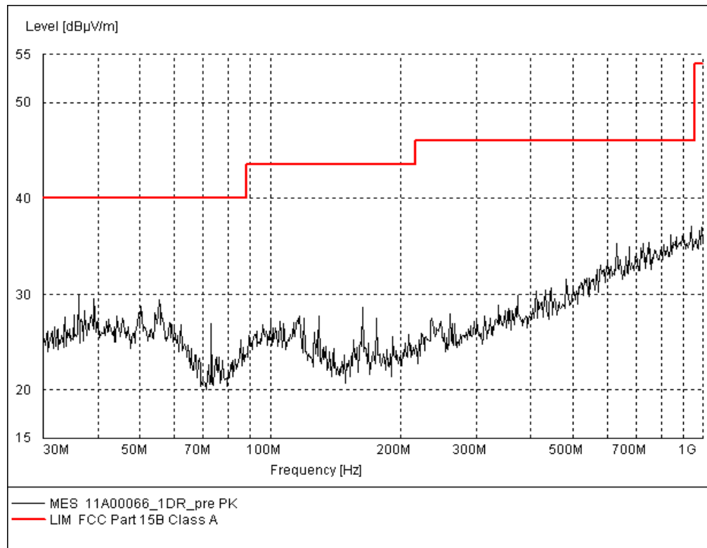
Figure A.3 Radiated Emission from 30MHz to 1GHz
