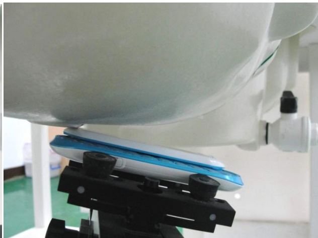
Right Tilted (DUT Slide Right)
