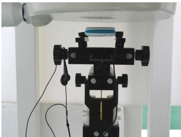
Face of the DUT with Phantom 1.5 cm Gap (DUT Slide Off)
