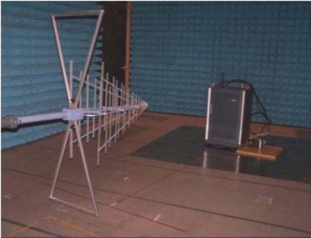
Radiated Emissions- Front View (Below 1 GHz)
