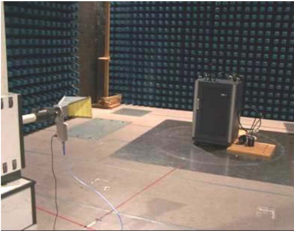
Radiated Emissions- Front View (Above 1 GHz)
