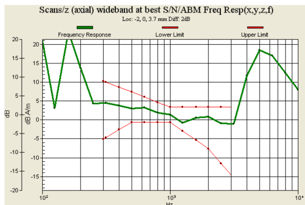
Fig. 9.6 CDMA2000 BC14 Ch1275
