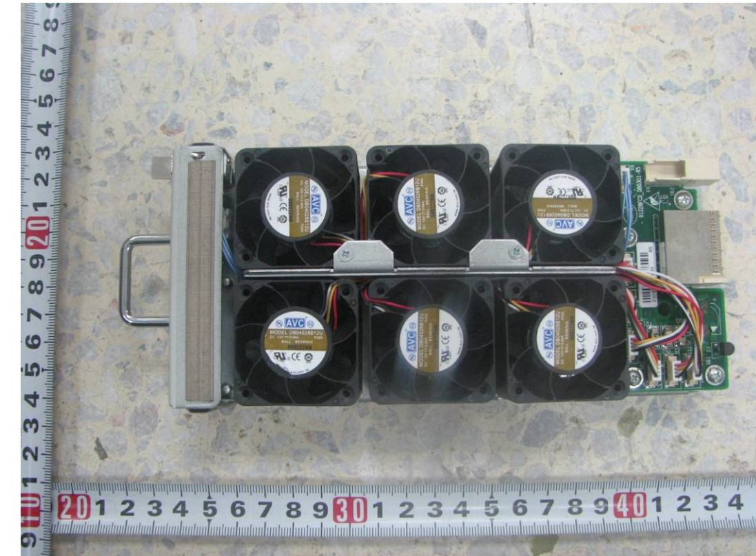
Front view of the fan module
