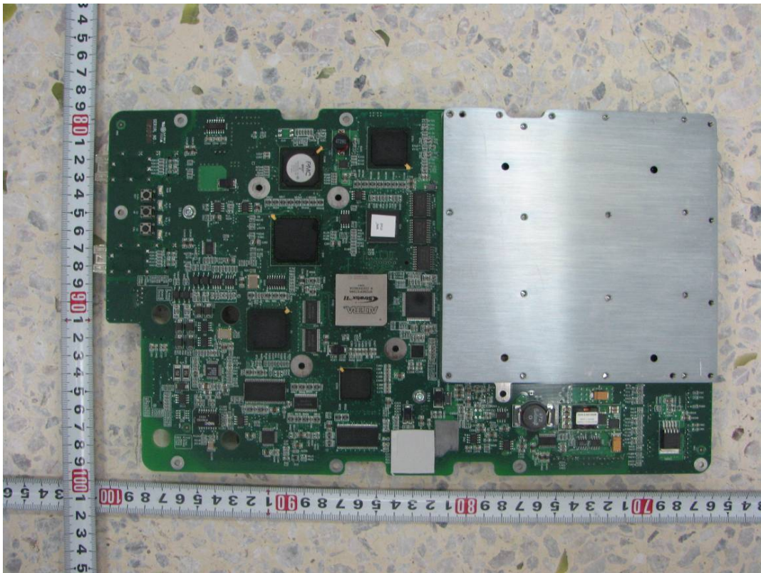
View of mainboard in RF module
