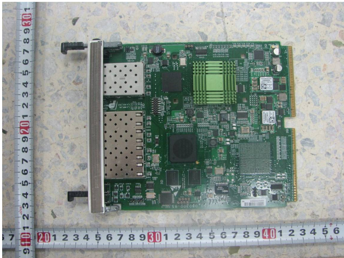
Front view of the FS board
