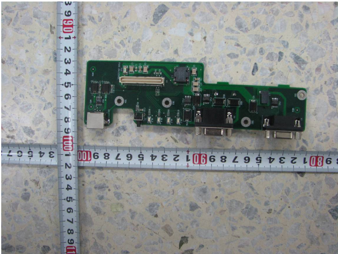
View of interface board
