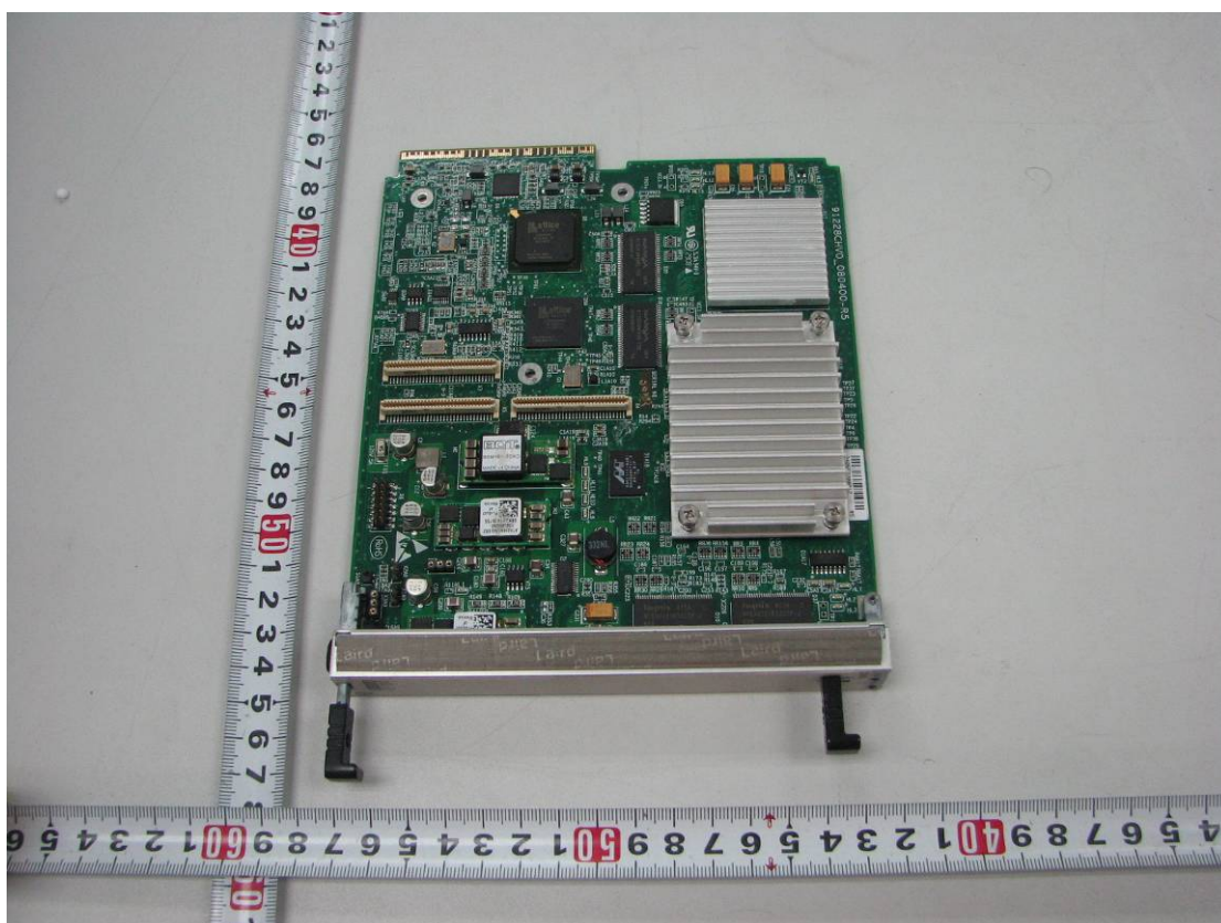
B side of CHV board
