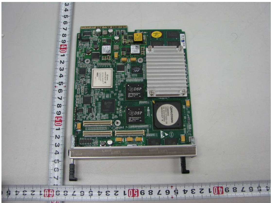
B side of CHD board
