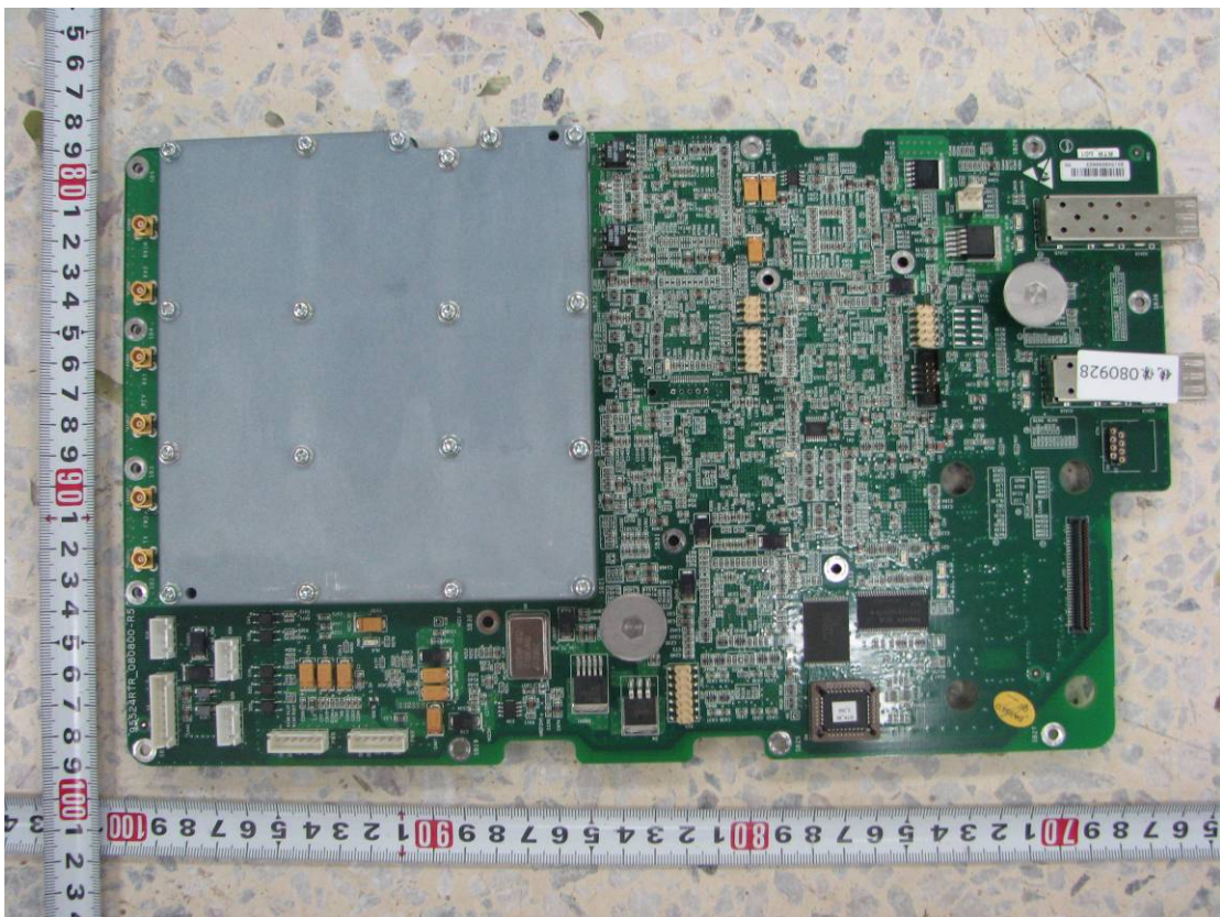
View of mainboard in RF module
