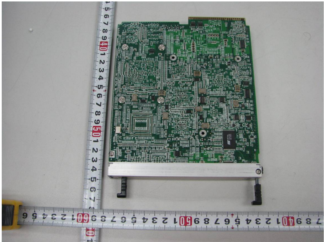
A Side of CHD board
