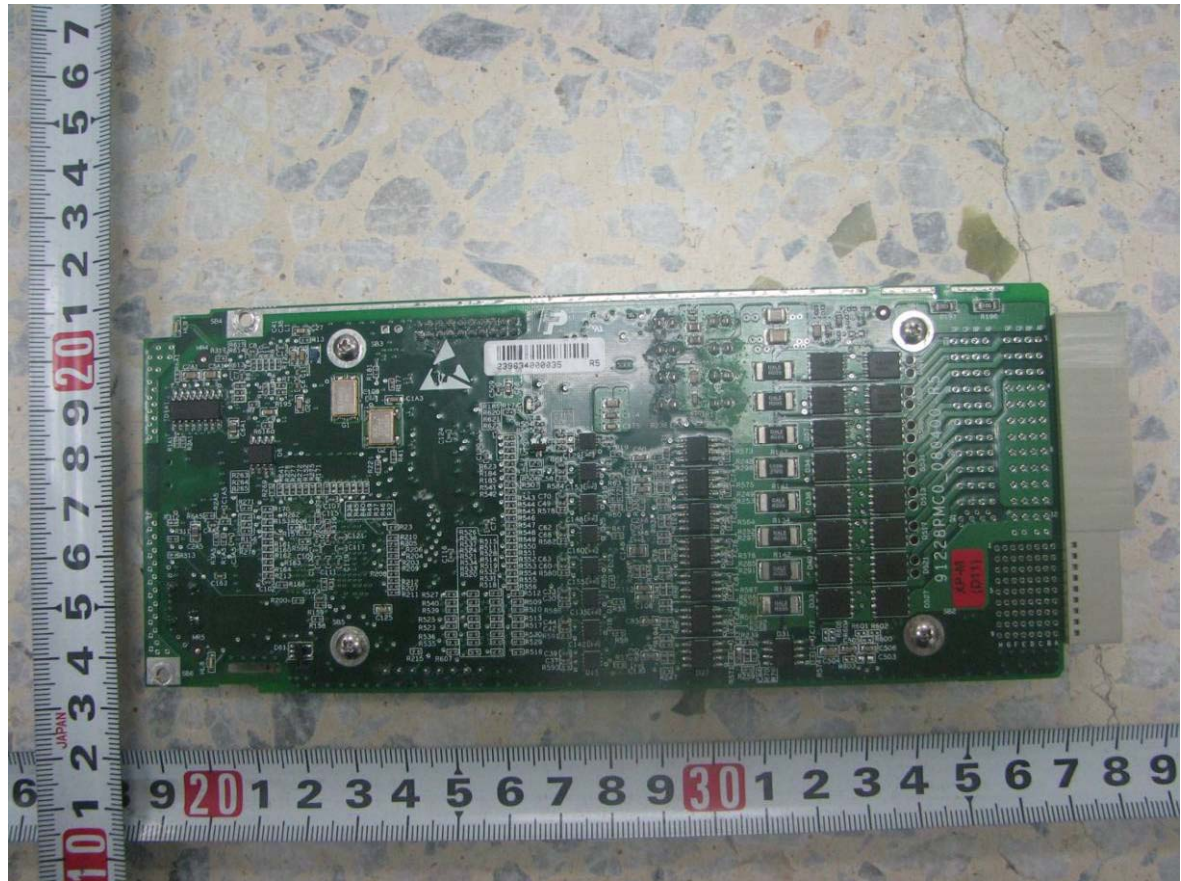
view of the power supply module
