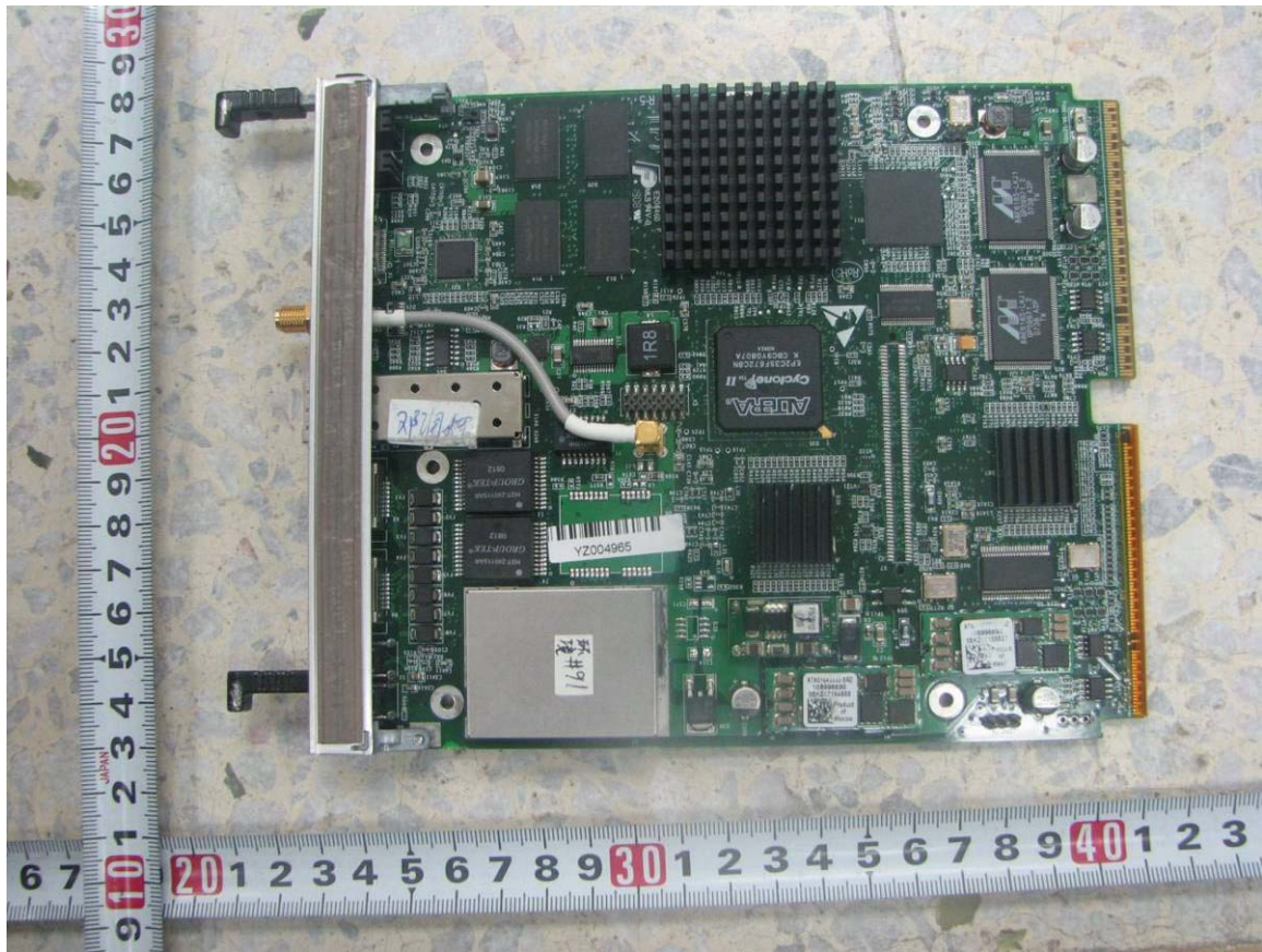
Front view of CC board
