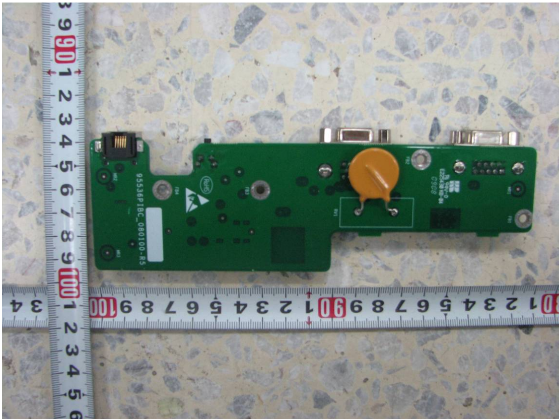
View of interface board (back side)
