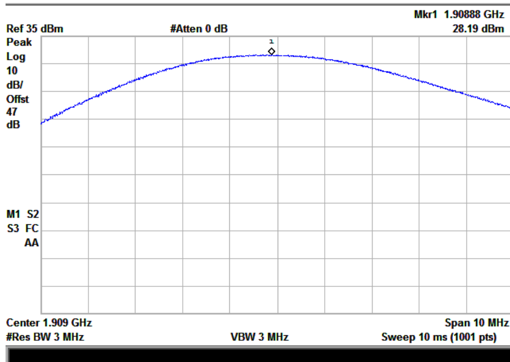
(Plot F: CDMA 1900MHz Channel = 1175)
