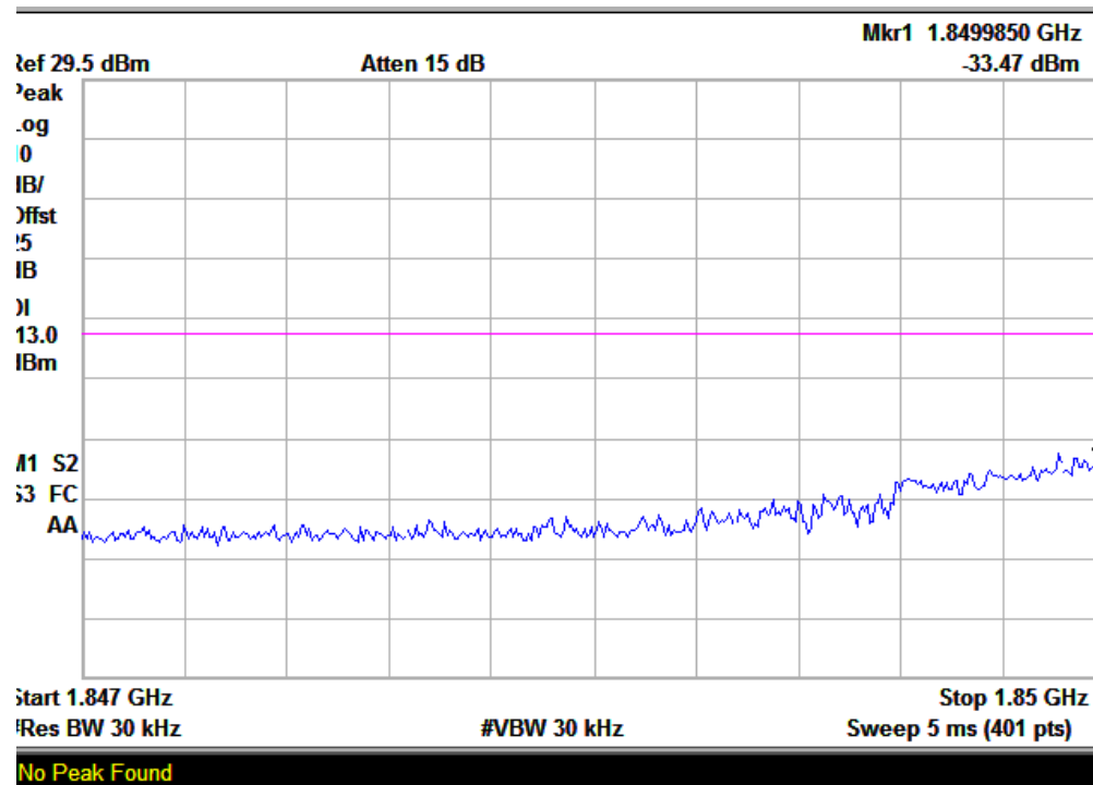
(Plot G: CDMA-EVDO 1900MHz Channel = 25)
