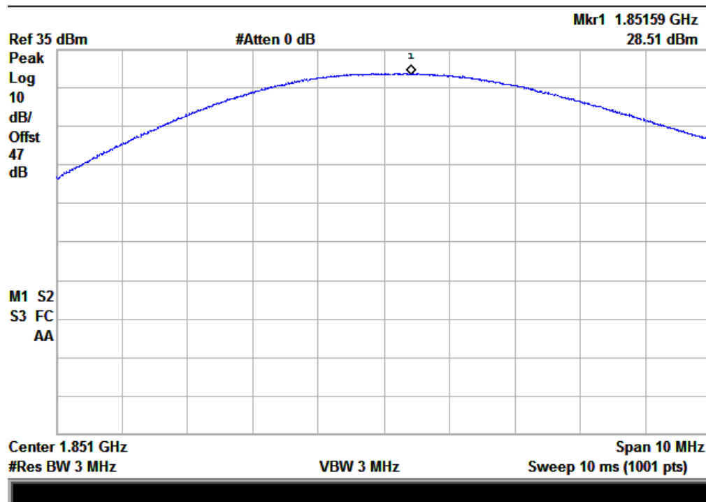
(Plot J: CDMA-EVDO 1900MHz Channel = 25)
