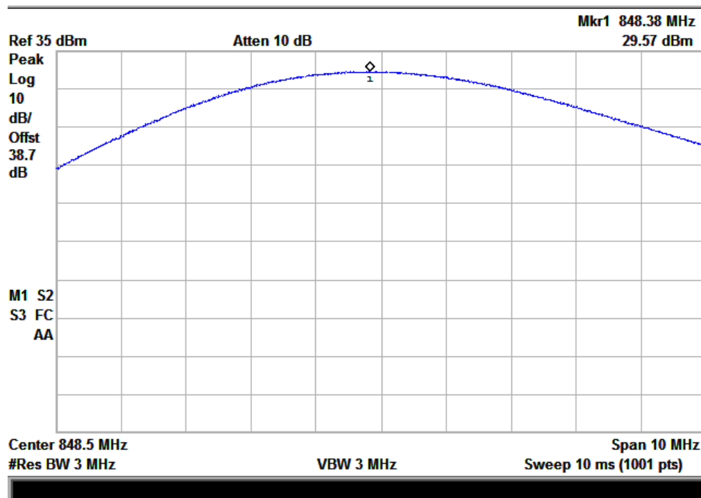
(Plot I: CDMA-EVDO 800MHz Channel = 777)
