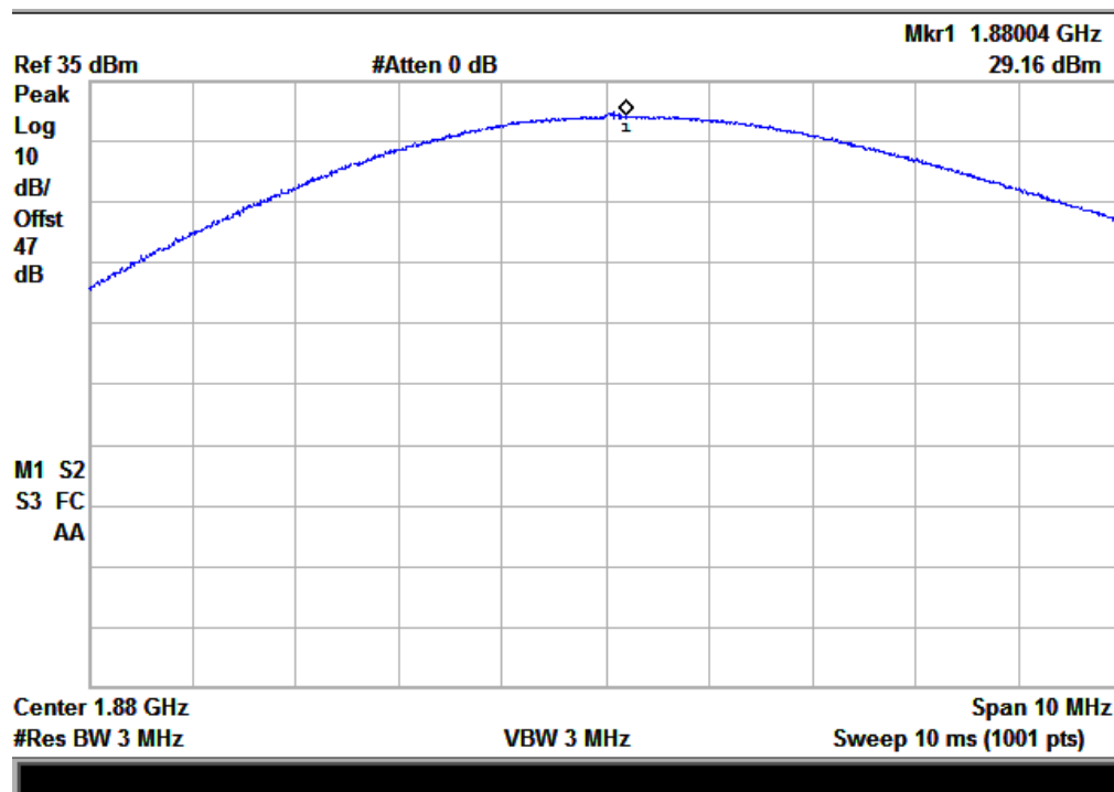
(Plot K: CDMA-EVDO 1900MHz Channel = 600)
