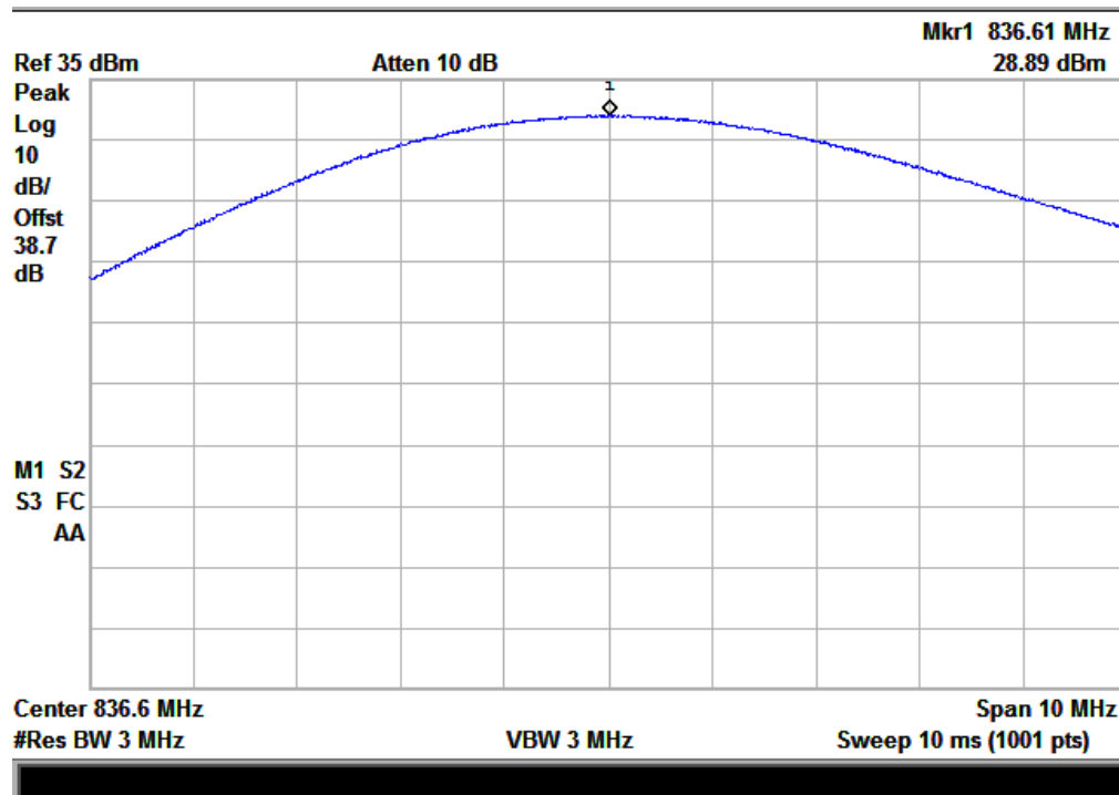
(Plot H: CDMA-EVDO 800MHz Channel = 384)
