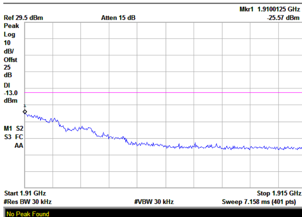
(Plot H: CDMA-EVDO 1900MHz Channel = 1175)
