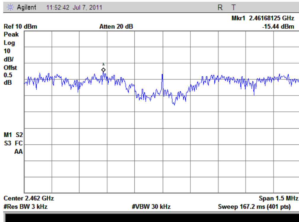
(Plot F: Channel = 11)
