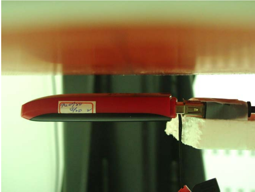
USB Configuration 2 with Phantom 10 mm Gap for Back-off SAR (Horizontal Down)
