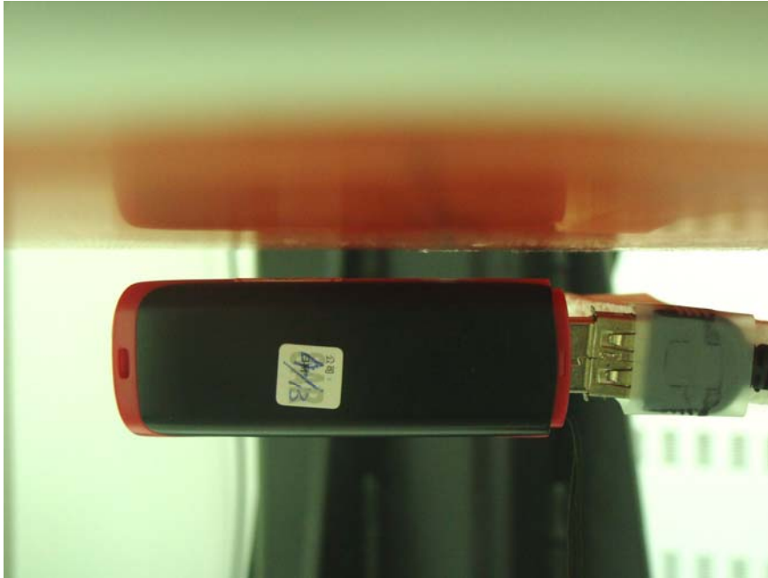
USB Configuration 3 with Phantom 5 mm Gap (Vertical Front)
