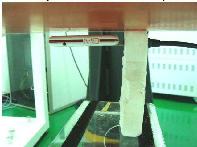
USB Configuration 2 (Horizontal Down) Straight mode with Phantom 5 mm Gap
