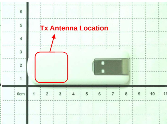
DUT is in Close mode - Bottom View
