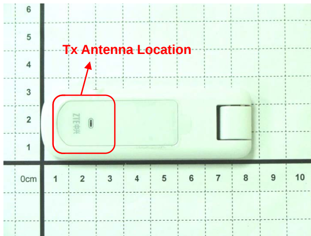
DUT is in Close mode - Top View
