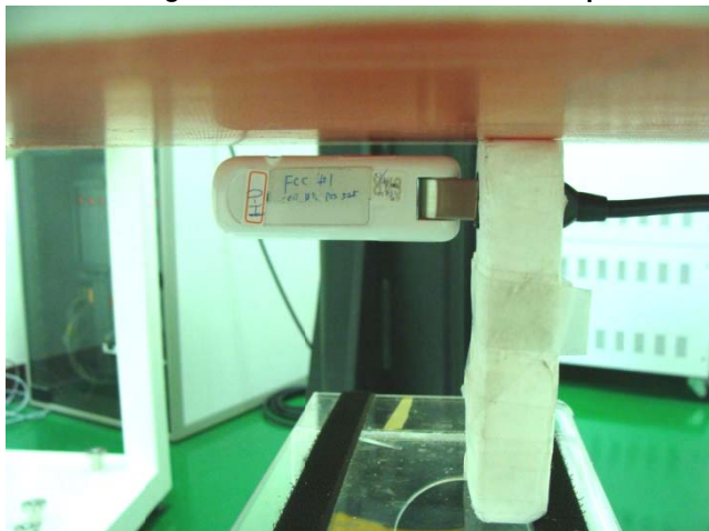
USB Configuration 3 (Vertical Front) Straight mode with Phantom 5 mm Gap
