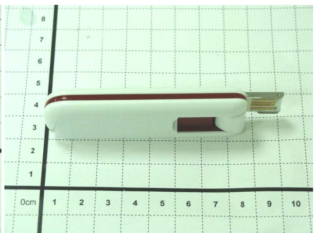
DUT is in Straight mode (0 degree) - Side View
