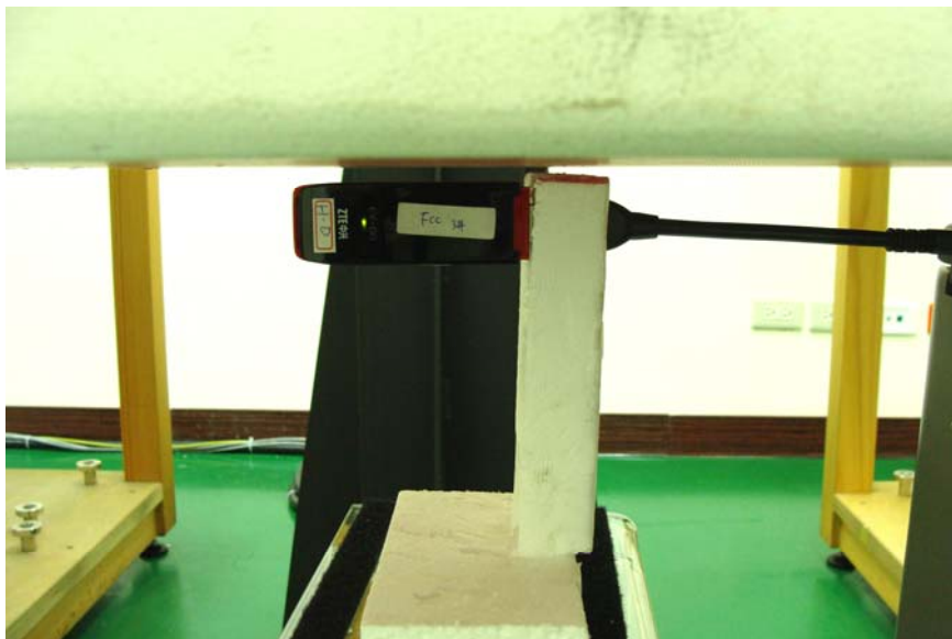
USB Configuration 4 with 5 mm separation (Vertical Back)
