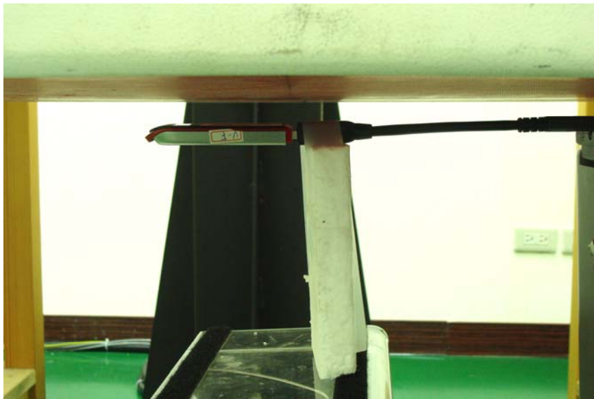
USB Configuration 2 with 15 mm separation for Back-Off SAR (Horizontal Down)
