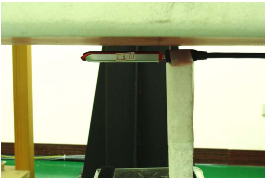
USB Configuration 2 with 5 mm separation (Horizontal Down)
