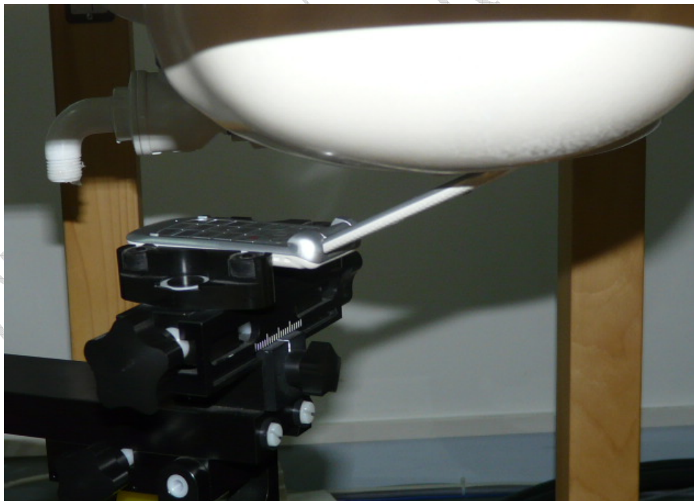
Picture 4: Head SAR tilt position 1
