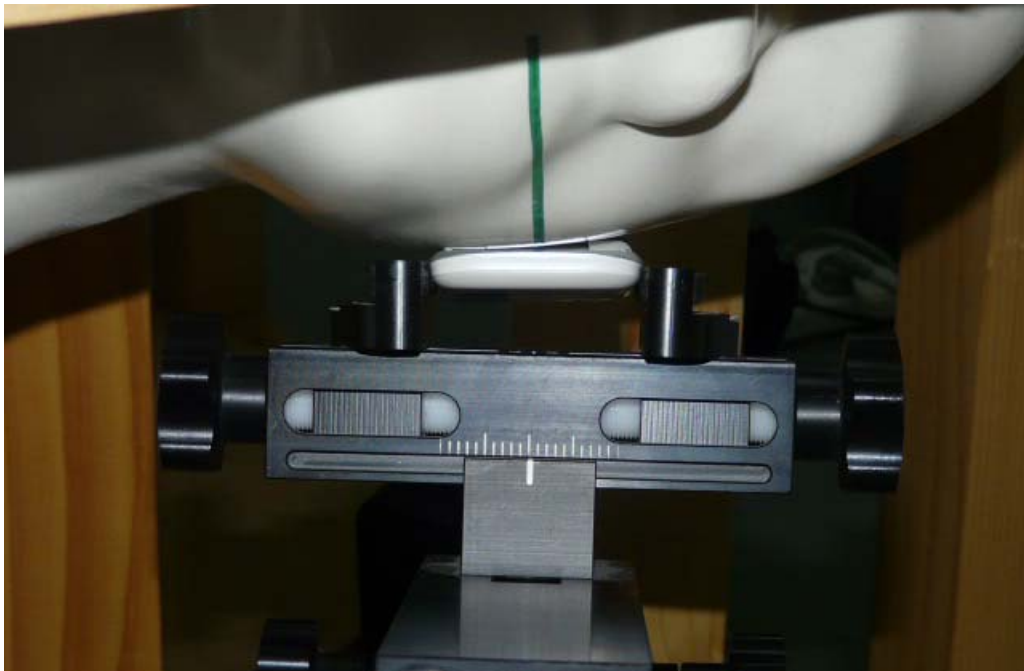
Picture 3: Head SAR touch position 2
