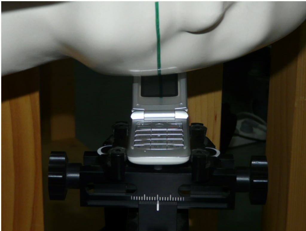
Picture 5: Head SAR tilt position 2
