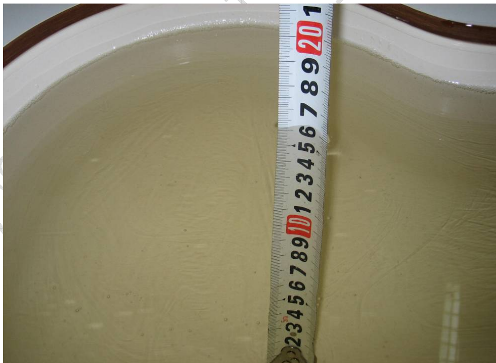
Picture 8 Liquid Depth at Ear Reference Point for 835MHz Head Liquid
