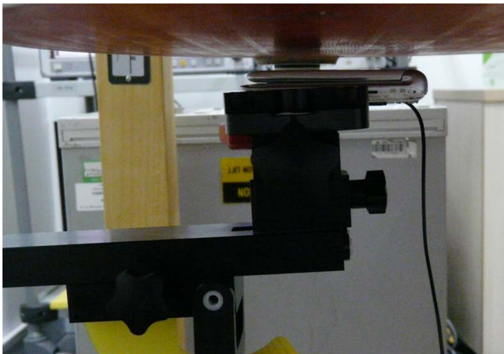
Picture 7: Body SAR front to the phantom
