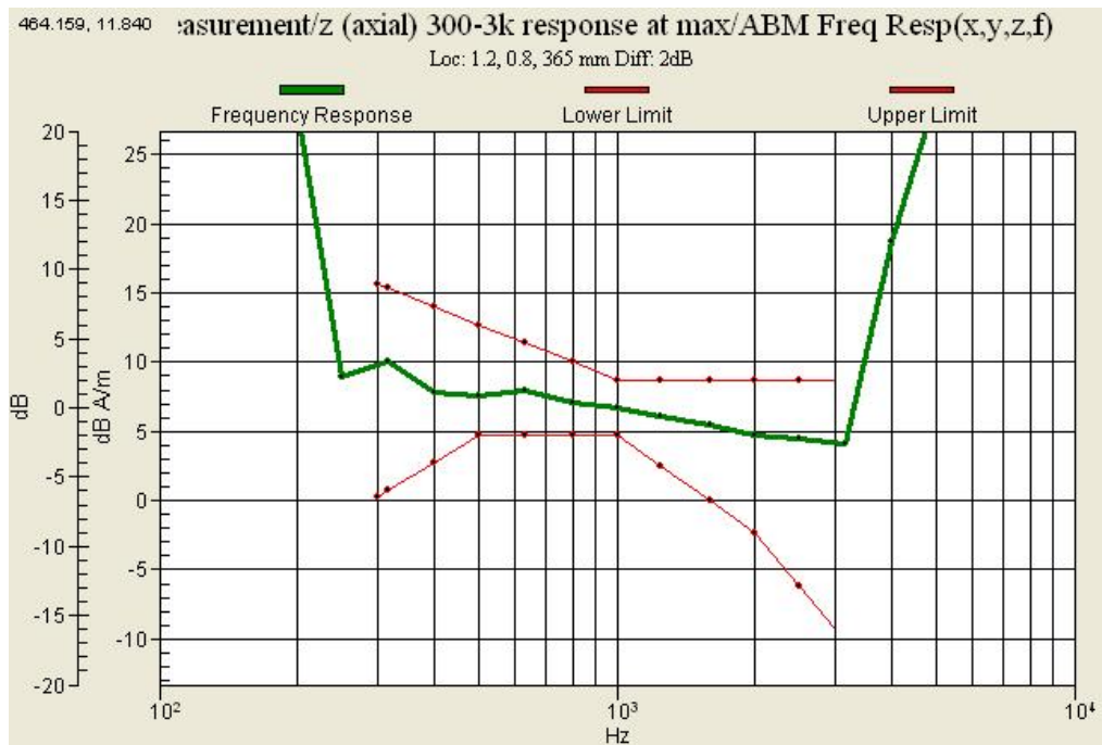
Graph 3 : CDMA 800 (CH 777) Frequency Response
