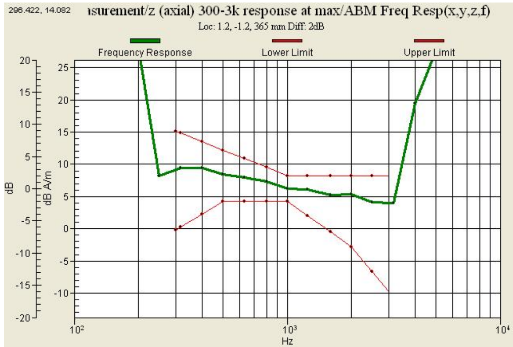
Graph 9 : AWS 1700(CH 875) Frequency Response
