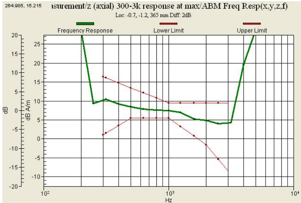
Graph 5 : PCS 1900 (CH 600) Frequency Response
