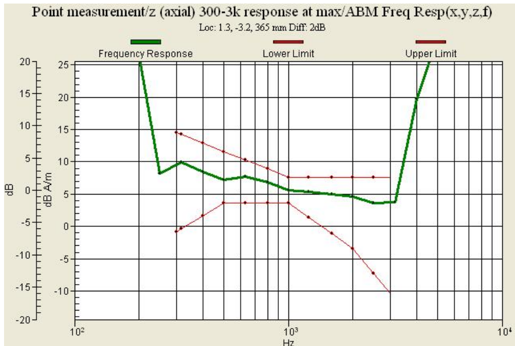
Graph 6 : PCS 1900 (CH 1175) Frequency Response
