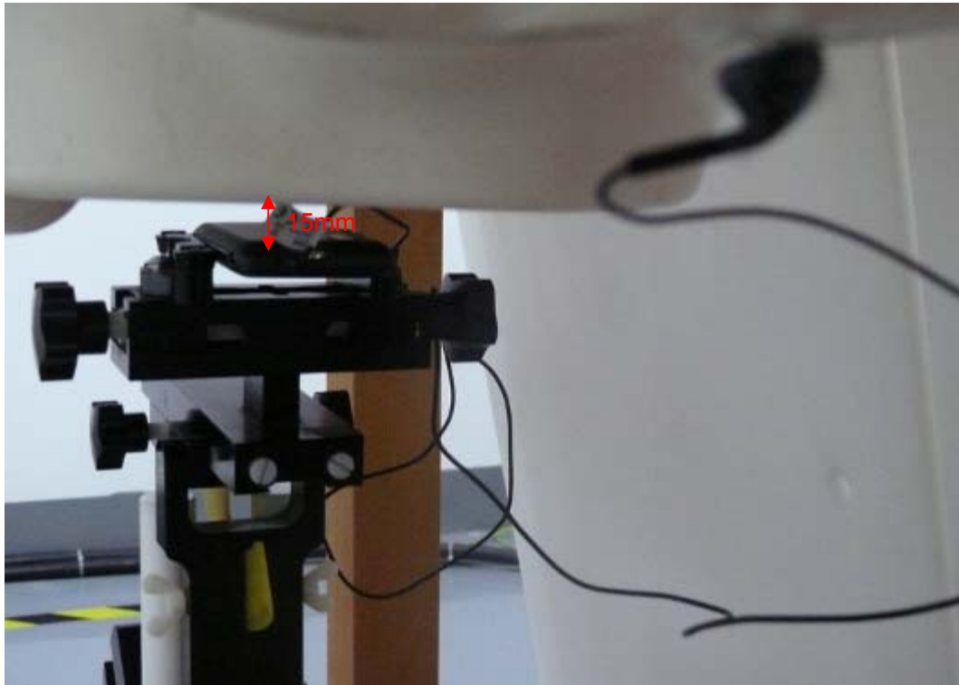
Picture 13: Body with earphone, The EUT display towards ground, the distance from handset to the bottom of the Phantom is 15mm
