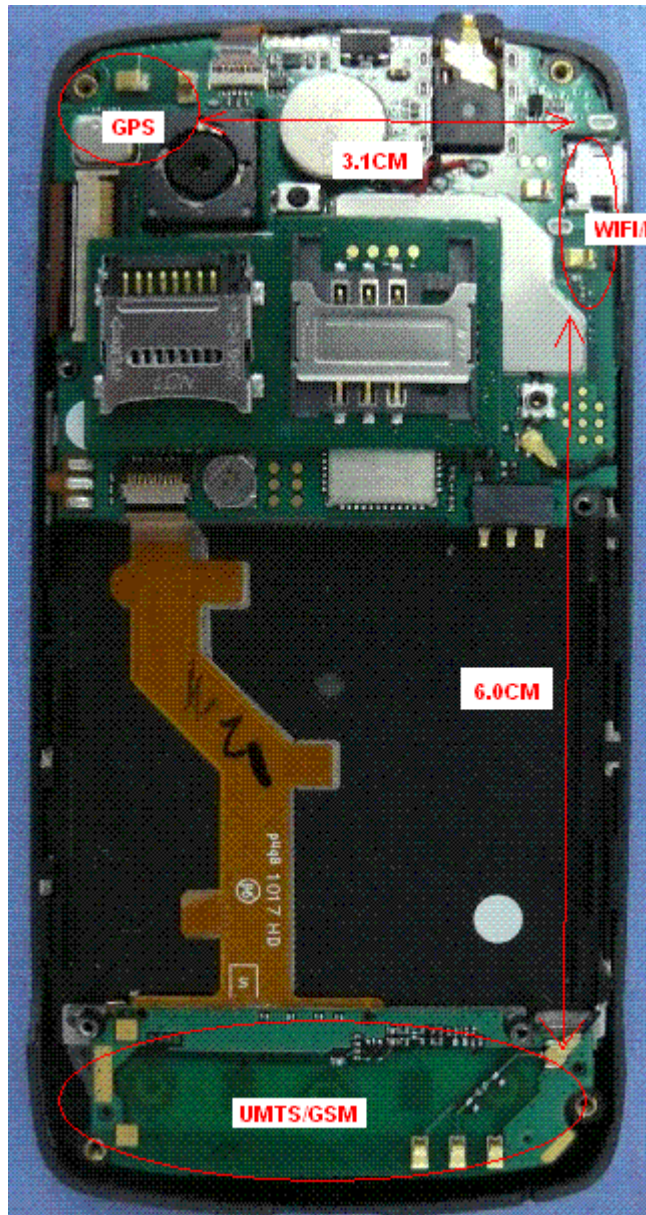
Picture 6: Constituents of EUT
