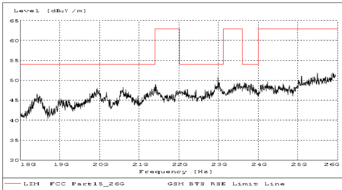
Fig. 57 Radiated emission: 18 GHz - 26 GHz
