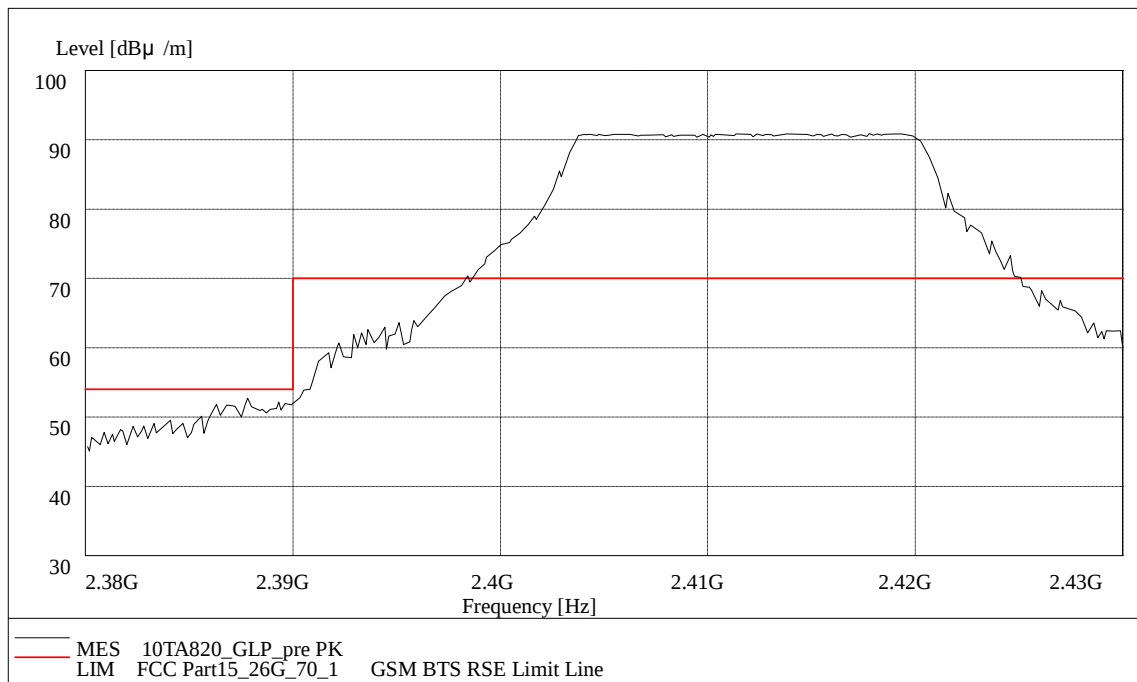
Fig. 46 Radiated Spurious Emission (Power): 802.11g, 2.38 GHz - 2.43GHz
