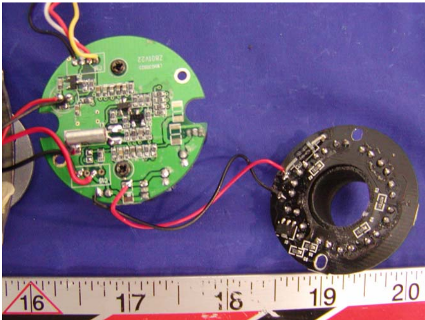
EUT – CMOS Board Bottom View
