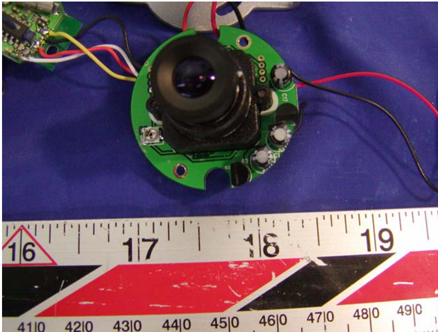
EUT – CMOS Board Top View
