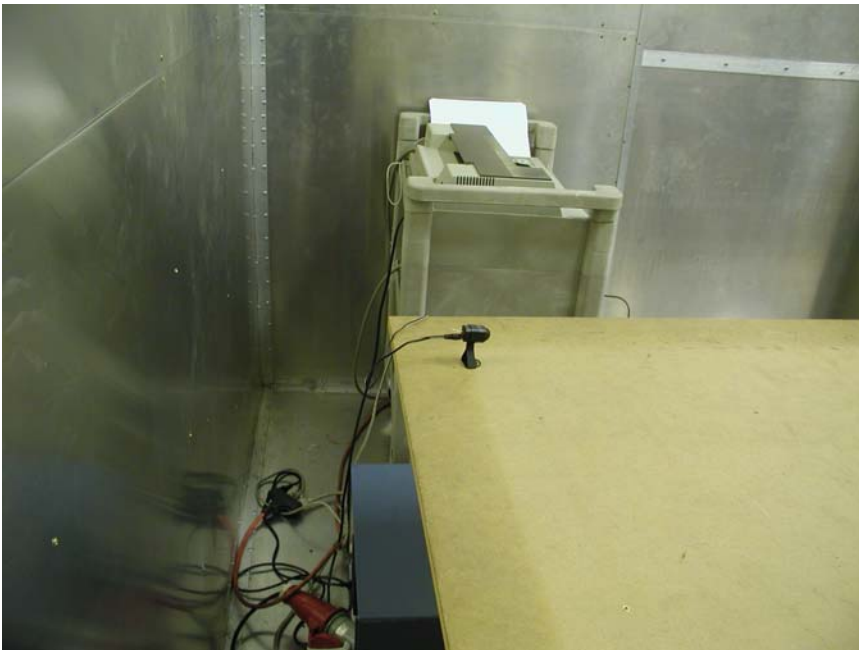
Transmitter Conducted Emission - Side View
