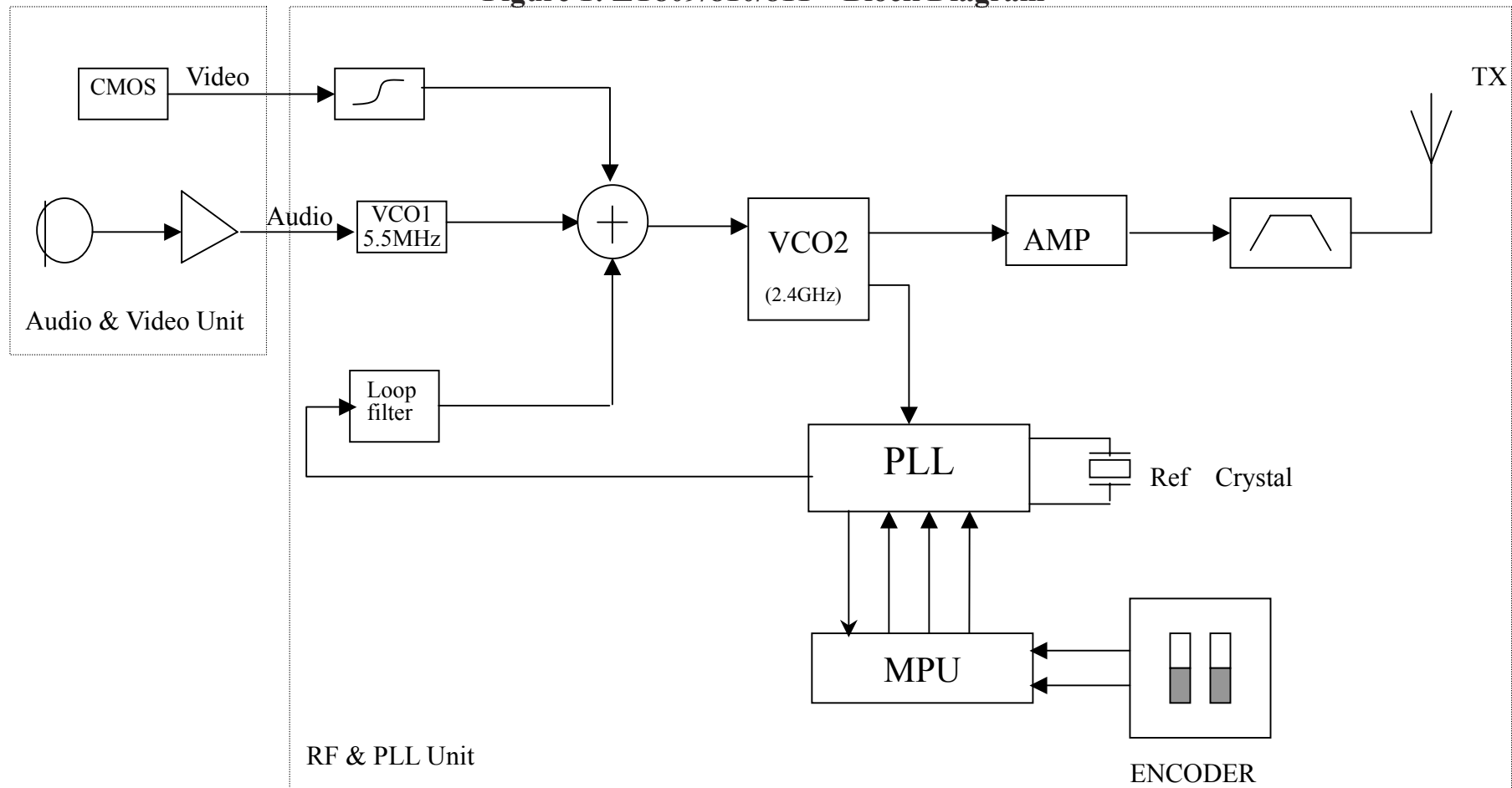
Figure 1: ZT809/810/811 Block Diagram
