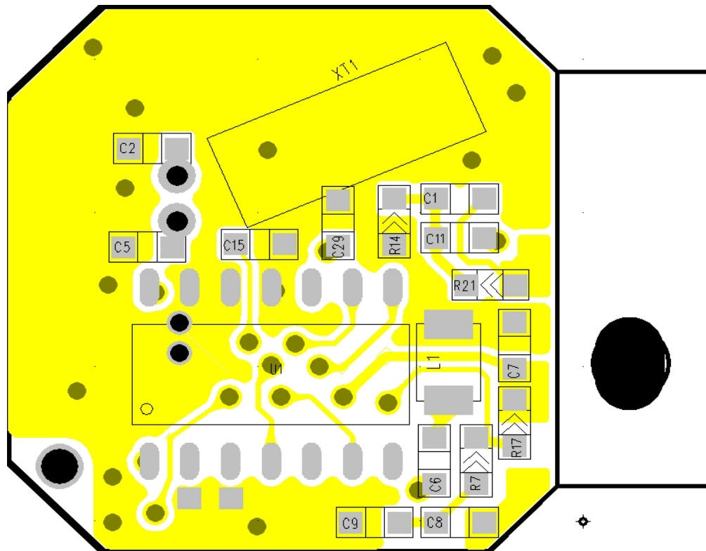
FIGURE2 BOTTOMVIEW OF RF.PCB
