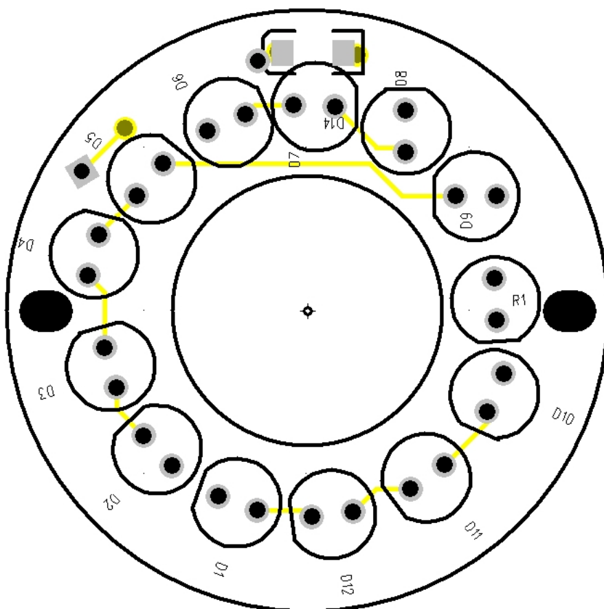
Figure3 TOPVIEW OF CMOS.PCB
