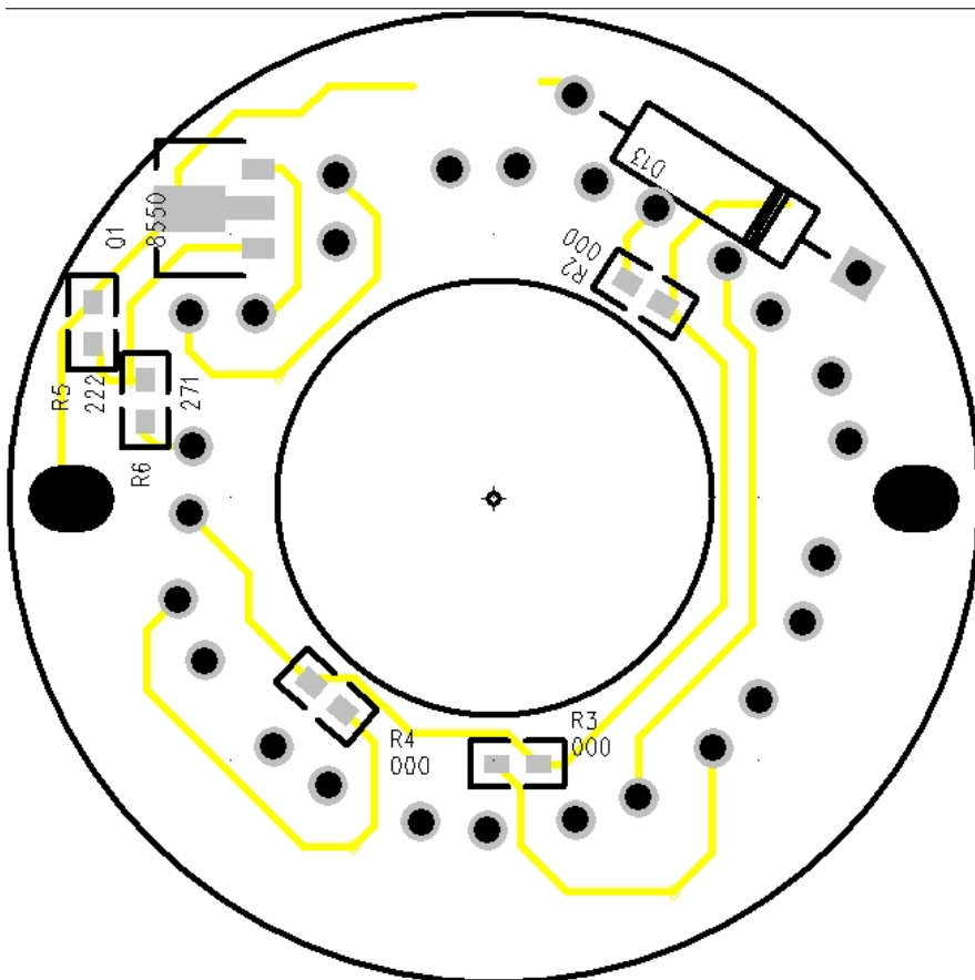
Figure4 BOTTOMVIEW OF LED.PCB
