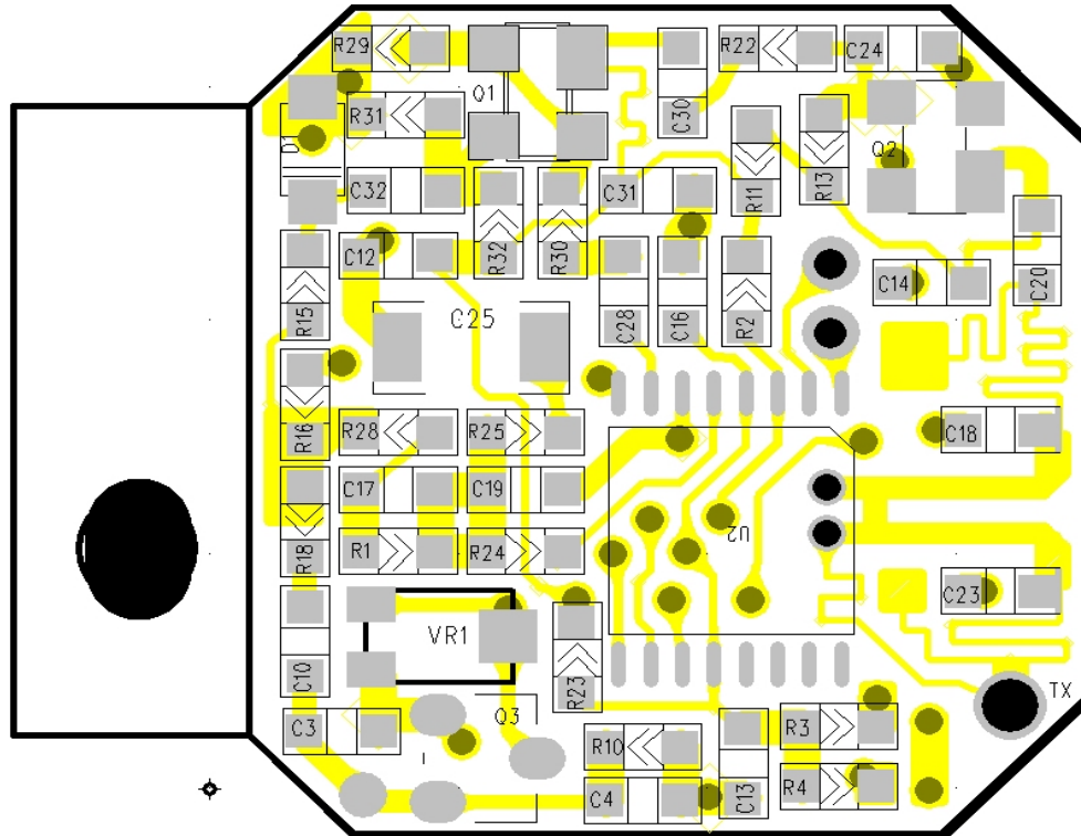
FIGURE1 TOPVIEW OF RF.PCB
