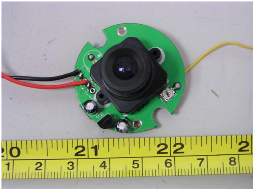
EUT-PCB View-1
