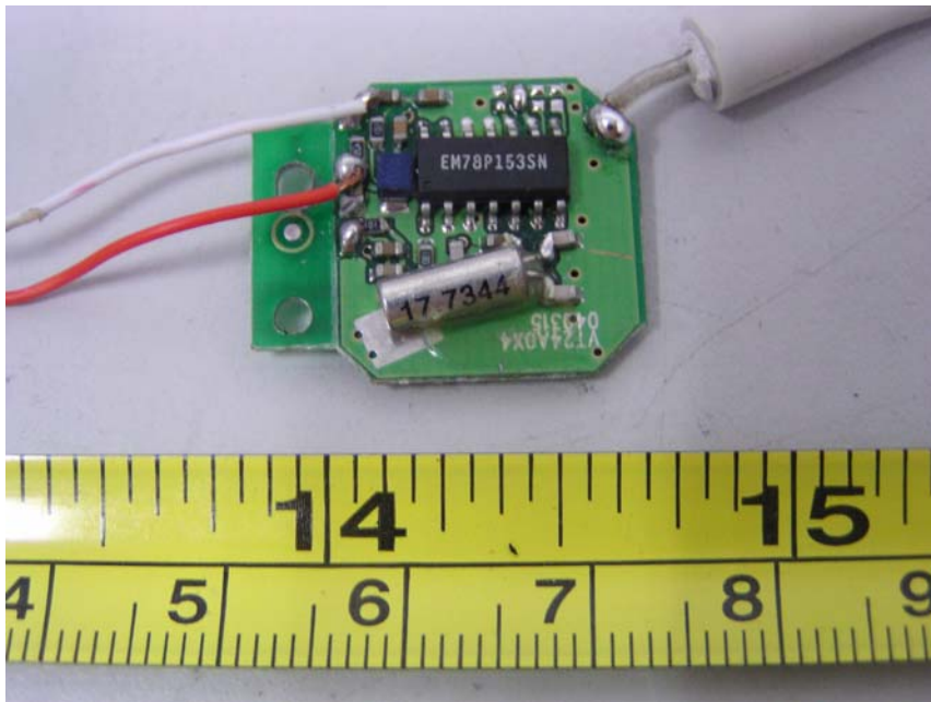
EUT-PCB View-3
