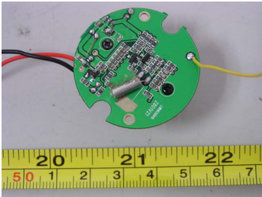
EUT-PCB View-2
