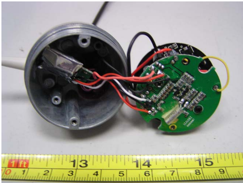
EUT-Internal View-3
