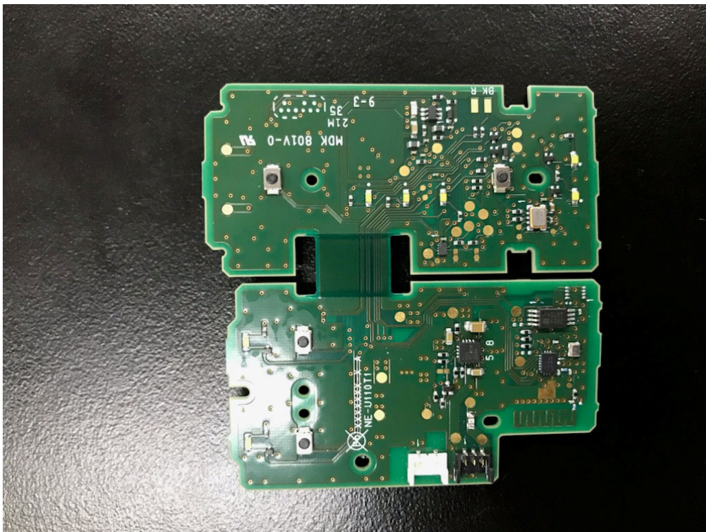
PCB_Back side
