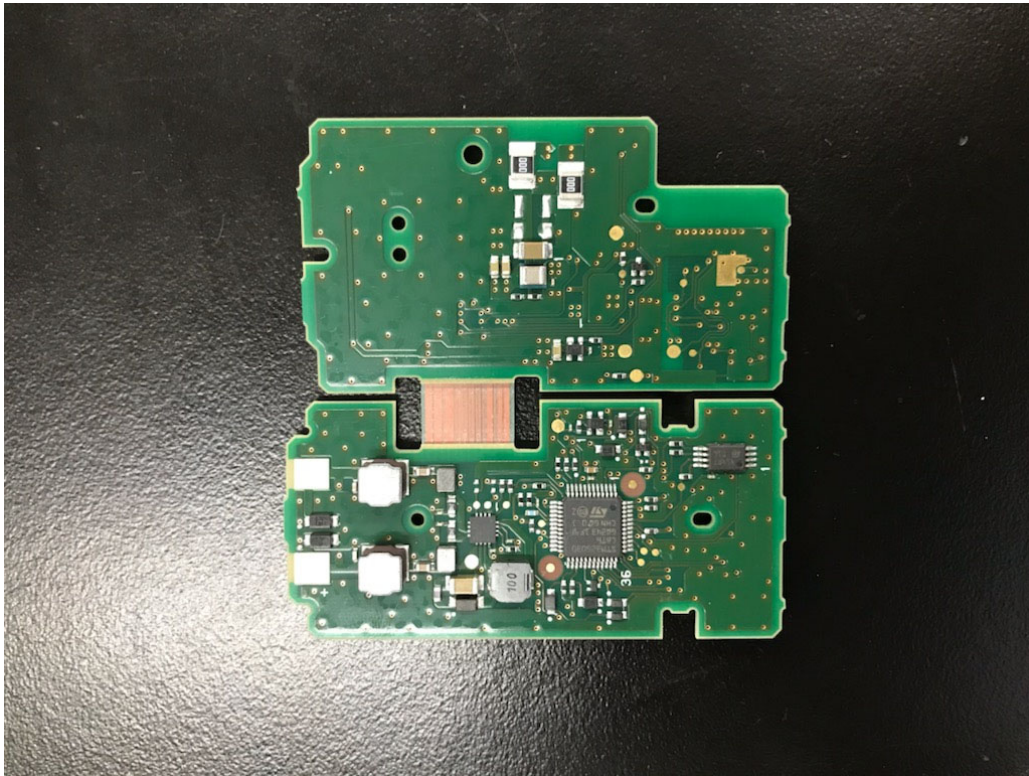
PCB_Front side
