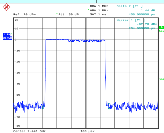
2-DH1
