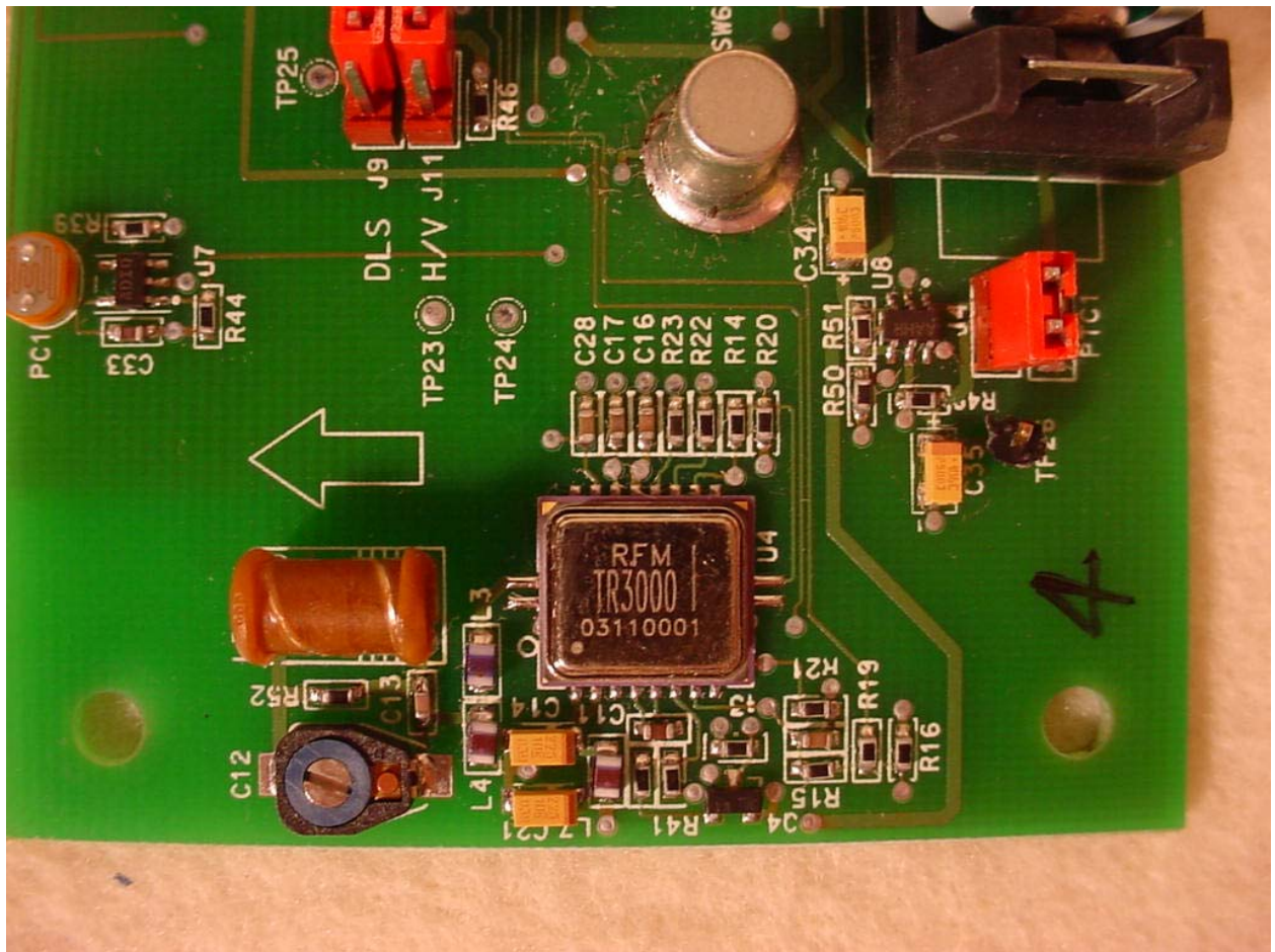
Figure 7: RF Circuitry
