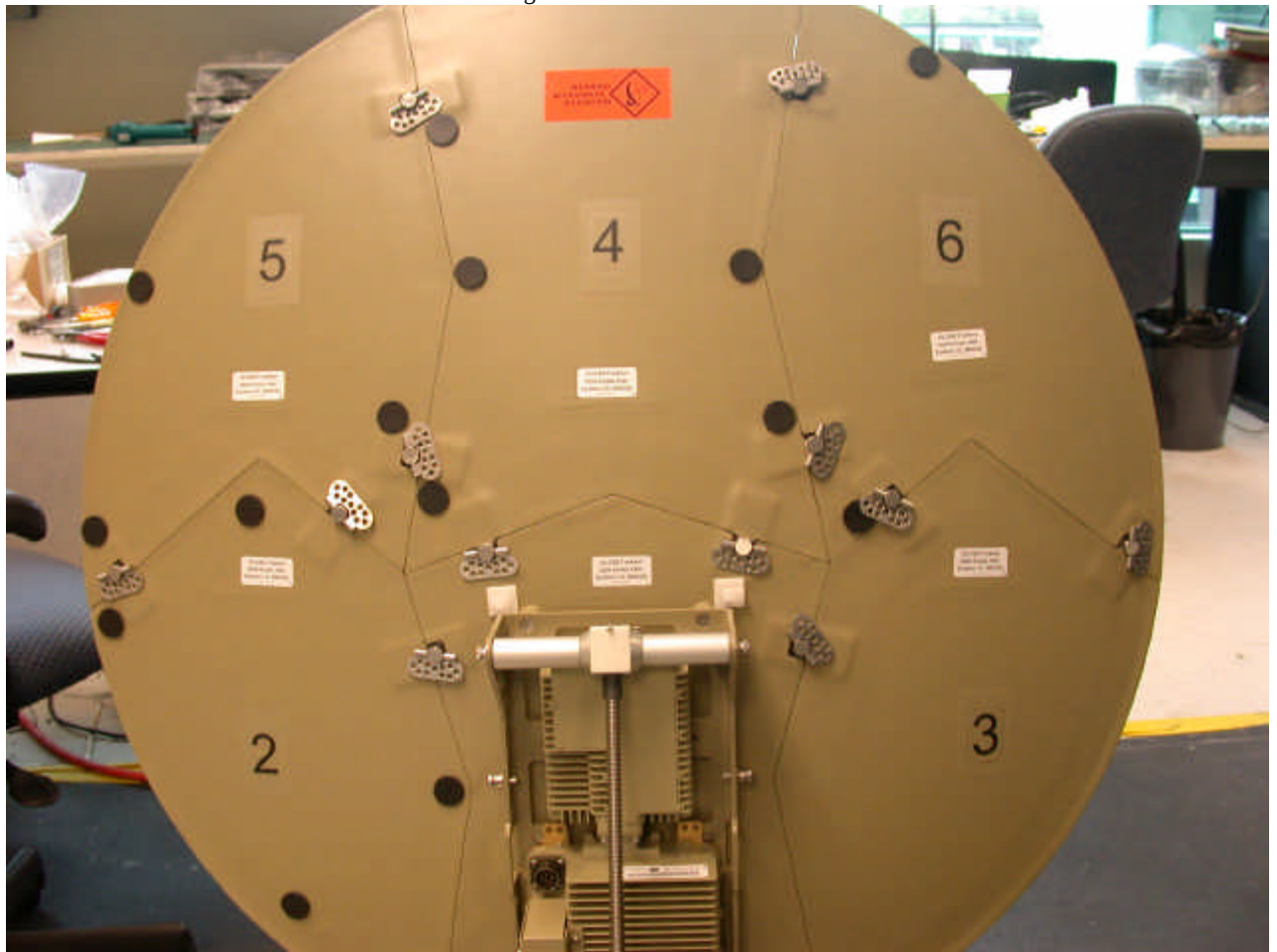
Norsat 5200-KUAA-IP – Microwave radiation warning label Location
