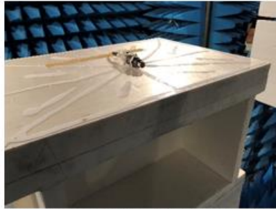
Test setup in Axis XY (worst case position):
