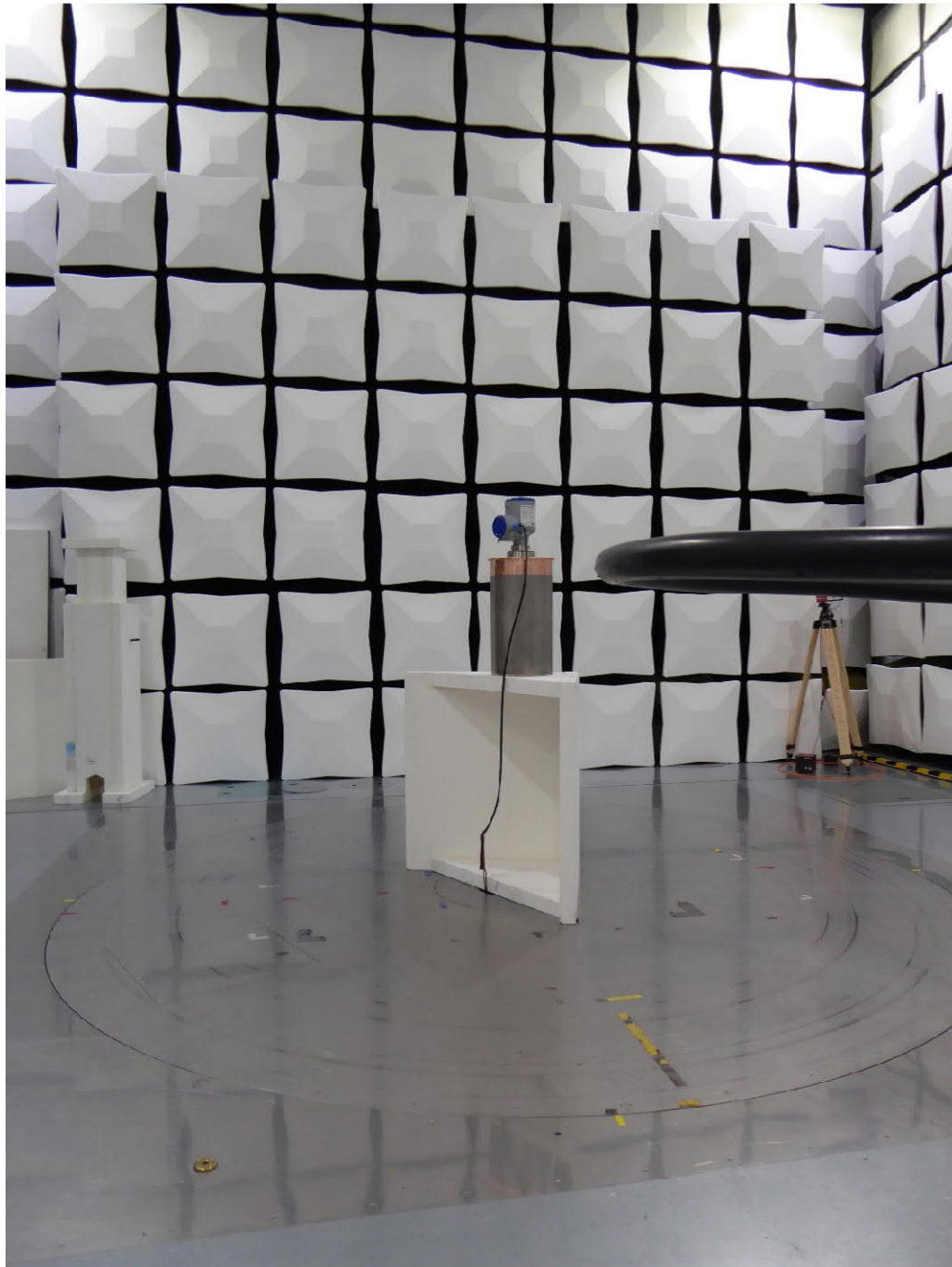
Test setup semi anechoic chamber (<30 MHz)
