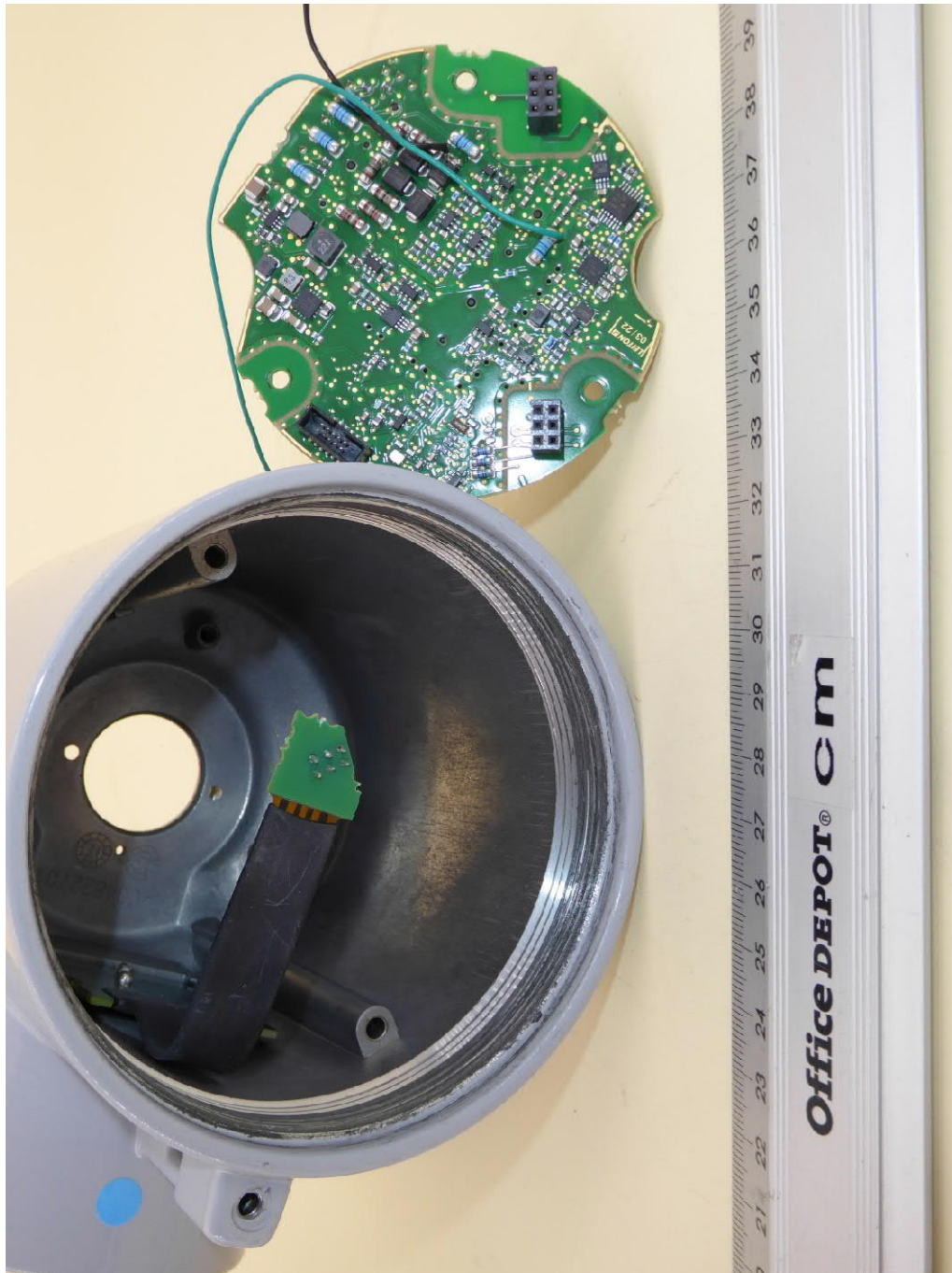
Internal view, sensor board removed
