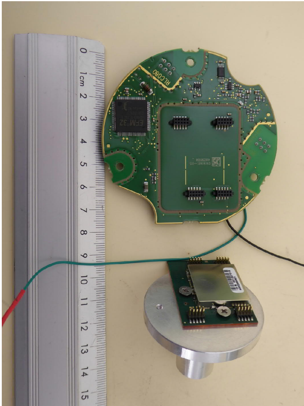
Sensor 80 GHz, RF-module removed
