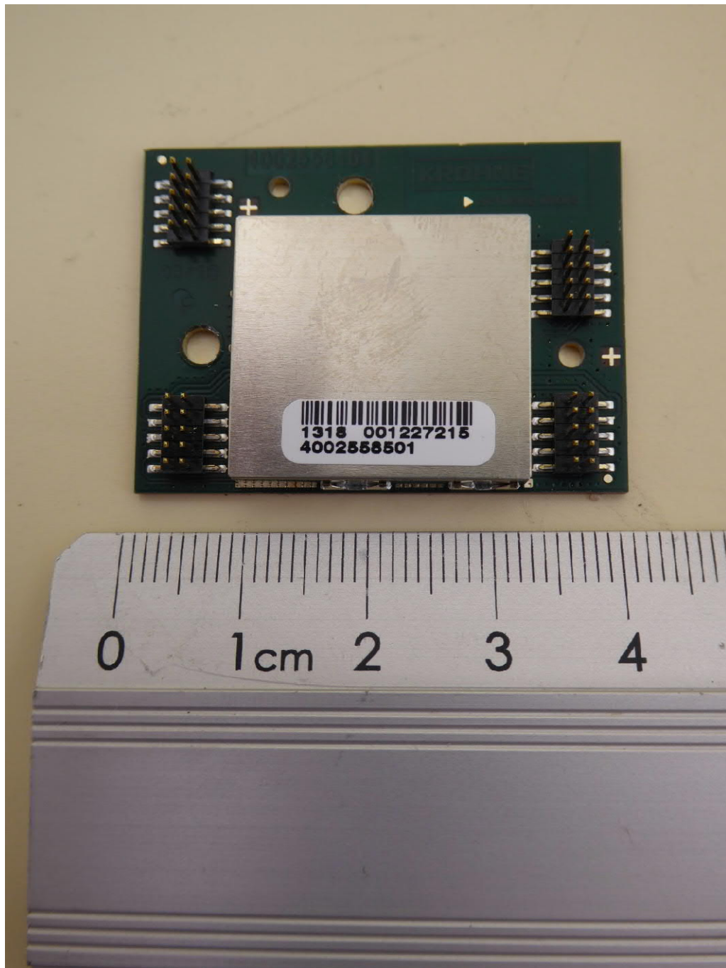
RF module, PCB, top view
