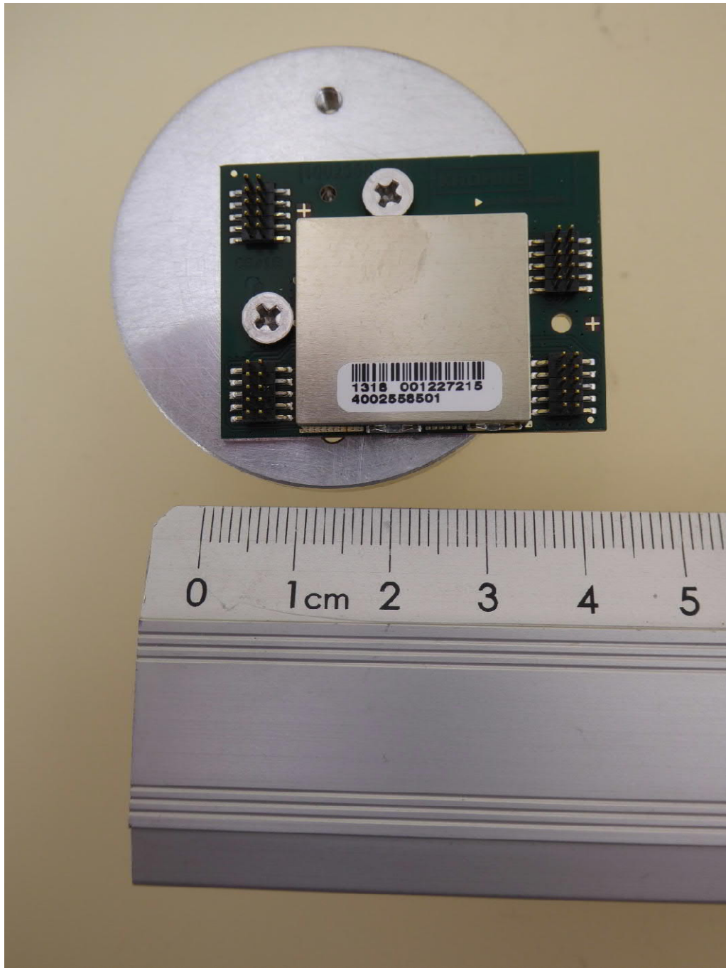
RF module mounted on waveguide
