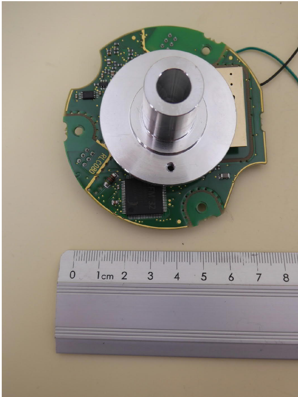
Sensor 80 GHz with RF-module
