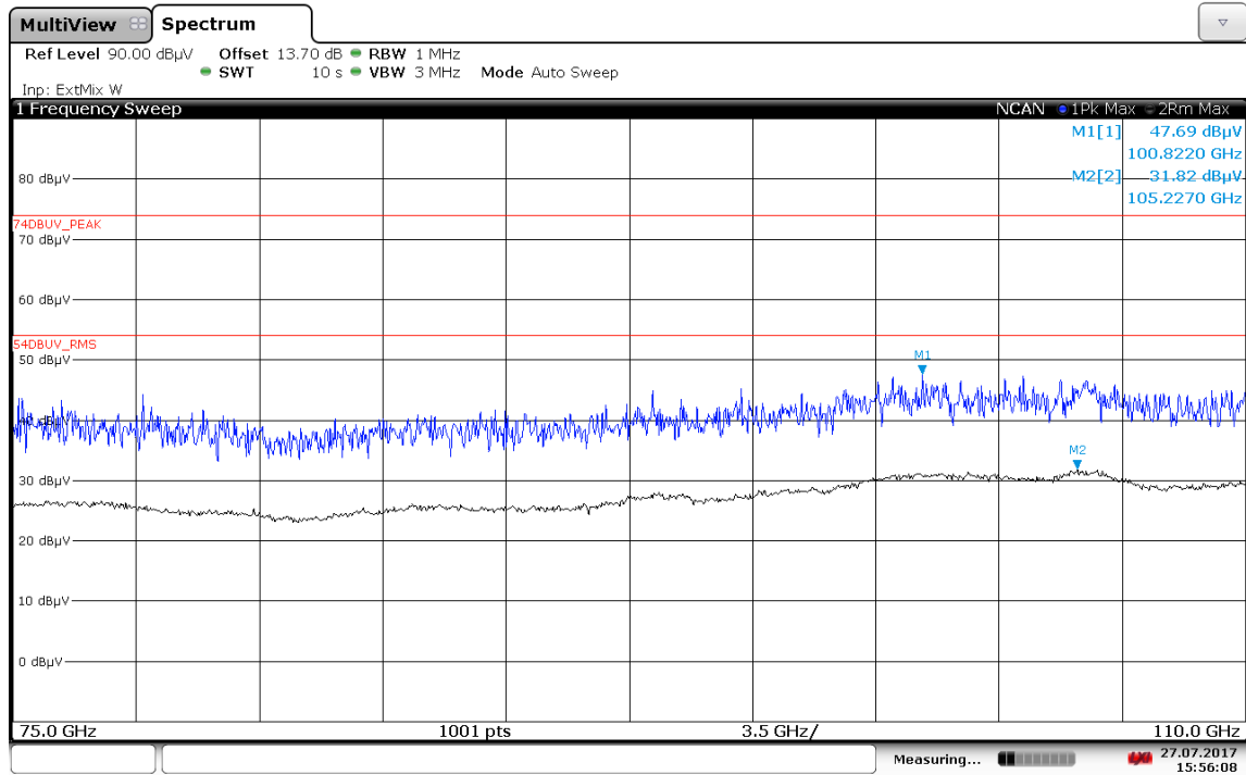
Plot 10: 75 GHz – 110 GHz, PEAK/RMS-measurement, special test mode, f_{low}/f_{mid}/f_{high}
