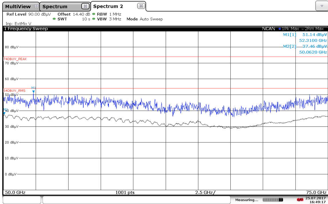
Plot 9: 50 GHz – 75 GHz, PEAK/RMS-measurement, special test mode, f_{low}/f_{mid}/f_{high}
