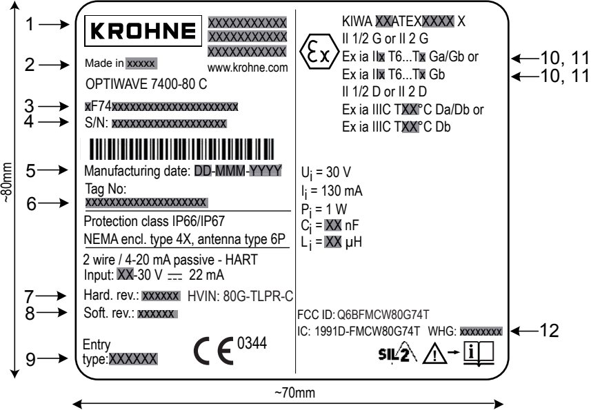
Nameplate for Ex ia 4-20mA/HART version of OPTIWAVE 7400-80 C
