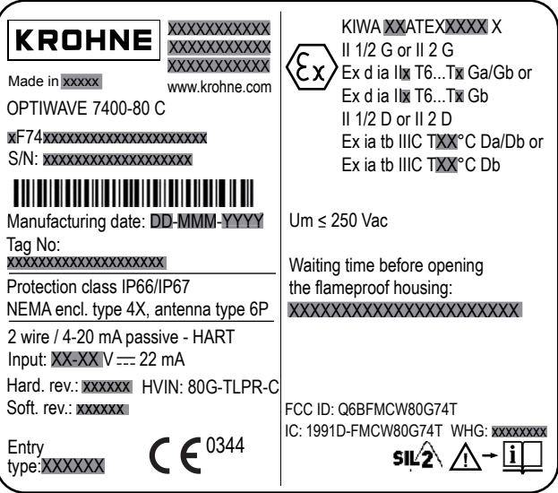
Nameplate for Ex d ia 4-20mA/HART version of OPTIWAVE 7400-80 C
