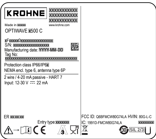
OPTIWAVE x500 C (LPR)-Lens 20/25/40/70mm antenna
