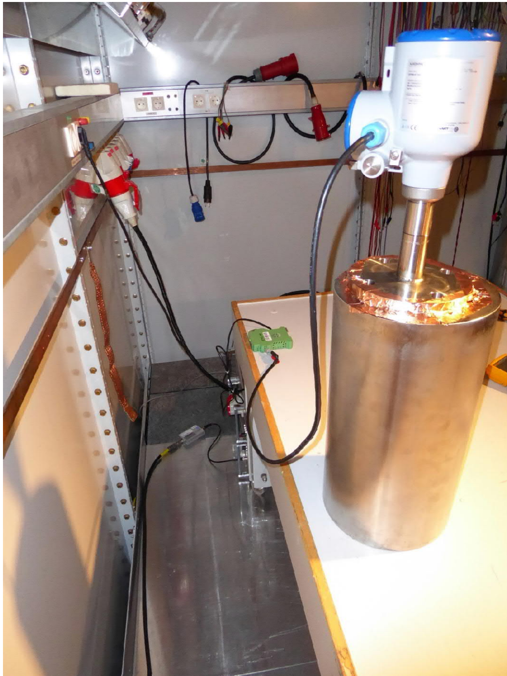
Test AC power line conducted emissions
