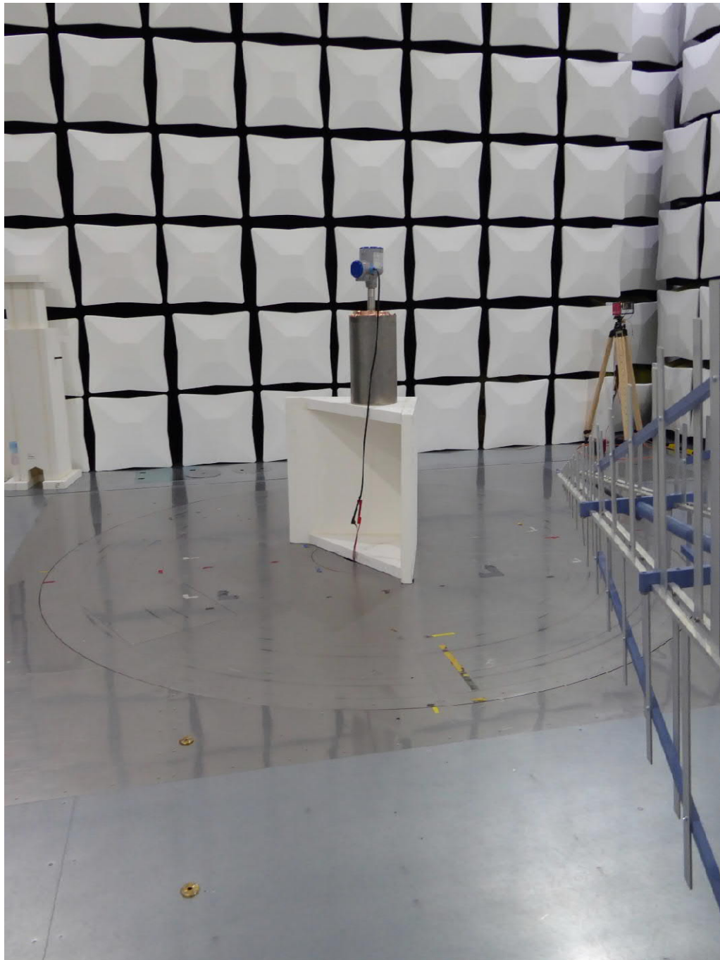
Test setup semi anechoic chamber (<1 GHz)
