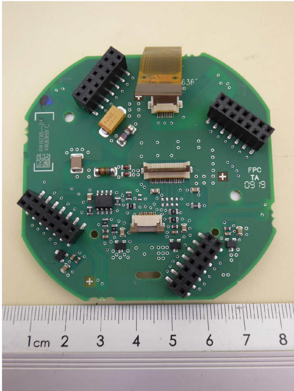
Display PCB, top view
