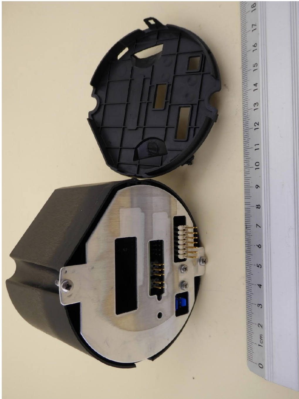
Internal view, converter unit opened
