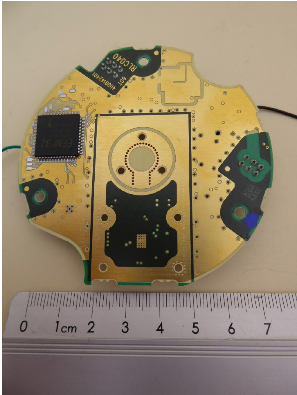
Sensor unit, PCB, top view, shielding removed
