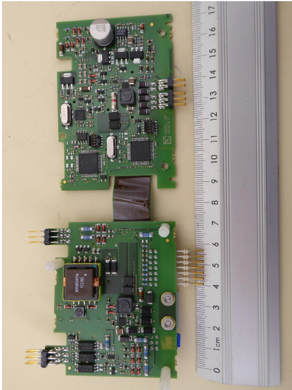
Converter PCB, top view
