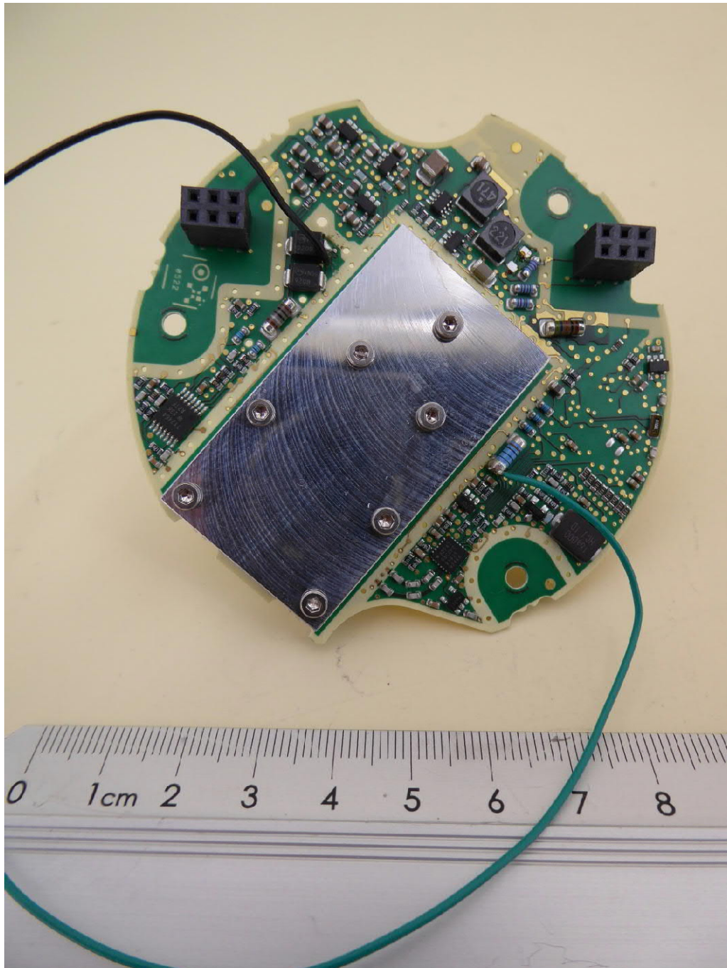
Sensor unit, bottom view
