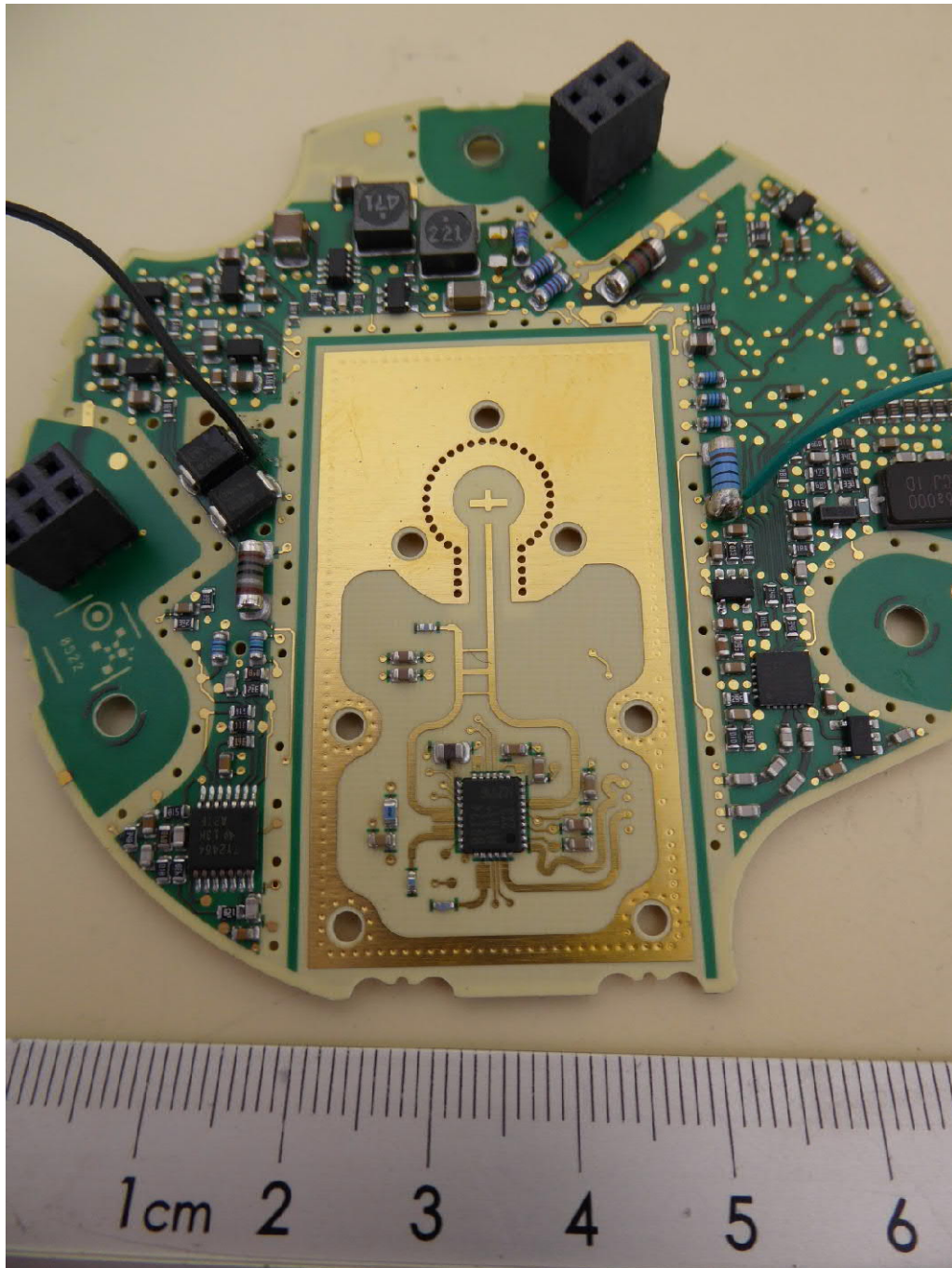
Sensor unit, PCB, bottom view, shielding removed
