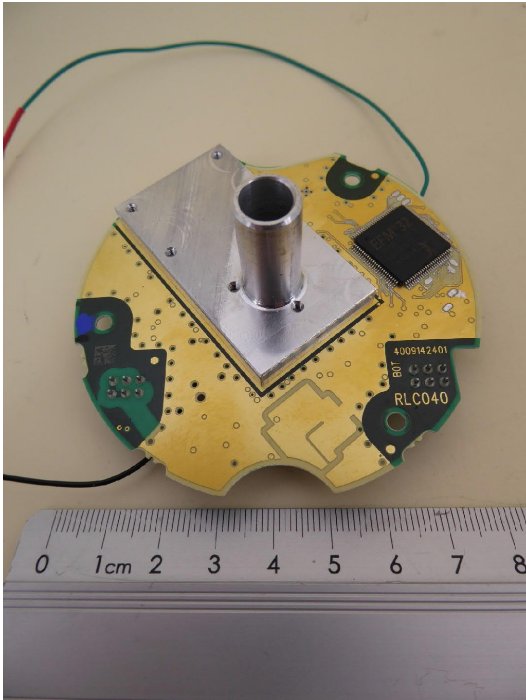
Sensor unit, top view
