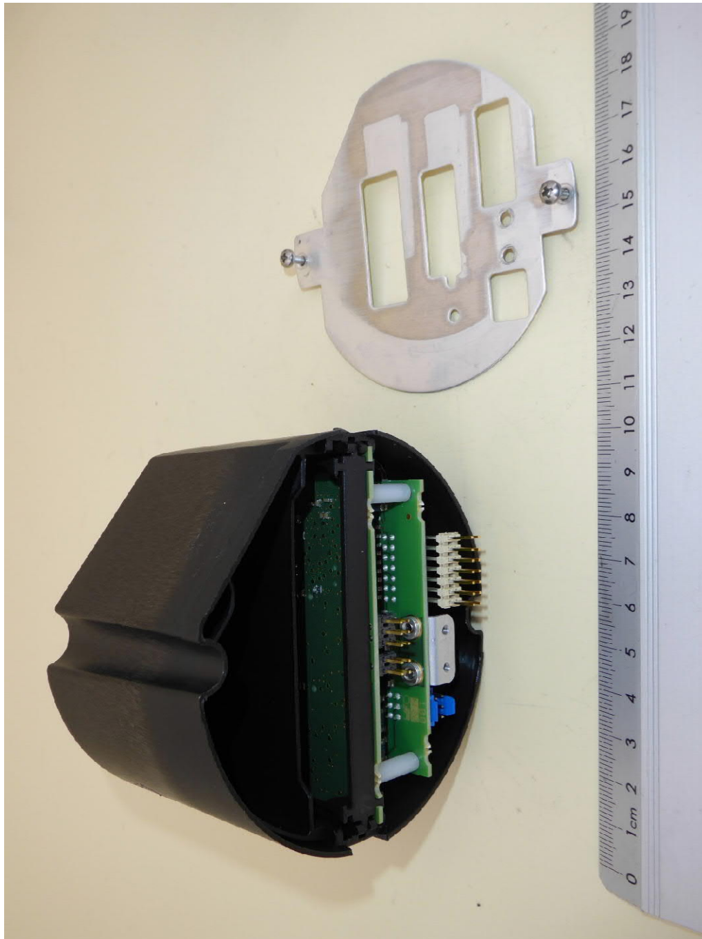
Internal view, converter unit, housing opened
