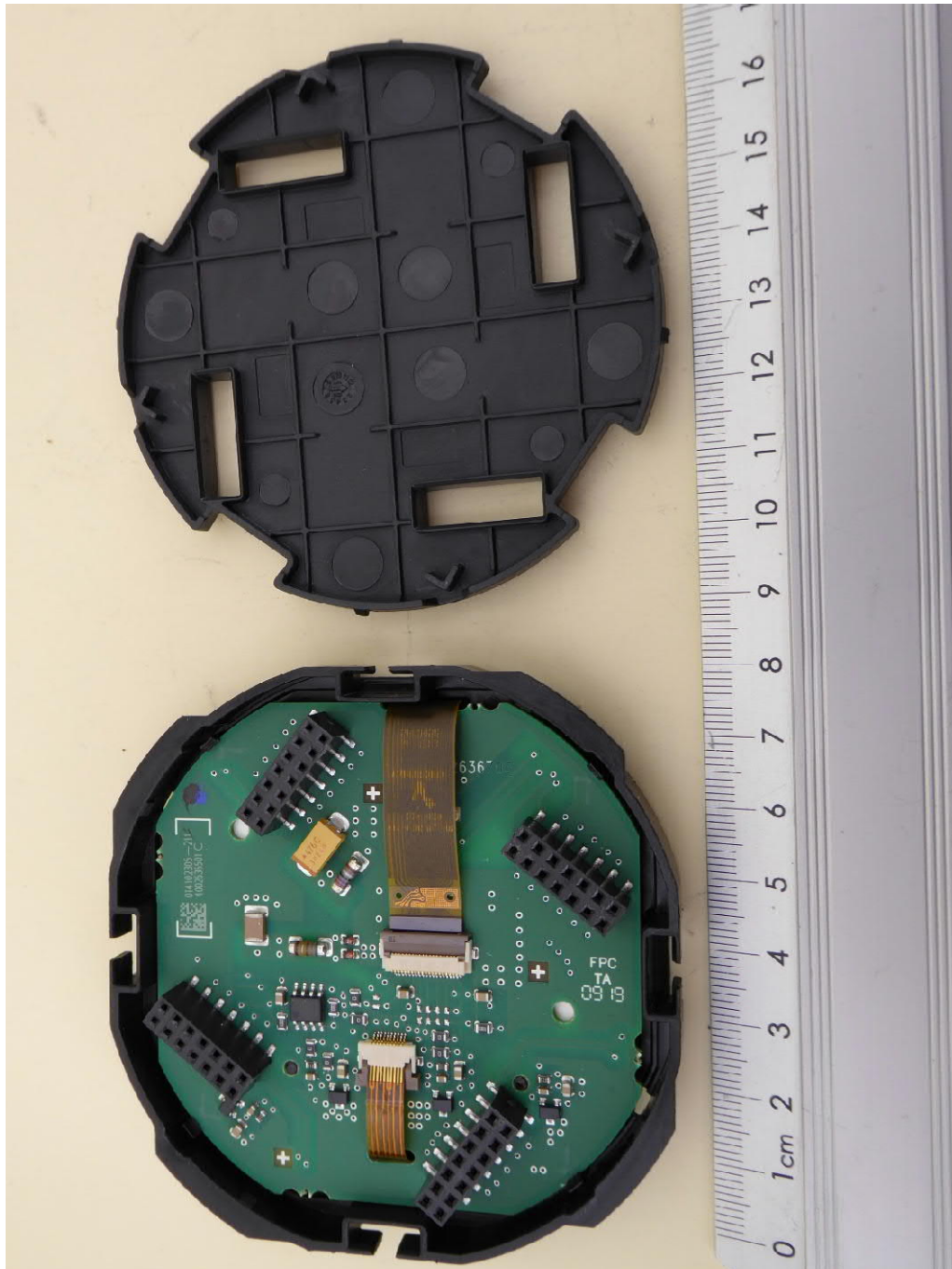
Internal view, display housing opened
