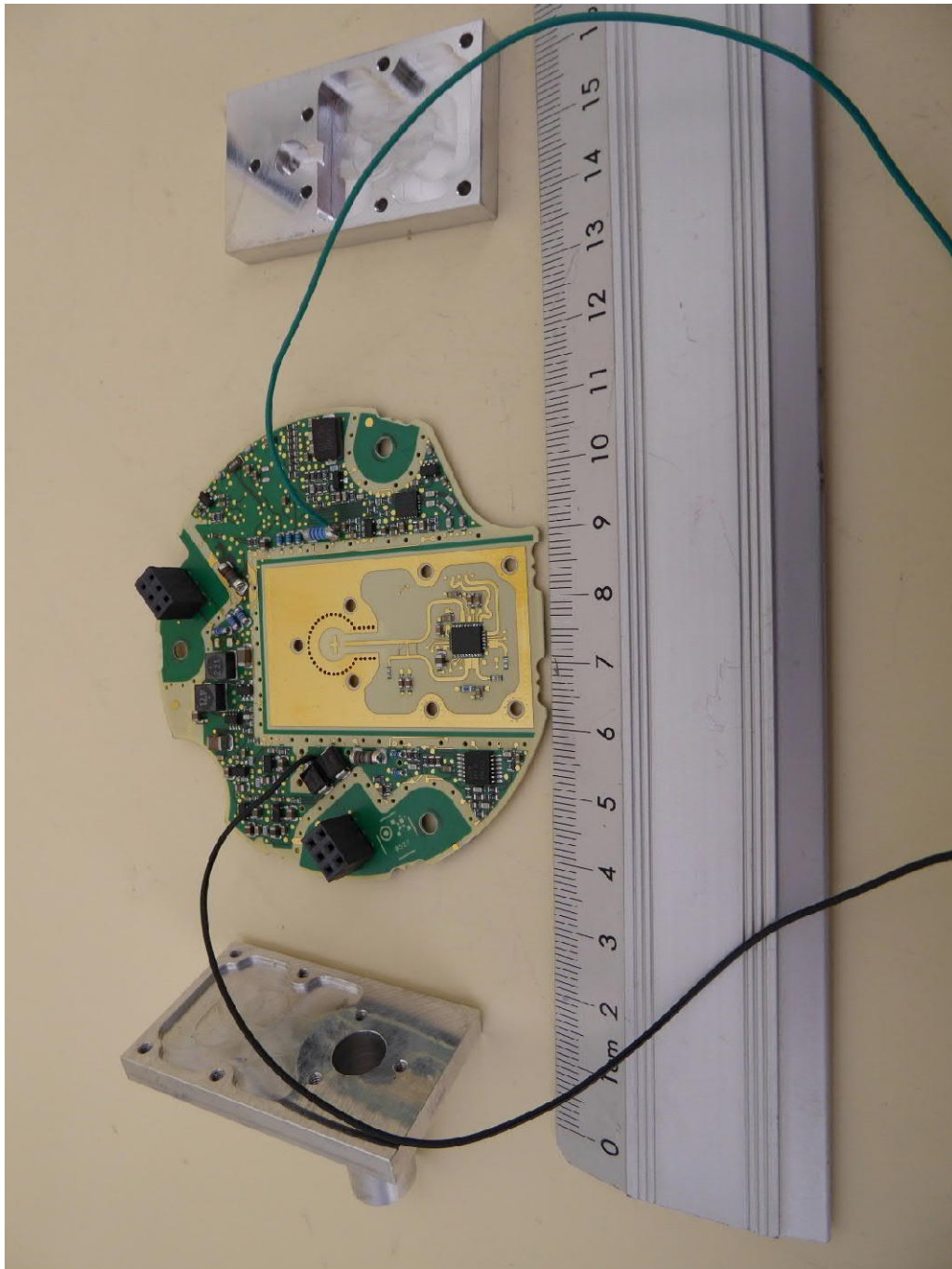
Sensor unit, shieldings removed
