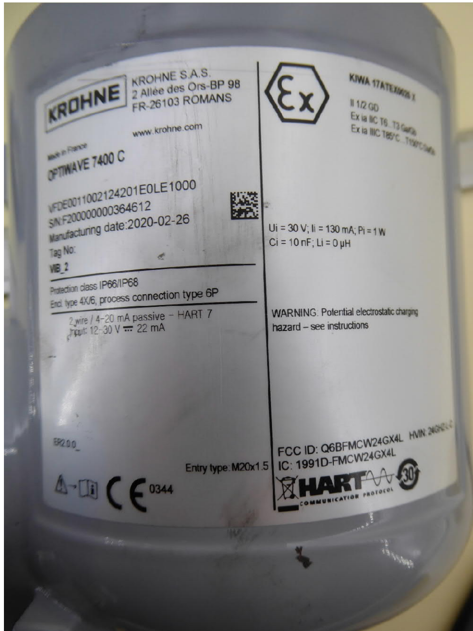
Type plate view
