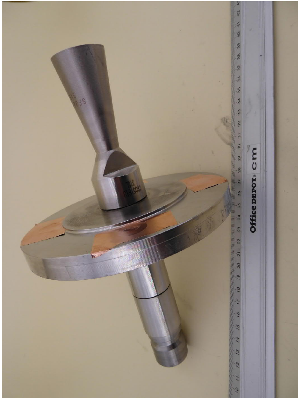
Antenna used for the measurements, with adaptor plate
