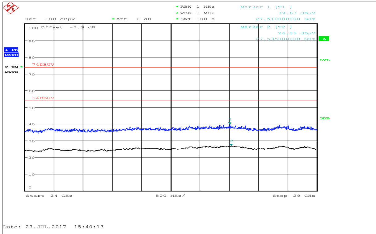
Plot 8: 24 GHz – 29 GHz, special test mode, f_{low}/f_{mid}/f_{high}
