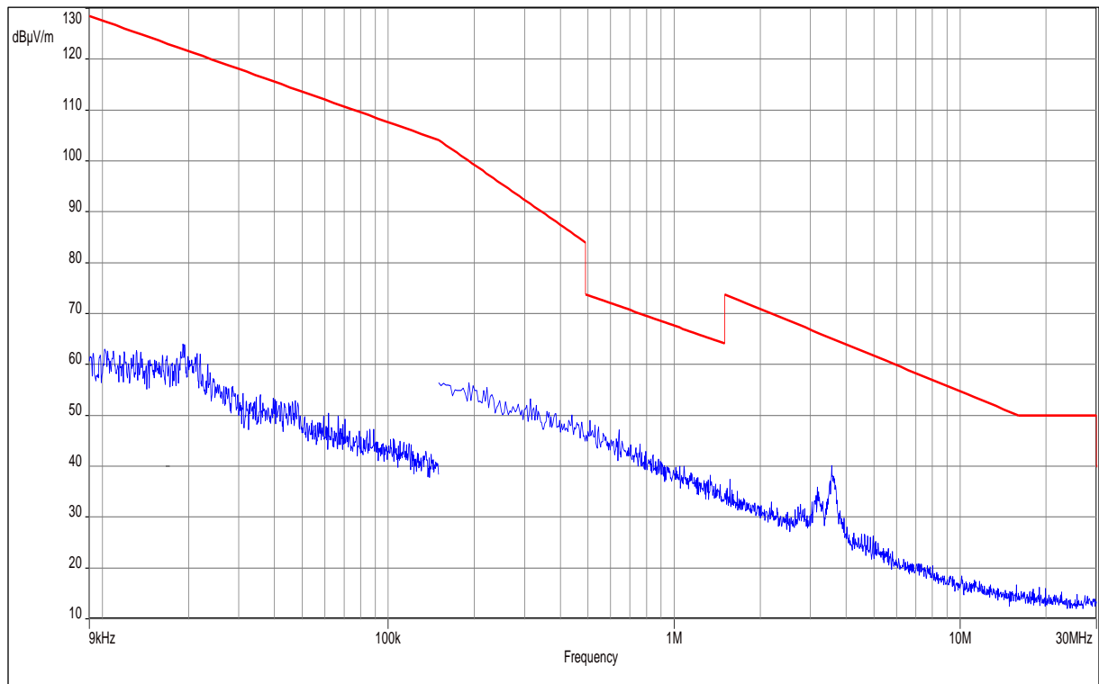
Plot 1: 9 kHz – 30 MHz, special test mode, frequency sweep stopped at f_{low}/f_{mid}/f_{high}
