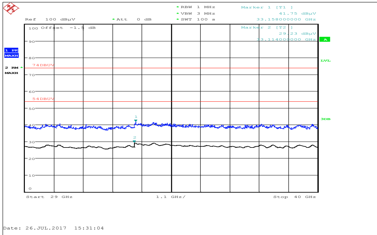
Plot 9: 29 GHz – 40 GHz, special test mode, f_{low}/f_{mid}/f_{high}
