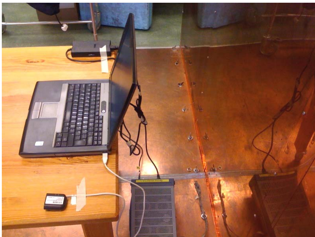
Conducted emission
