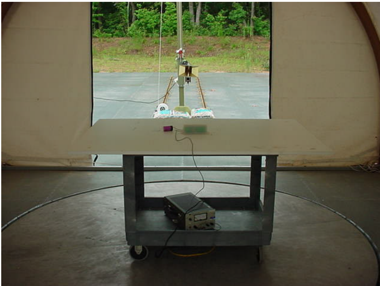
Figure 2: Radiated Emissions – Rear View
