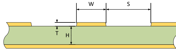
Figure 1. RF Track Dimensions
