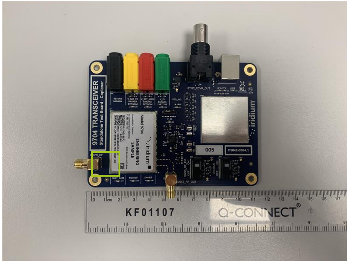
Figure 8 - View of test board used during compliance testing (coplanar waveguide antenna trace shown in green box)
