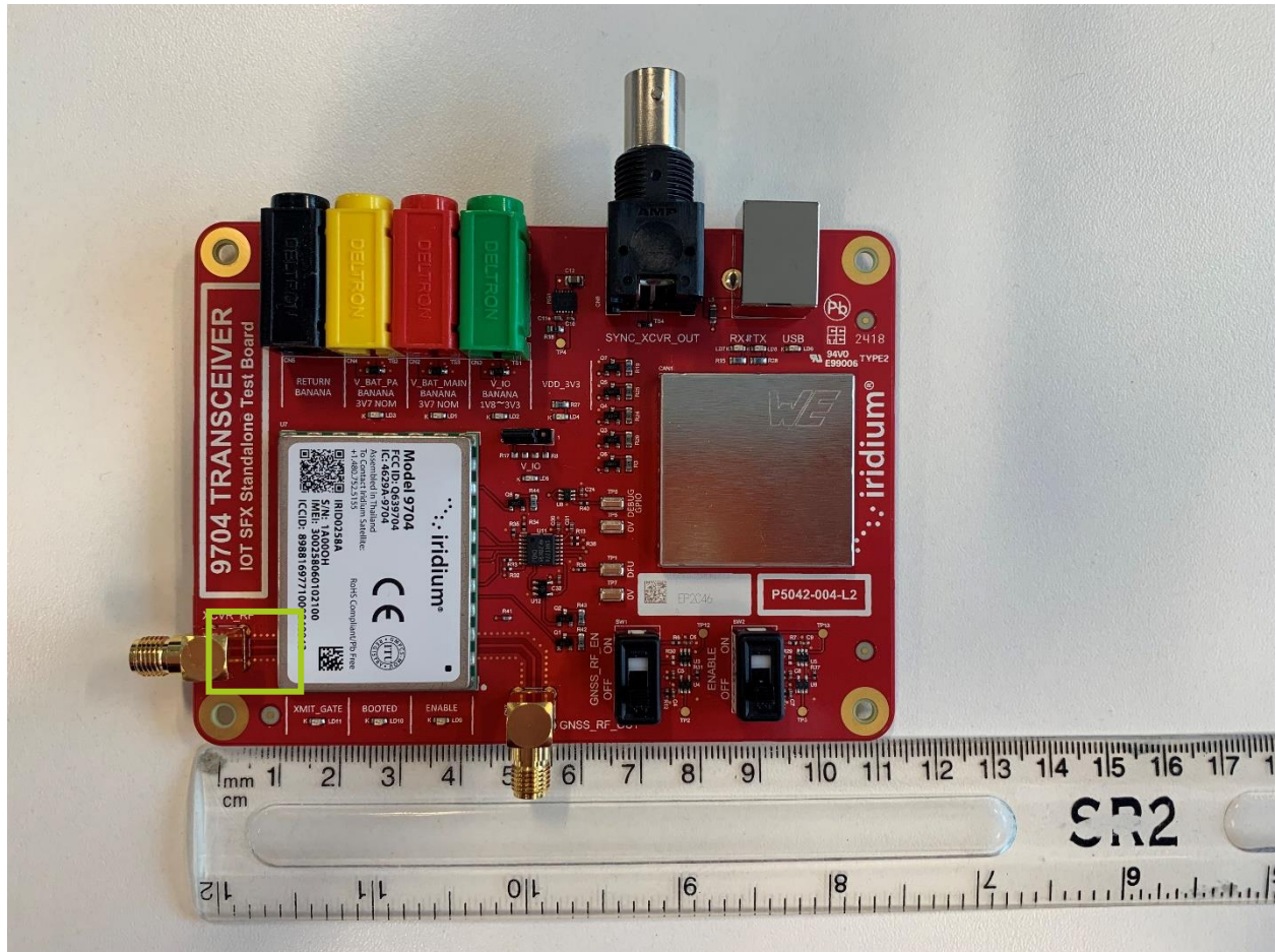
Figure 7 - View of test board used during compliance testing (microstrip antenna trace shown in green box)
