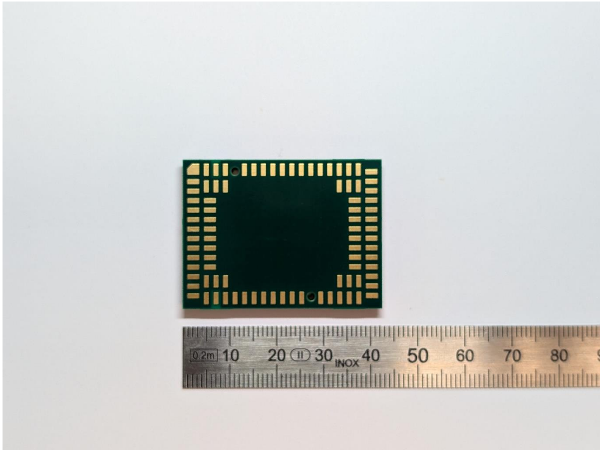
Figure 3 - 9704 transceiver bottom view
