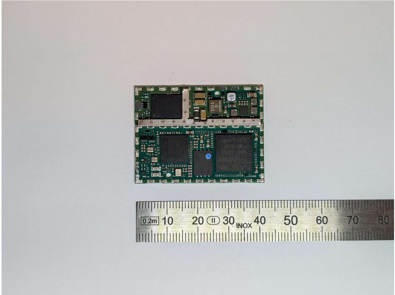
Figure 1 - 9704 transceiver internal top view
