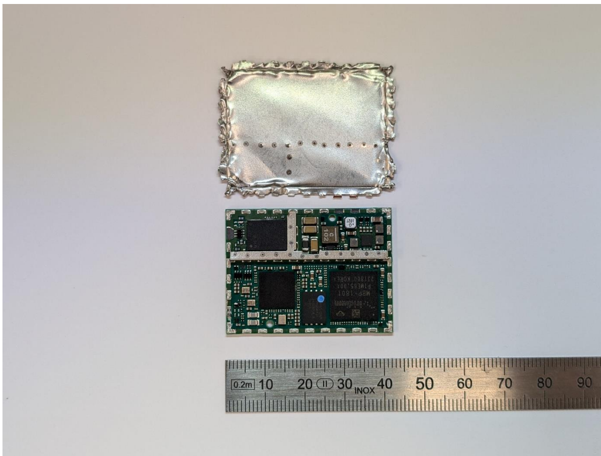
Figure 2 - 9704 transceiver internal top view including screening can lid
