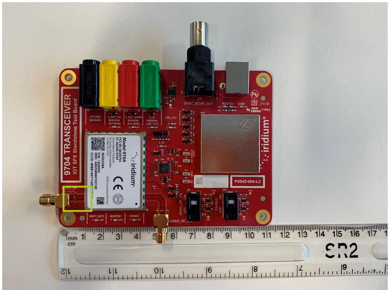
Figure 7 - View of test board used during compliant testing (antenna trace shown in green box)
