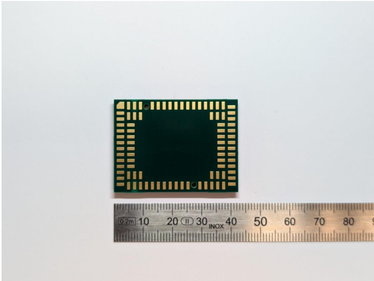
Figure 2 - 9704 transceiver external bottom view
