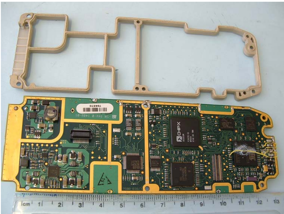
Rear of RF PCB Gasket Removed
