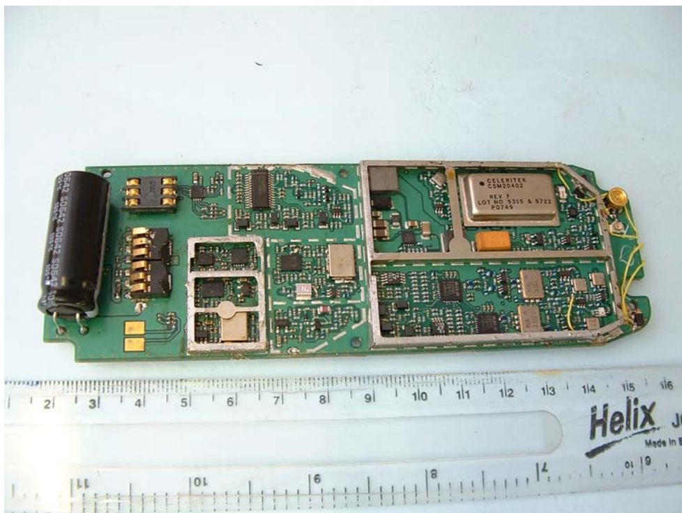
RF Side of PCB Cans Removed
