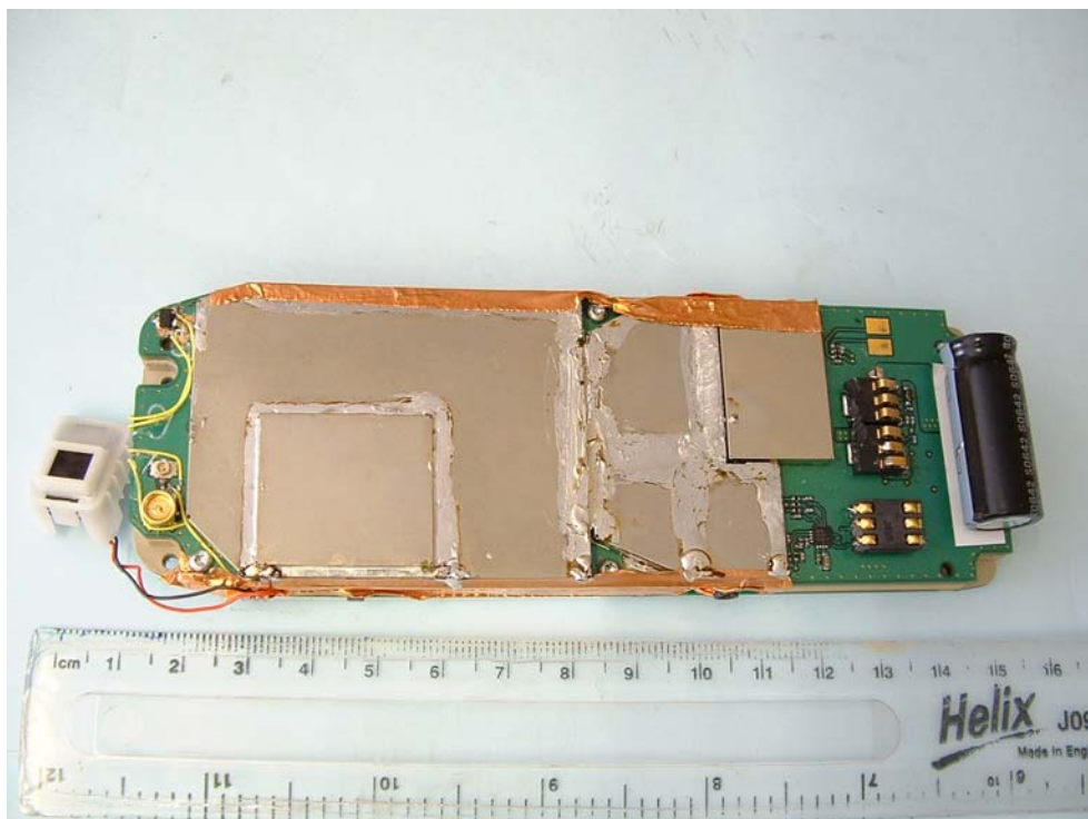
Assembled PCBs Rear
