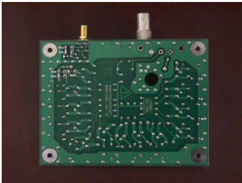
MARX Generator Assembly
