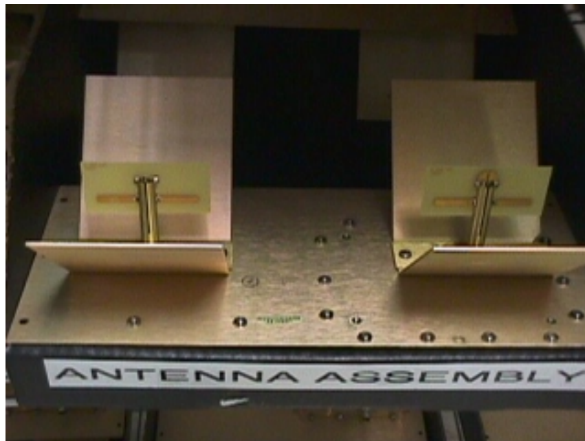
Antenna Assembly
