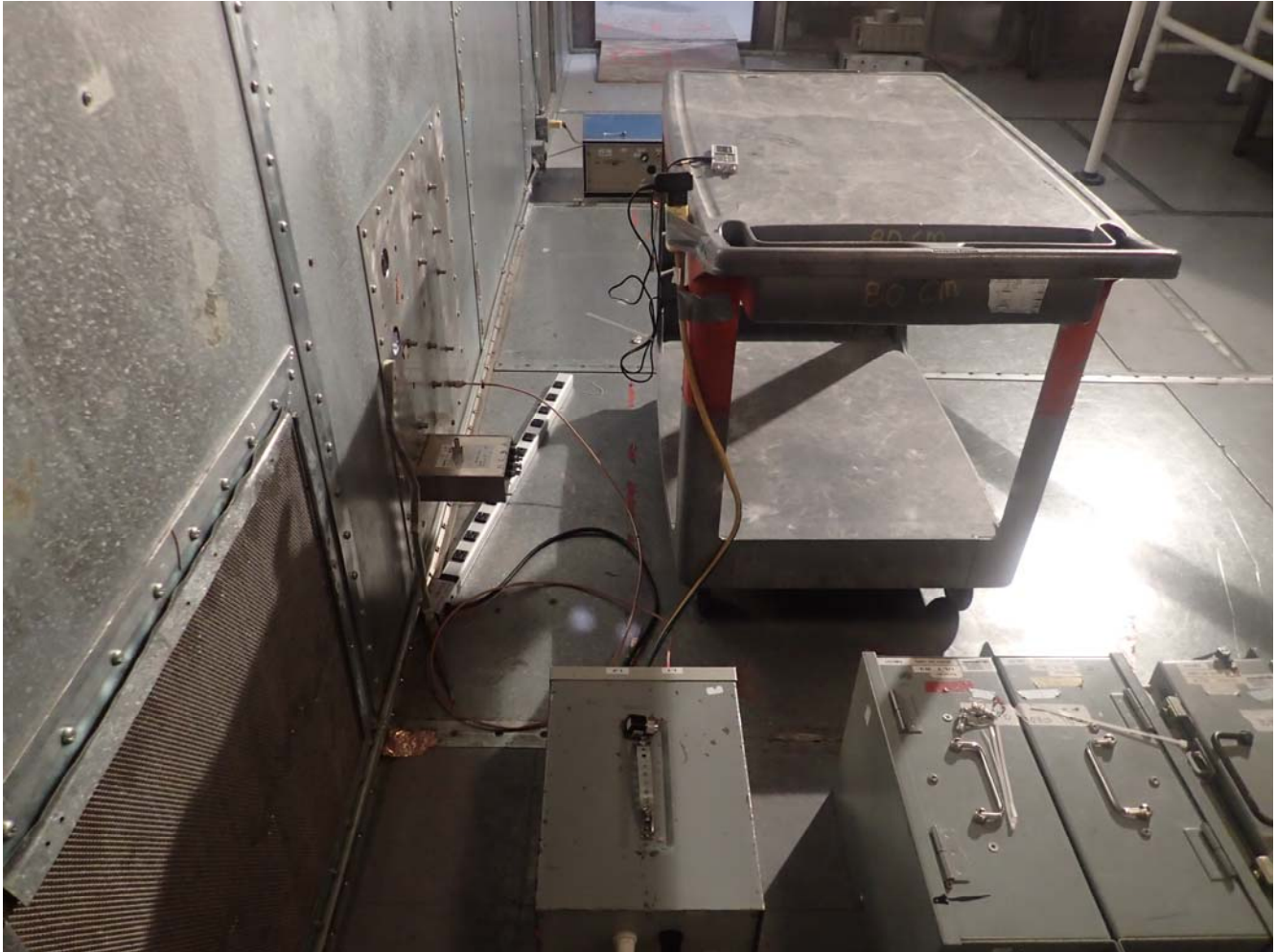
Power Line Conducted Emissions Test Configuration 1: 5 VDC Via AC Adapter
