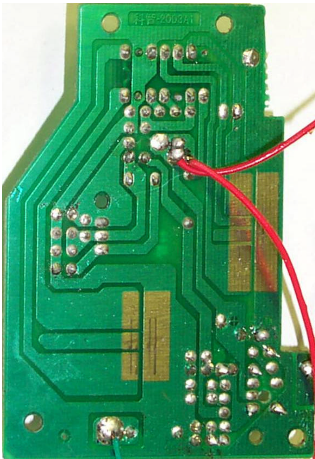
Foil Side
