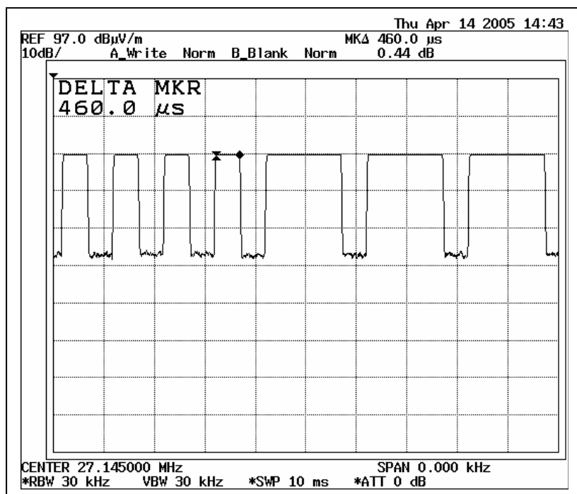
Duty Cycle 3
