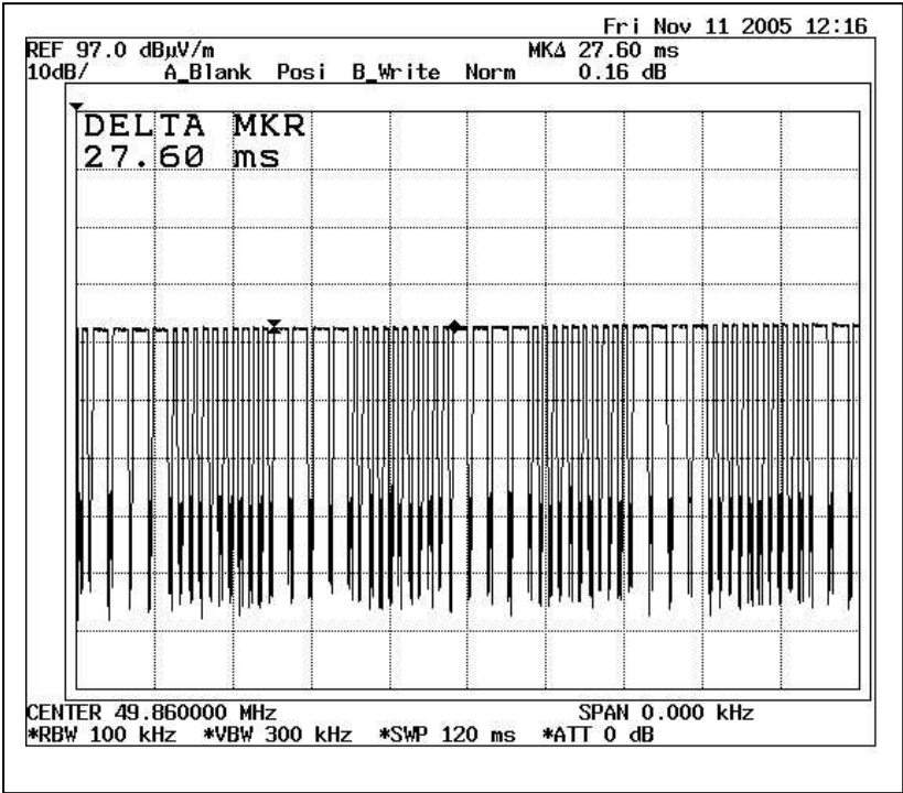
Duty Cycle
