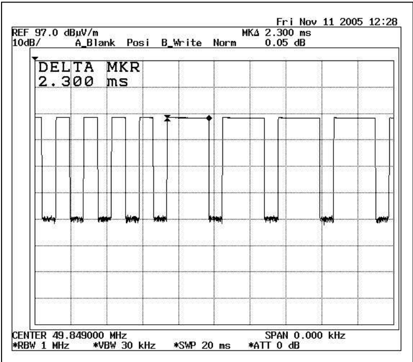
Duty Cycle 2
