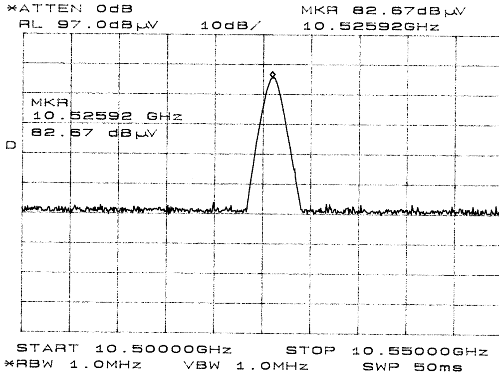
Figure Three, occupied bandwidth and bandedge compliance.
