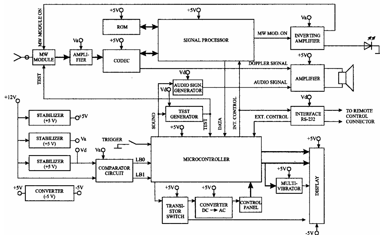
Block Diagram for Stealth Tracker, Model ST-M-S
